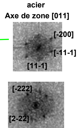
structure spinelle
