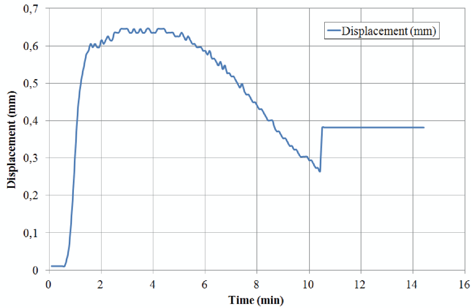
Figure 6.27: Evolution of the trial test displacement with time when the set up is composed of the tooling corresponding to the sample A \phi = 8 \text{ mm} and h_f = 13.6 \text{ mm}
