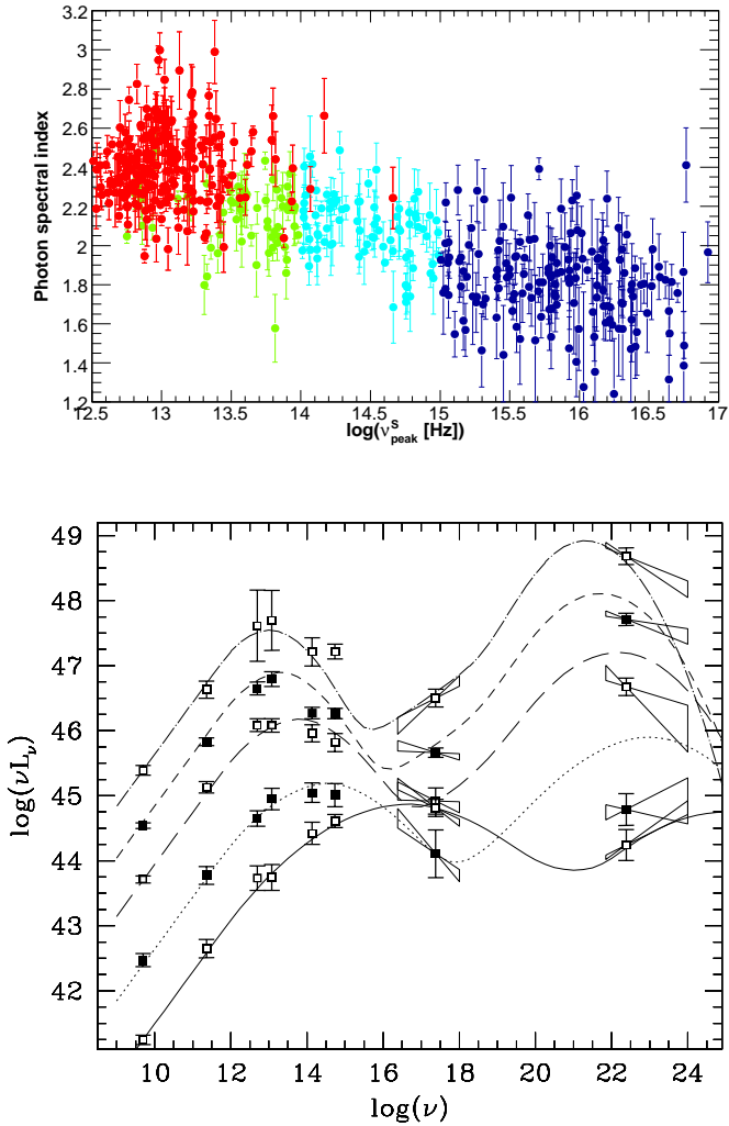
FIGURE 6. Top: Photon index vs frequency of the peak of the synchrotron component for the blazars detected with Fermi -LAT (cf. Fig. 5 for the color code). Extracted from Ackermann et al. (2011). Bottom: Spectral energy distributions of different types of blazars. From top left to bottom right: FSRQs, LBLs, IBLs and HBLs. Extracted from Fossati et al. (1998).
