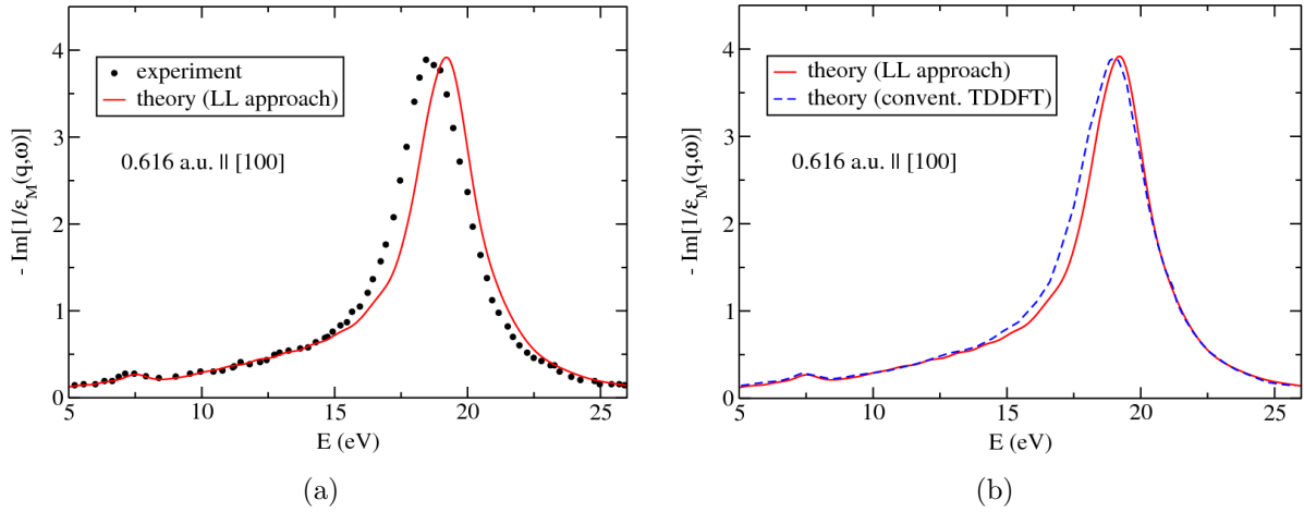
Figure 7.9: Comparison between the EEL spectrum of Al for \mathbf{q} = 0.616 \text{ a.u.} \parallel [100] calculated with the Liouville-Lanczos (LL) approach, using a 10 \times 10 \times 10 MP \mathbf{k} point mesh, a Lorentzian broadening \sigma = 0.051 \text{ Ry} , 400 Lanczos iterations, and the extrapolation scheme, with (a) the experimental spectrum [320], and (b) the theoretical EEL spectrum obtained within the conventional TDDFT approach [320] (see Sec. 3.3.3).
