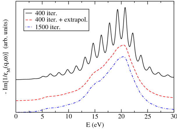
Figure 7.3: Effect of the extrapolation technique on the convergence of the EEL spectrum of bulk Si for \mathbf{q} = 0.53 \text{ a.u.} \parallel [100] . Curves have been shifted vertically for clarity.
