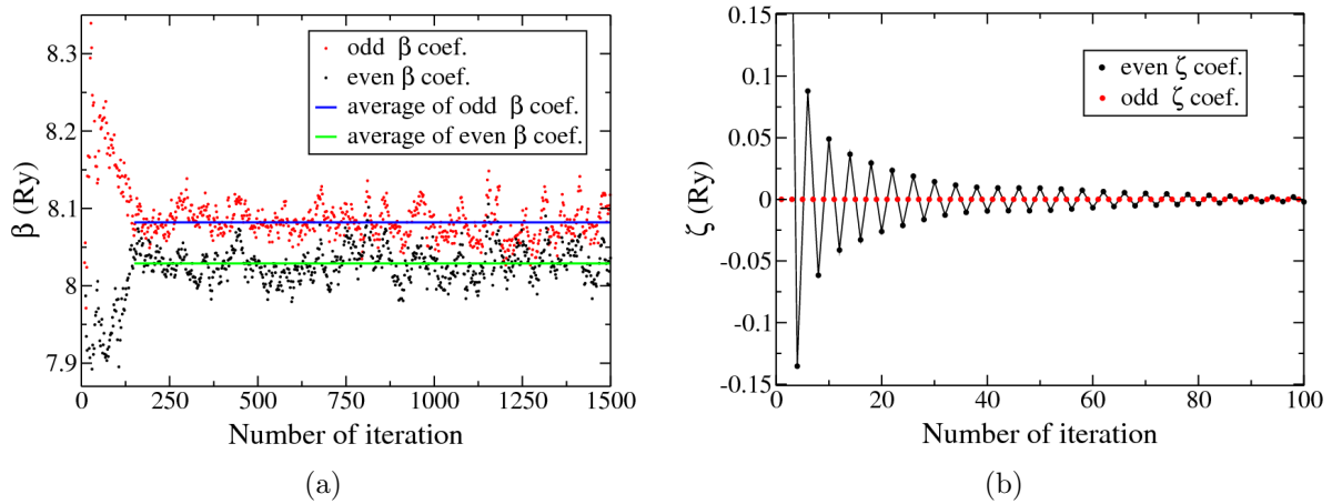
Figure 7.2: Coefficients of the Lanczos recursion method for bulk Si, \mathbf{q} = 0.53 \text{ a.u.} \parallel [100] . (a) Numerical behaviour of odd and even \beta coefficients as functions of the Lanczos iteration number. The horizontal lines are the averages of odd and even \beta coefficients. (b) Numerical behaviour of odd and even \zeta coefficients as functions of the Lanczos iteration number. Solid lines are guides for the eye.
