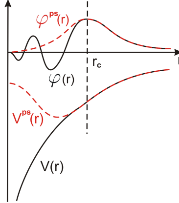
Figure 2.1: Schematic illustration of the replacement of the true potential V(r) and true electronic wavefunction \varphi(r) by a fictitious pseudopotential V^{ps}(r) and pseudo-wavefunction \varphi^{ps}(r) , respectively. For r > r_c , the PPs and wavefunctions become identical. This is the basic idea of the PP approximation. According to Ref. [75].
