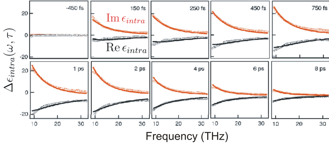
Figure 6.6: Pump-induced change of the intraband dielectric function \Delta\epsilon_{intra}(\omega, \tau) at several pump-probe delays (circles). In each panel, the upper (lower) curve is the imaginary (real) part of the variation of the intraband dielectric function. Fits obtained with the Drude model (solid lines) are superimposed onto the experimental data. From Ref. [245].
