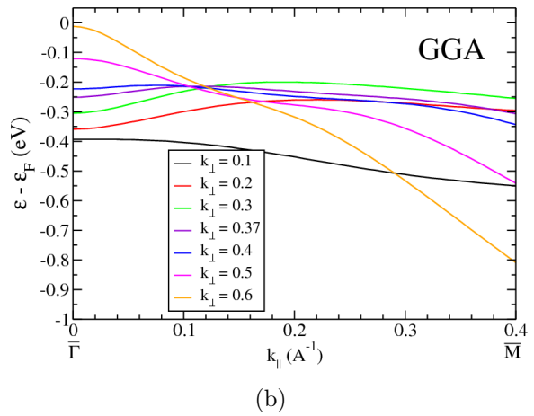
Figure 5.7: Kohn-Sham band structure of bulk Bi calculated along the direction in the bulk Brillouin zone which is parallel to the \bar{\Gamma} - \bar{M} direction of the surface Brillouin zone, at various values of k_{\perp} . The unit of k_{\perp} is \text{\AA}^{-1} . (a) Calculation within the LDA at the LDA-ELP, (b) Calculation within the GGA at the GGA-ELP. (Unpublished)
