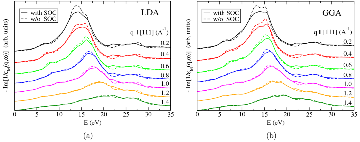
Figure 7.17: EEL spectra of bulk Bi at various values of the transferred momentum \mathbf{q} along the [111] direction, in units of \text{\AA}^{-1} . (a) Calculations within the LDA with and without spin-orbit coupling (SOC), (b) Calculations within the GGA with and without SOC. Curves have been shifted vertically for clarity. Calculations have been performed by using a 12 \times 12 \times 12 uniform \mathbf{k} point mesh centered at the \Gamma point, and a Lorentzian broadening \sigma = 0.035 Ry.
