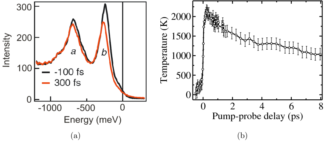
Figure B.2: (a) Photoelectron spectra acquired 100 fs before and 300 fs after the arrival of the pump beam along the \bar{\Gamma}-\bar{M} direction at k_{\parallel} = 0.12 \text{ \AA}^{-1} . (b) The effective temperature T_+ of the photoexcited electrons as a function of the pump-probe delay. From Ref. [267].
