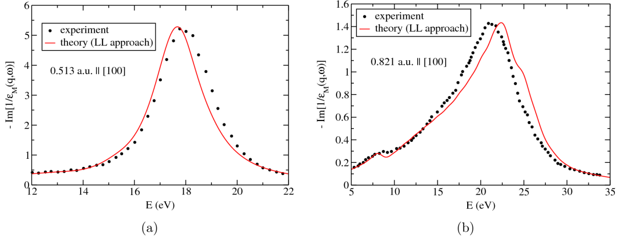
Figure 7.10: (a) Comparison of the EEL spectra of Al for \mathbf{q} = 0.513 a.u. || [100] between experiment [320] and theory, using a 10 \times 10 \times 10 MP \mathbf{k} point mesh, a Lorentzian broadening \sigma = 0.056 Ry, 300 Lanczos iterations, and the extrapolation technique. (b) Comparison of the EEL spectra of Al for \mathbf{q} = 0.821 a.u. || [100] between experiment [320] and theory, using a 14 \times 14 \times 14 MP \mathbf{k} point mesh, a Lorentzian broadening \sigma = 0.068 Ry, 450 Lanczos iterations, and the extrapolation technique.
