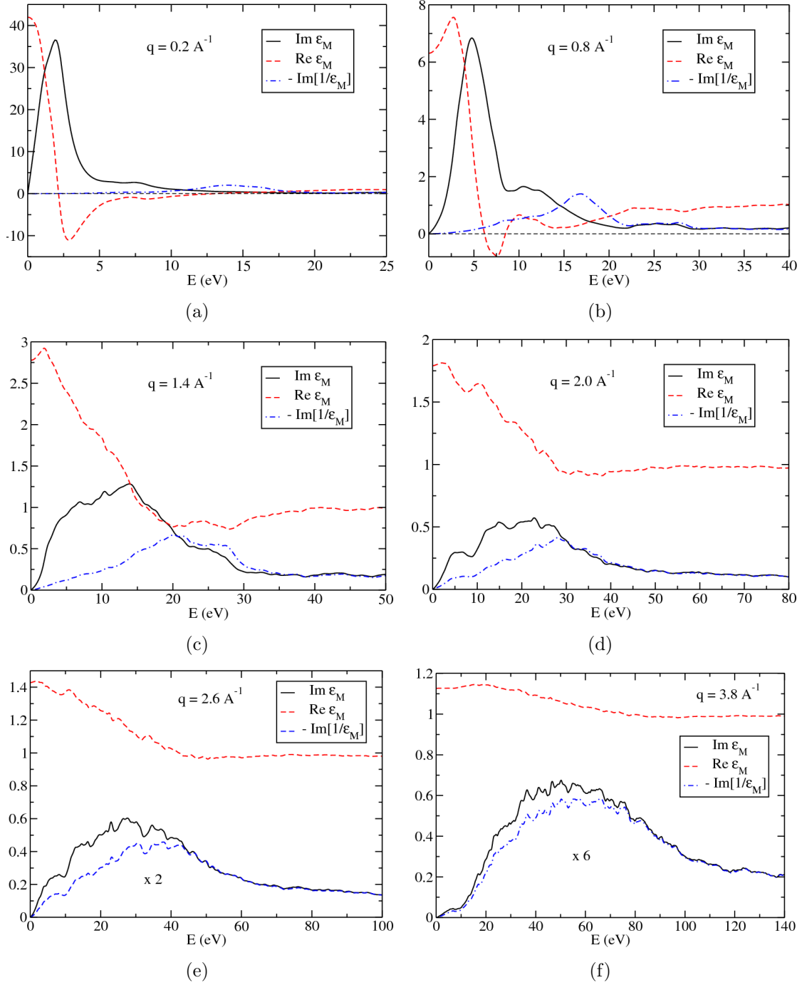
Figure 7.19: (a)-(f) Comparison of \text{Re}[\epsilon_M] , \text{Im}[\epsilon_M] , and -\text{Im}[1/\epsilon_M(\mathbf{q})] at various values of \mathbf{q} along the [111] direction. Calculations have been performed within the LDA without the spin-orbit coupling, by using a 12 \times 12 \times 12 uniform \mathbf{k} point mesh centered at the \Gamma point, and a Lorentzian broadening \sigma = 0.035 Ry. In panels (e) and (f), \text{Im}[\epsilon_M] and -\text{Im}[1/\epsilon_M(\mathbf{q})] have been multiplied by a factor for better visibility.
