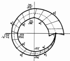
Figure 3. — A_{1,2}(1, 0) .
