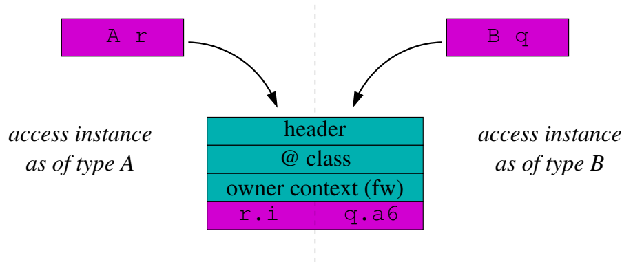
Figure 4.6: Field access in the confused object instance.
