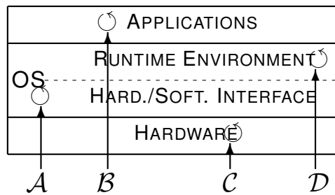
Figure 6.2: Different requests handling
