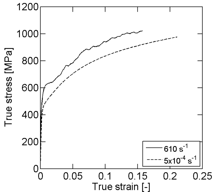
Figure 3-13: True stress-strain curves at pre-necking plastic strain rates of 5 \times 10^{-4}/s (dashed line) and 610/s (solid line).
