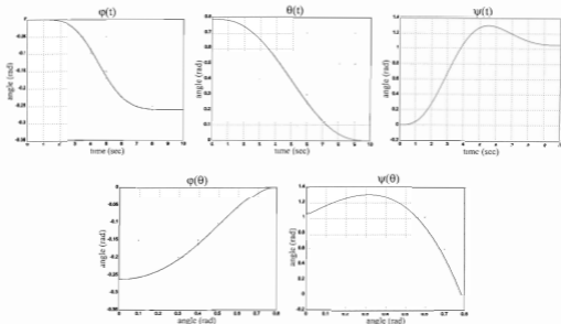
Figure 2.15: The solution of the MPP for the orientation angles.
