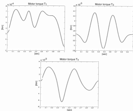
Figure 3.14: Motor torques generating the horizontal displacement; see Figure 3.12 for the notations T_1 , T_3 and T_4
