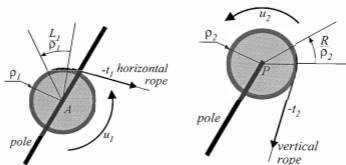
Figure 3.4: Torques at the winches
