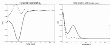
Figure 3.22: Closed-loop tracking behavior under PD control. Trajectory of the rope lengths: i ) stabilizing equilibrium controller (hashed line); ii ) tracking controller with motion planning; iii ) reference to steer to equilibrium along a straight line (dotted).
