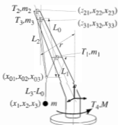
Figure 3.12: 3D US Navy crane
