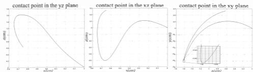
Figure 2.17: Trajectory of the contact points on the tangent planes
