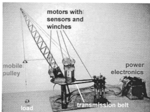
Figure 3.1. Reduced size model of the US Navy crane
