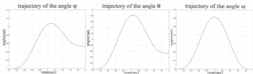
Figure 2.16: Trajectory of the orientation of the sphere ( RPY angles: \varphi , \theta , \psi )
