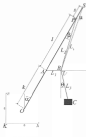
Figure 3.2: Planar version of the crane
