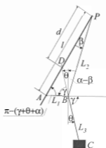
Figure 3.5: Geometry of the planar crane
