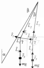
Figure 3.19: The two equilibria coincide: reasoning by contradiction
