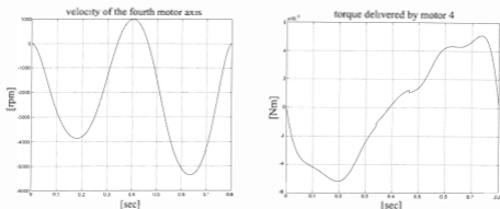
Figure 3.18: The rpm (revolutions per minute) and the torque delivered by the fourth motor (rotating the platform with the boom), corresponding to the trajectory illustrated in Figure 3.17 (travelling duration equals to 0.8 sec)
