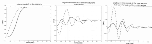
Figure 3.23: Closed-loop tracking behavior under PD control. Trajectory of the angles: i ) stabilizing equilibrium controller (hashed line); ii ) tracking controller with motion planning; iii ) reference to steer to equilibrium along a straight line (dotted).
