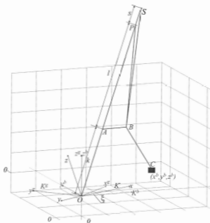
Figure 3.7: Crane in three dimensions
