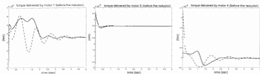
Figure 3.24: Closed-loop tracking behavior, motor torques: i ) stabilizing equilibrium controller (hashed line); ii ) tracking controller with motion planning; iii ) reference to steer to equilibrium along a straight line (dotted).
