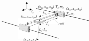
Figure 3.11: 3D Overhead crane
