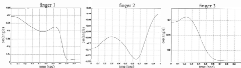
Figure 2.19: Cosine of angles between the contact forces and the surface normals.
