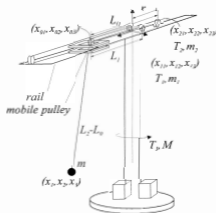
Figure 3.10: 3D Cantilever crane
