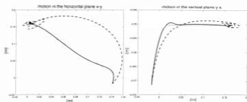
Figure 3.21: Closed-loop tracking behavior under PD control. Trajectories of the load in the horizontal and vertical planes: i ) stabilizing equilibrium controller (hashed line); ii ) tracking controller with motion planning; iii ) reference to steer to equilibrium along a straight line (dotted).
