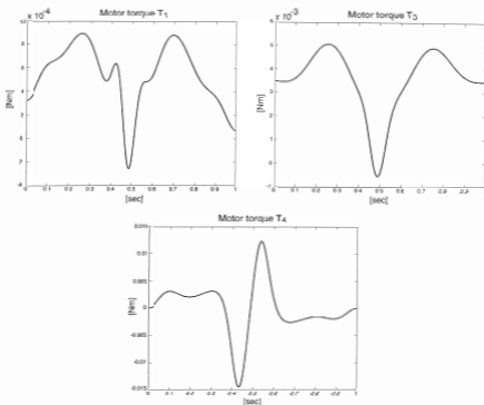
Figure 3.16: Motor torques generating the parabolic trajectory; see Figure 3.12 for the notations T_1 , T_3 and T_4
