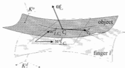
Figure 2.3: Rolling without slipping of surfaces
