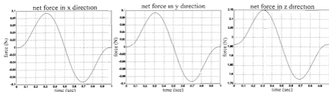
Figure 2.18: Components of the net force applied on the object by the fingers.
