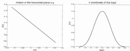
Figure 3.15: Parabolic displacement of the load
