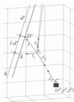
Figure 3.8: Rope tensions
