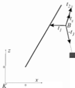
Figure 3.3: Rope tensions (at the free pulley)
