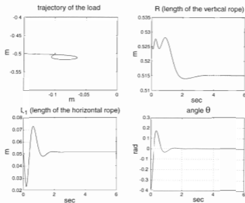
Figure 3.20: Closed-loop behaviour under PD control
