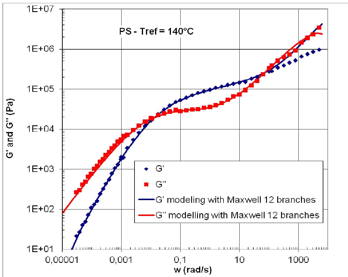
Figure 3.32. Viscoelastic behavior modeling of the studied PS at 140°C.
