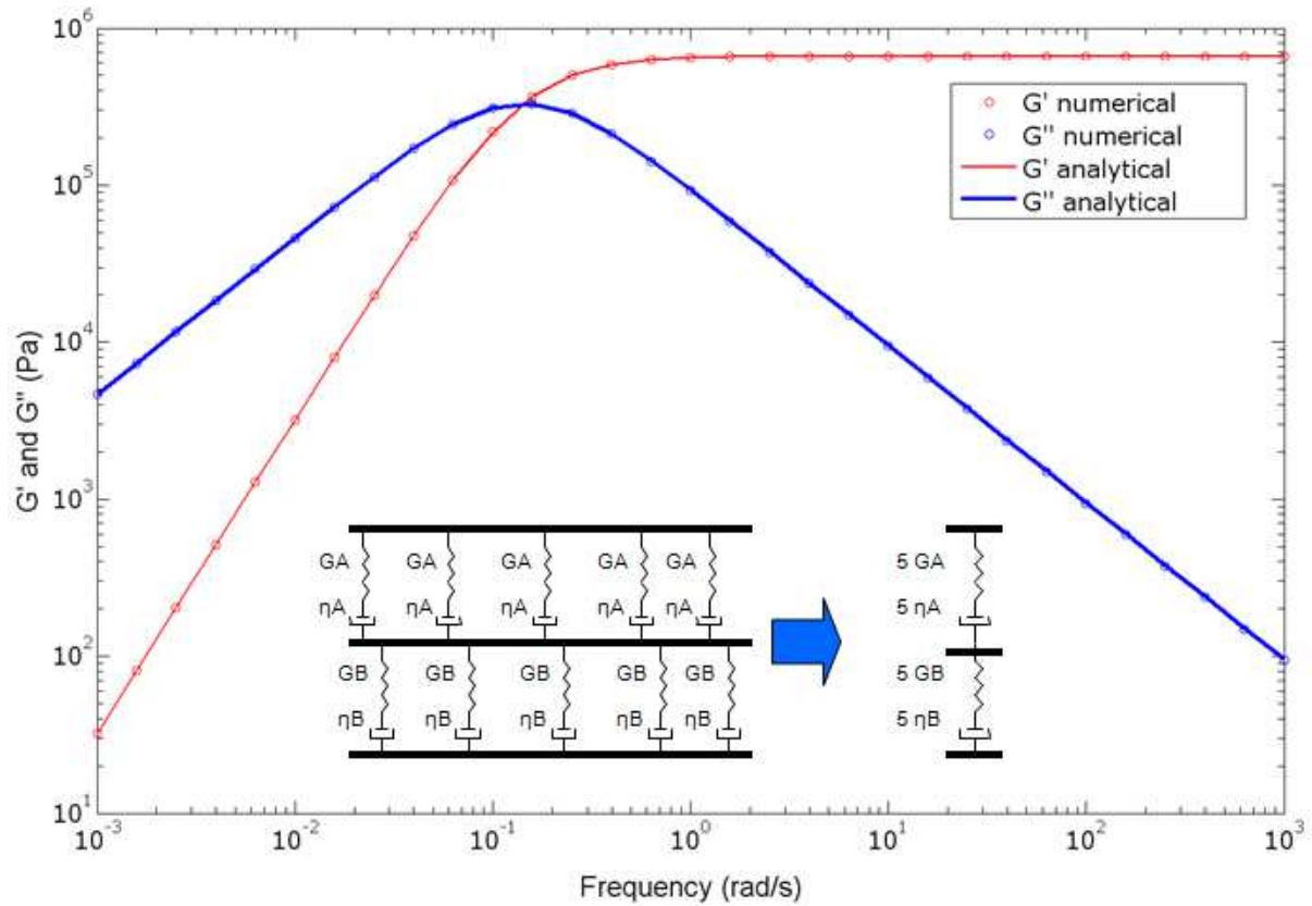
Figure 3.41. Analytical versus numerical solution for a multilayer, each layer modeled by a generalized Maxwell model:
