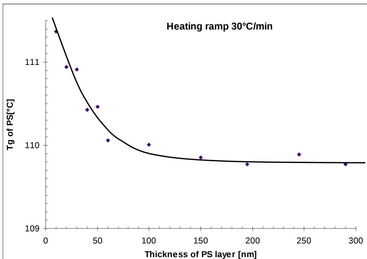
Figure 3.7. Dependence : T_g versus layers thicknesses: a continuous increase of T_g with decreasing PS layer thickness resulting in a difference of about 2°C between PS 10 nm and PS 290 nm.
