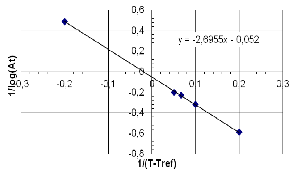
Figure 3.28. C1 and C2 identification of WLF law for PC at T ref = 140°C.
