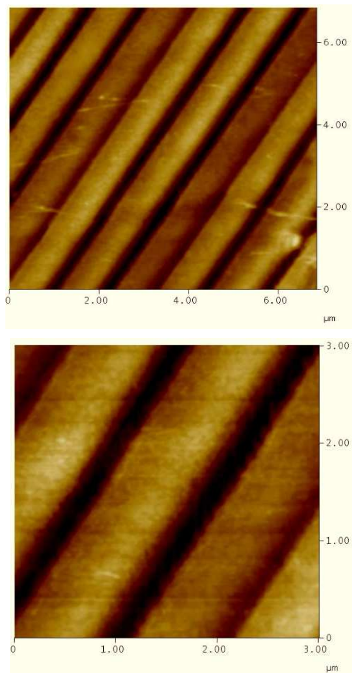
Figure 3.1. AFM images for the film PC/PS, 70/30, 125 \mu\text{m} thick ( scale: 6 \mu\text{m} - top image and 3 \mu\text{m} – lower image). The light bands belong to polycarbonate and the dark ones correspond to polystyrene layers.
