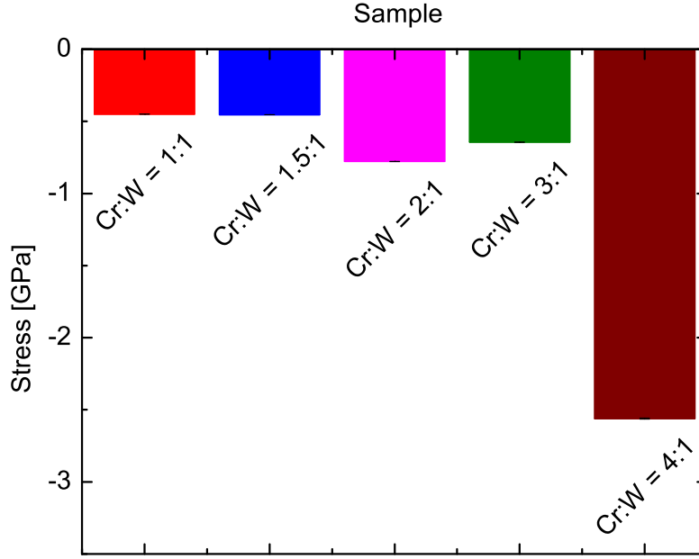
Figure 3.32: Compressive stress of CrN-WC samples deposited on Si, at low fixed Ar/N 2 ratio and low deposition temperature.
