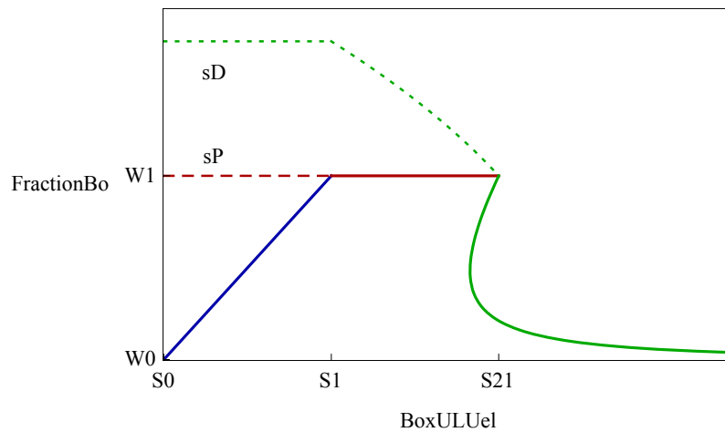
Figure 4.25: The stress-displacement response for the E - P - DP response: the elastic phase (blue); the damaging phase (solid green); the coupled plasticity-damaging phase (solid red); the damage yield stress (dashed green) and plastic yield stress (dashed red) at the center of the localization zone
