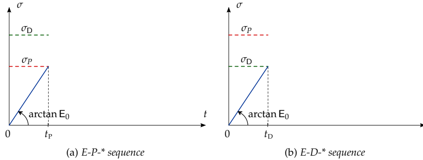
Figure 3.6: Elastic response
