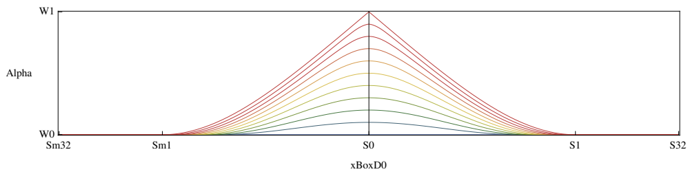
Figure 4.17: The damage profiles evolution in a one-dimensional bar
