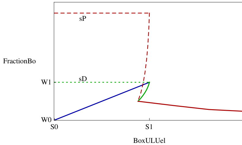
Figure 4.13: The stress-displacement diagram for the E-D-PD response: the elastic phase (blue); the damaging phase (solid green); the coupled plasticity-damaging phase (solid red); the damage yield stress (dashed green) and plastic yield stress (dashed red) at the center of the localization zone
