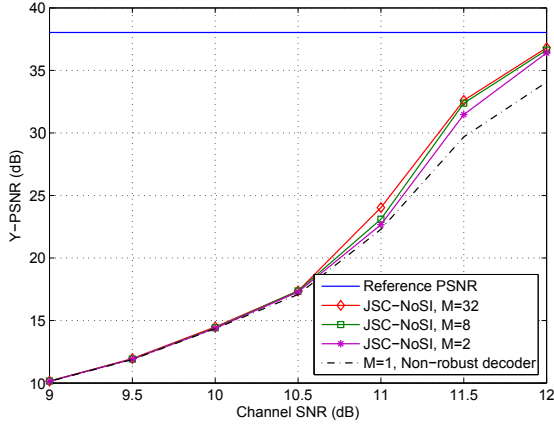
(a) foreman.qcif , block size 22 \times 18
