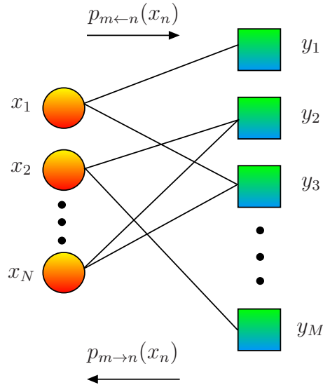
Figure 5.5.: Factor graph for the linear mixing estimation problem.
