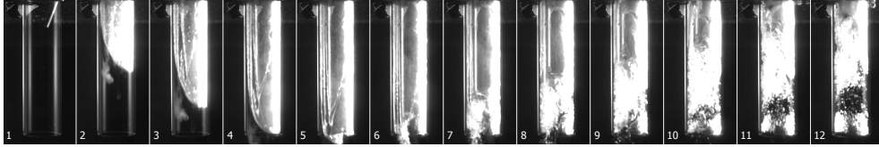
FIGURE 13. Chronophotography of a confined cavity in a tube of 5 cm diameter and 17.3 cm length. The initial velocity of expansion of the cavity is 3.3 m/s. The expansion stops at the end of the tube. The time step between images is 15 ms.
