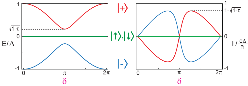
Figure 1.2: Energies (left) and supercurrents (right) of the four different configurations of the ABS versus the phase difference for a superconducting short single channel of transmission \tau = 0.95 . Whereas the even states |-\rangle and |+\rangle carry opposite supercurrent, the odd ones |\uparrow\rangle and |\downarrow\rangle do not carry any.
