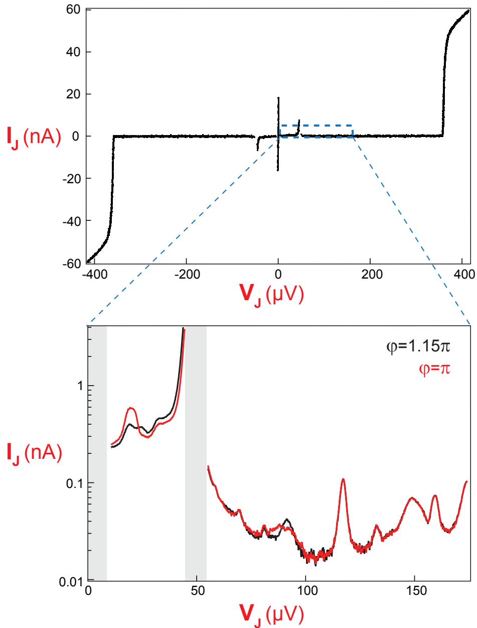
Figure 6.4: Current-voltage I_J(V_J) characteristic of the JJS, for contact V {0.985, 0.37, ..}, at different magnifications. Top: at large scale and at flux \phi = 0 . In the subgap region, a large peak is visible near 45 \mu V. Bottom: at higher magnification (log current scale) and for two different flux values \phi = 1.15\pi (black line) and \phi = \pi (red line). The gray regions are unstable and thus not accessible to measurement. In addition to the large peak, several smaller peaks are observed.
