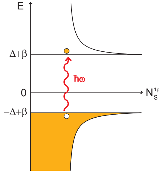
Figure 2.5: Sketch of the photon-absorption spectroscopy, in the one-particle picture.
