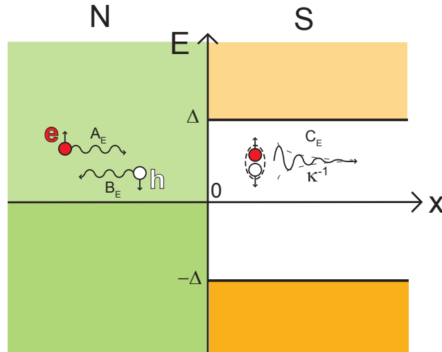
Figure 2.6: Sketch of the Andreev reflection. The discontinuity in the superconducting order parameter behaves as a barrier potential. In addition to the usual specular reflection (not represented), the pairing interaction in the superconductor induces a new type of reflection, the Andreev reflection, in which a spin-up electron (red) is reflected into a spin-down hole (white). When the energy of the incident propagating states in the normal region is smaller than \Delta , they become evanescent in the superconducting region on a length scale \kappa^{-1} . Note that all waves should be at the same energy but are shifted for readability.
