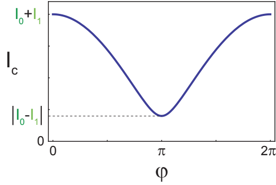
Figure F.2: Critical current of a SQUID made of two different \mathbb{J}\mathbb{J} as a function of the phase, for a critical current asymmetry \alpha = 0.2 . Note that the minimum of the critical current is always found at \varphi = \pi , independently on the critical current asymmetry \alpha .
