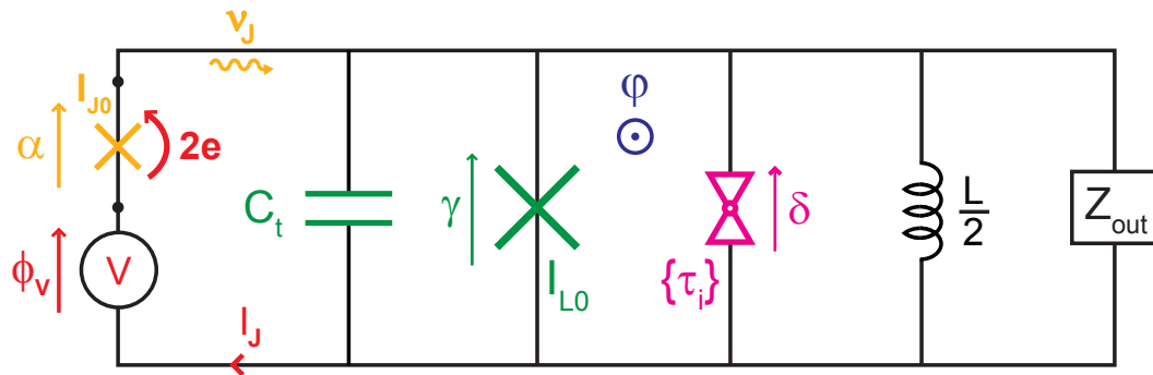
Figure 7.1: Electrical circuit as seen from the Josephson junction spectrometer.
