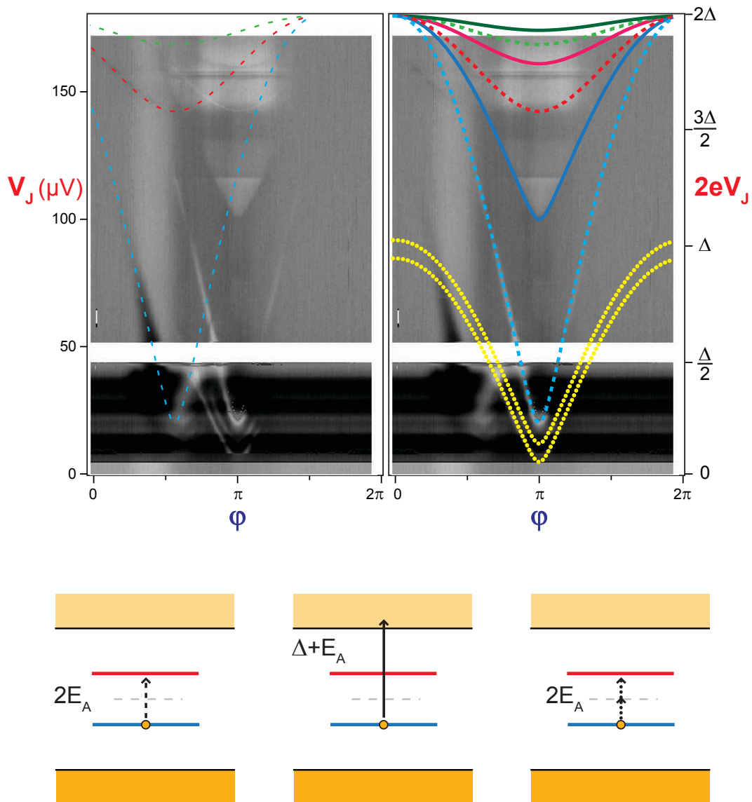
Figure 8.3: Switching spectrum P_{sw}(\phi, V_J) for contact V (same scale as Fig. 8.2). Right: The dashed lines are the Andreev resonances 2eV_J = 2E_A(\phi, \tau_i) . The solid lines correspond to the energy thresholds of transitions from the lower ABS to the continuum 2eV_J = \Delta + E_A(\phi, \tau_i) . The dotted lines correspond to higher order transitions of energies 2eV_J = E_A(\phi, \tau_i) + 3\mu\text{eV} and 2eV_J = E_A(\phi, \tau_i) - 11\mu\text{eV} . Left: The thin dashed lines are the Andreev resonances 2eV_J = 2E_A(\phi + 0.3\pi, \tau_i) shifted in flux by \arcsin(s_0) \simeq 0.3\pi . These transitions occur during the measurement pulse. Bottom: Sketch of the different transitions.
