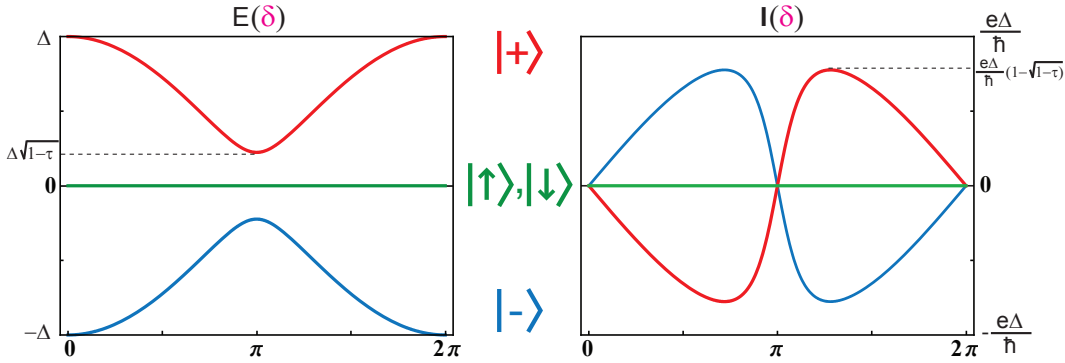
Figure 3.1: Energies (left) and supercurrents (right) of the four states corresponding to the possible occupations of the 2 ABS versus the phase difference for a JC of transmission \tau = 0.95 . Whereas the even states |-\rangle and |+\rangle carry opposite supercurrent, the odd ones |\uparrow\rangle and |\downarrow\rangle do not carry any.
