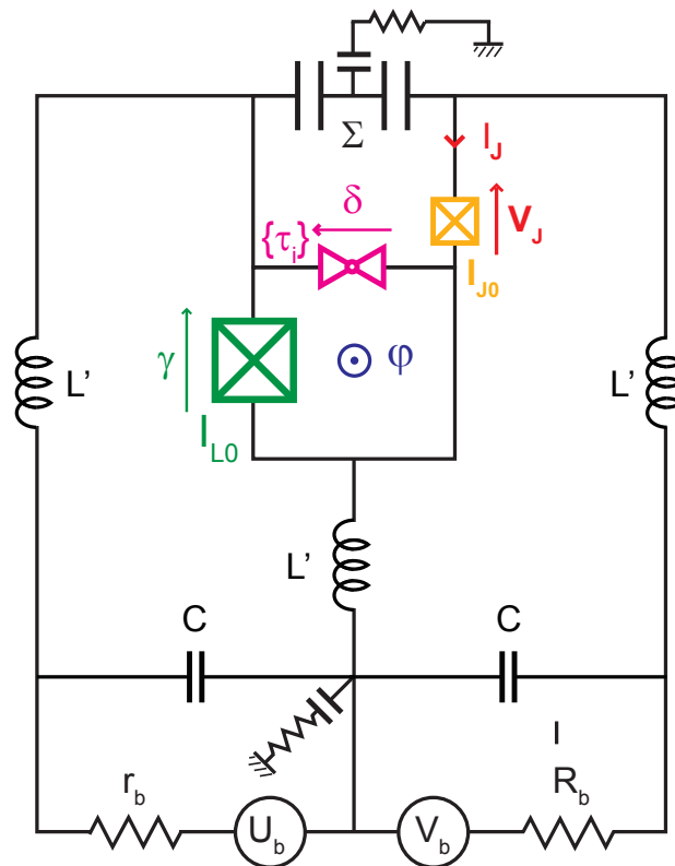
Figure G.1: Schematic of the sample JT6. The JJS [respectively the SQUID] is biased by a voltage source V_b [ U_b ] through an on-chip LC filter ( L' \simeq 450 pH, C \simeq 20 pF) and a series resistance R_b = 2 k \Omega [ r_b = 200 \Omega ] mounted at the same temperature as the sample. The current I_J (red) [ I_S (magenta)] is measured from the voltage drop across R_b [ r_b ]. These two parts, which are independent from the dc point of view, are coupled through an on-chip capacitor \Sigma \simeq 30 pF. The extra capacitors ( \sim 1 pF) and resistances represent the capacitive coupling to the resistive (chrysocal) ground plane.
