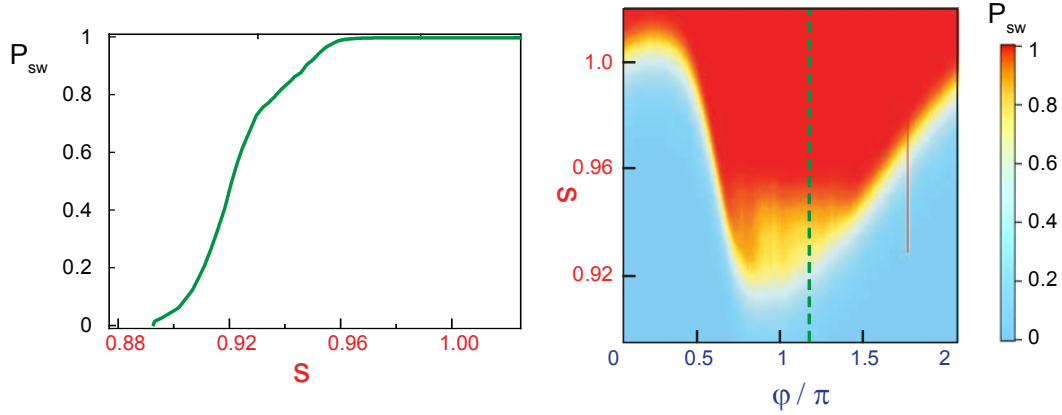
Figure 8.4: Right: Switching probability P_{sw}(\varphi, s) as a function of both the reduced bias current s and the flux \varphi , for contact V , while the JJS is biased at a voltage V_J = 150 \mu\text{V} . Left: Cut P_{sw}(s) at the position of the dashed line.
