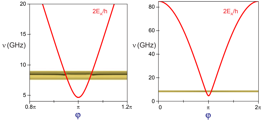
Figure L.8: Full theoretical (solid red line) Andreev spectrum 2E_A(\varphi, 0.19)/h , for \tau = 0.997 . The experimental spectrum for contact \{0.997, 0.19\} is superimposed at the same scale.
