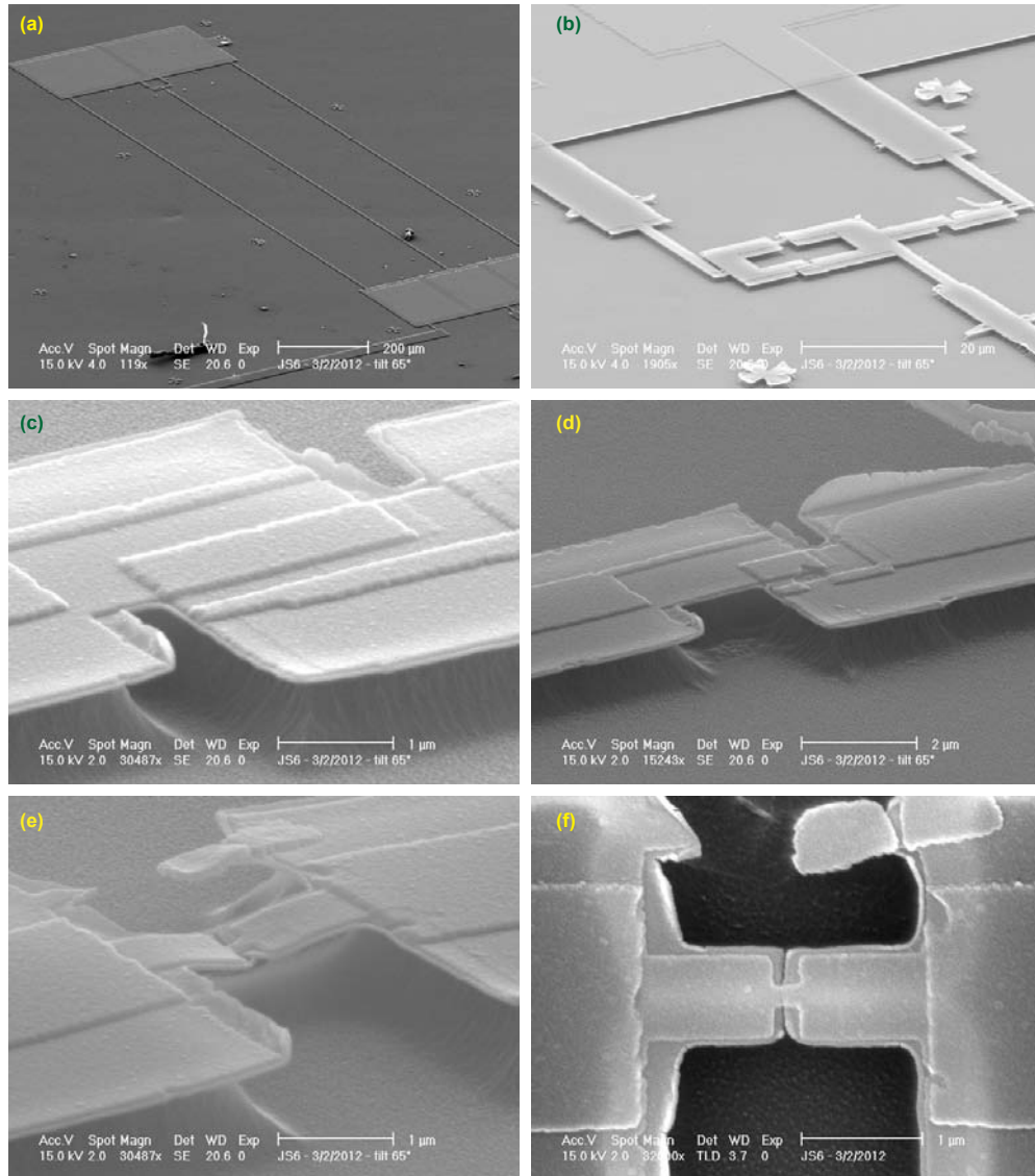
Figure 9.9: SEM micrograph of sample JS6 at different magnifications: (a) capacitors and inductive lines; (b) SQUID loop and JJs at large scale; (c) JJ of the SQUID; (d) JJs; (e,f) bridge for atomic contacts. The first five pictures are taken under both tilt and planetary angle.
