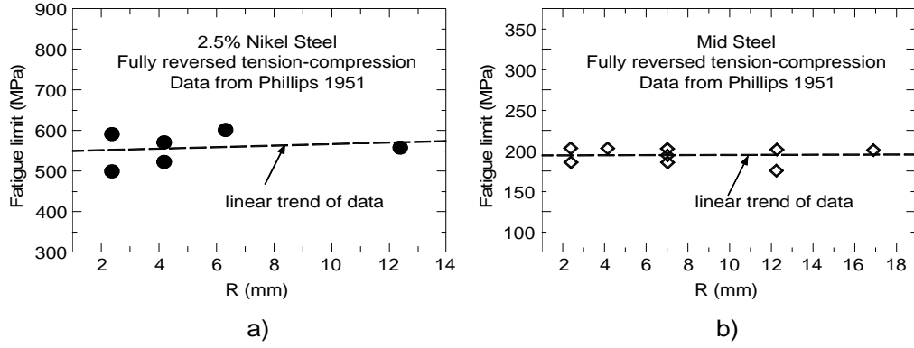
Figure 5.5 : Fully reversed tension-compression fatigue limit data (Results of Phillips and Heywood [138], represented by Papadopoulos and Panoskaltzis [135])
