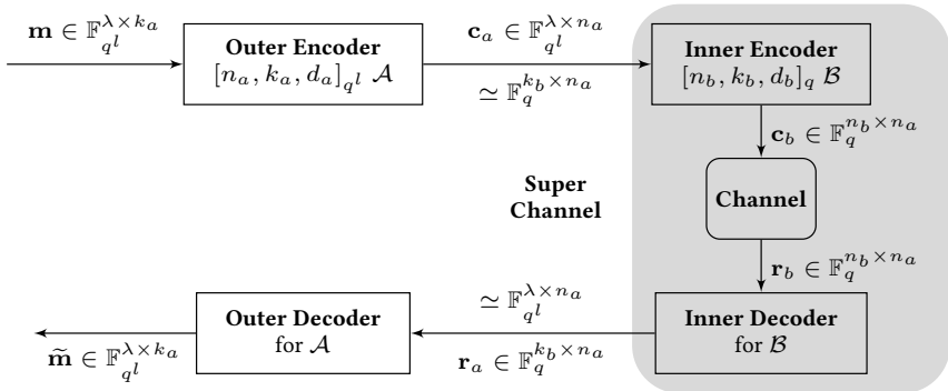
Figure 2.2: The super channel in a classic concatenated code scheme with an [n_a, k_a, d_a]_{q^l} outer code \mathcal{A} and an [n_b, k_b, d_b]_q inner code \mathcal{B} where k_b = \lambda \cdot l .
