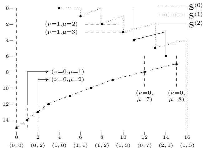
Figure 4.1: Illustration of the row pointers \kappa_0 , \kappa_1 and \kappa_2 of Algorithm 4.1 applied to a horizontal band of three Hankel matrices \mathbf{S}^{(0)} , \mathbf{S}^{(1)} and \mathbf{S}^{(2)} . The columns of the 16 \times 18 matrix (\mathbf{S}^{(0)} \mathbf{S}^{(1)} \mathbf{S}^{(2)}) are arranged under \prec_{4-1}^H -ordering. The three lines trace the row pointers \kappa_0 , \kappa_1 and \kappa_2 for each sub-matrix \mathbf{S}^{(0)} , \mathbf{S}^{(1)} and \mathbf{S}^{(2)} . The second axis of abscissae shows the column pointer (\nu, \mu) indicating the \mu -th column of the sub-matrix \mathbf{S}^{(\nu)} .
