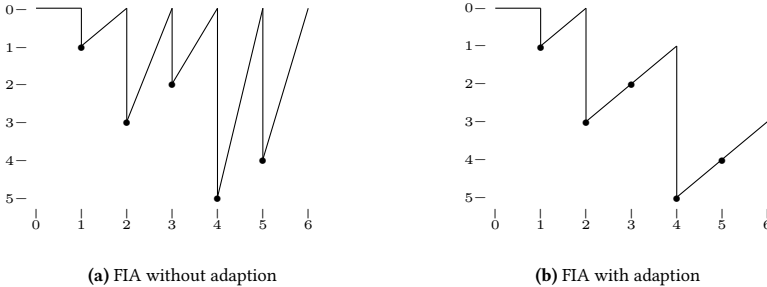
Figure 3.3: Illustration of the row pointer \kappa of the classic FIA (Subfigure 3.3a) and of the adjusted Algorithm 3.3 (Subfigure 3.3b), when both algorithms are applied to a 6 \times 7 Hankel syndrome matrix of a [16, 4]_{17} GRS code. The dots indicate the calculation of a non-zero discrepancy and where an update of the interim polynomial is not possible (core discrepancy, see Definition 3.10). Then, both algorithms enter a new column with different initialization of their row pointers.
