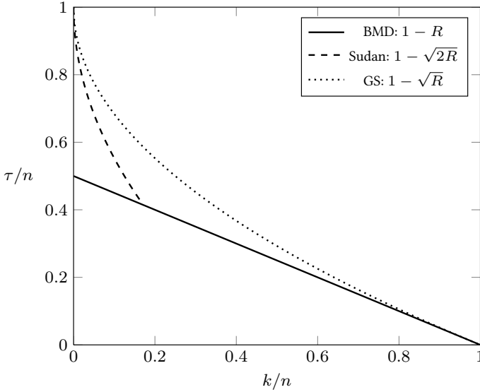
Figure 3.5: Illustration of the normalized decoding radius \tau/n for BMD, Sudan ( m = 1 ) and Guruswami–Sudan ( m \rightarrow \infty ) decoding as a function of the code-rate k/n for the asymptotic case ( n \rightarrow \infty ).
