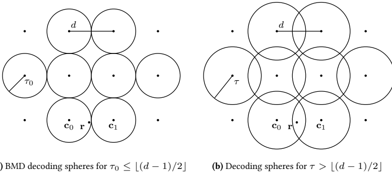
(a) BMD decoding spheres for \tau_0 \leq \lfloor (d-1)/2 \rfloor
