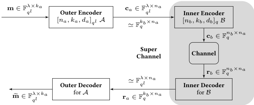
Figure 2.2: The super channel in a classic concatenated code scheme with an [n_a, k_a, d_a]_{q^l} \mathcal{A} outer code \mathcal{A} and an [n_b, k_b, d_b]_q \mathcal{B} inner code \mathcal{B} where k_b = \lambda \cdot l .
