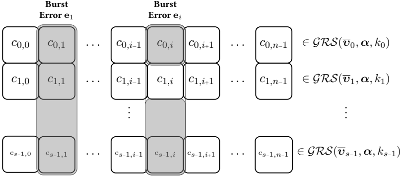
Figure 3.4: Illustration of an IGRS code \mathcal{IGRS}(\bar{\mathbf{v}}, \boldsymbol{\alpha}, \mathbf{k}) , where each sub-code is a GRS code \mathcal{GRS}(\bar{\mathbf{v}}_t, \boldsymbol{\alpha}, k_t) , for all t \in [s] . Two burst errors \mathbf{e}_1, \mathbf{e}_i \in \mathbb{F}_q^s occurred at position 1 and i . The second burst error \mathbf{e}_i has one zero component e_{i,1} .
