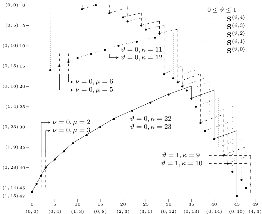
Figure 4.2: Illustration of the row pointer (\vartheta, \kappa) of Algorithm 4.2 applied to a 48 \times 50 Block-Hankel matrix \mathbf{S} . The matrix consists of two vertically arranged bands of five horizontally arranged Hankel matrices. The first band consists of 32 rows and the second one of 16. The plotted matrix \mathbf{S}' consists of the rearranged columns and rows of the matrix \mathbf{S} under \prec_{k-1}^H - respective \prec_n^V -ordering. The mixture of rows of the two vertical lines starts in line 16 (marked by the dotted horizontal line). The five zig-zag lines trace the row pointer for the five sub-blocks (\mathbf{S}^{(0,0)} \mathbf{S}^{(1,0)})^T , (\mathbf{S}^{(1,0)} \mathbf{S}^{(1,1)})^T, \dots, (\mathbf{S}^{(4,0)} \mathbf{S}^{(4,1)})^T of two vertically arranged Hankel matrices. The second axis of abscissae shows the column pointer (\nu, \mu) indicating the \mu -th column of the sub-block (\mathbf{S}^{(0,\nu)} \mathbf{S}^{(1,\nu)})^T .
