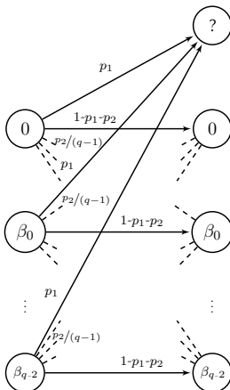
Figure 3.2: The q -ary symmetric error/erasure channel: The symbols of the q -ary alphabet are mapped to a (q + 1) -ary alphabet with erasure probability p_1 and with error probability p_2 .
