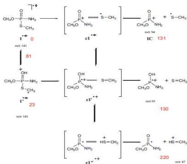
Scheme 7. Fragmentation pathways of electron ionized methamidophos 1^+ (in red, calculated B3LYP/6-31+G(d) \Delta H^\ddagger_{298} values, in \text{kJ mol}^{-1} ). (For interpretation of the references to colour in this scheme, the reader is referred to the web version of this article.)
