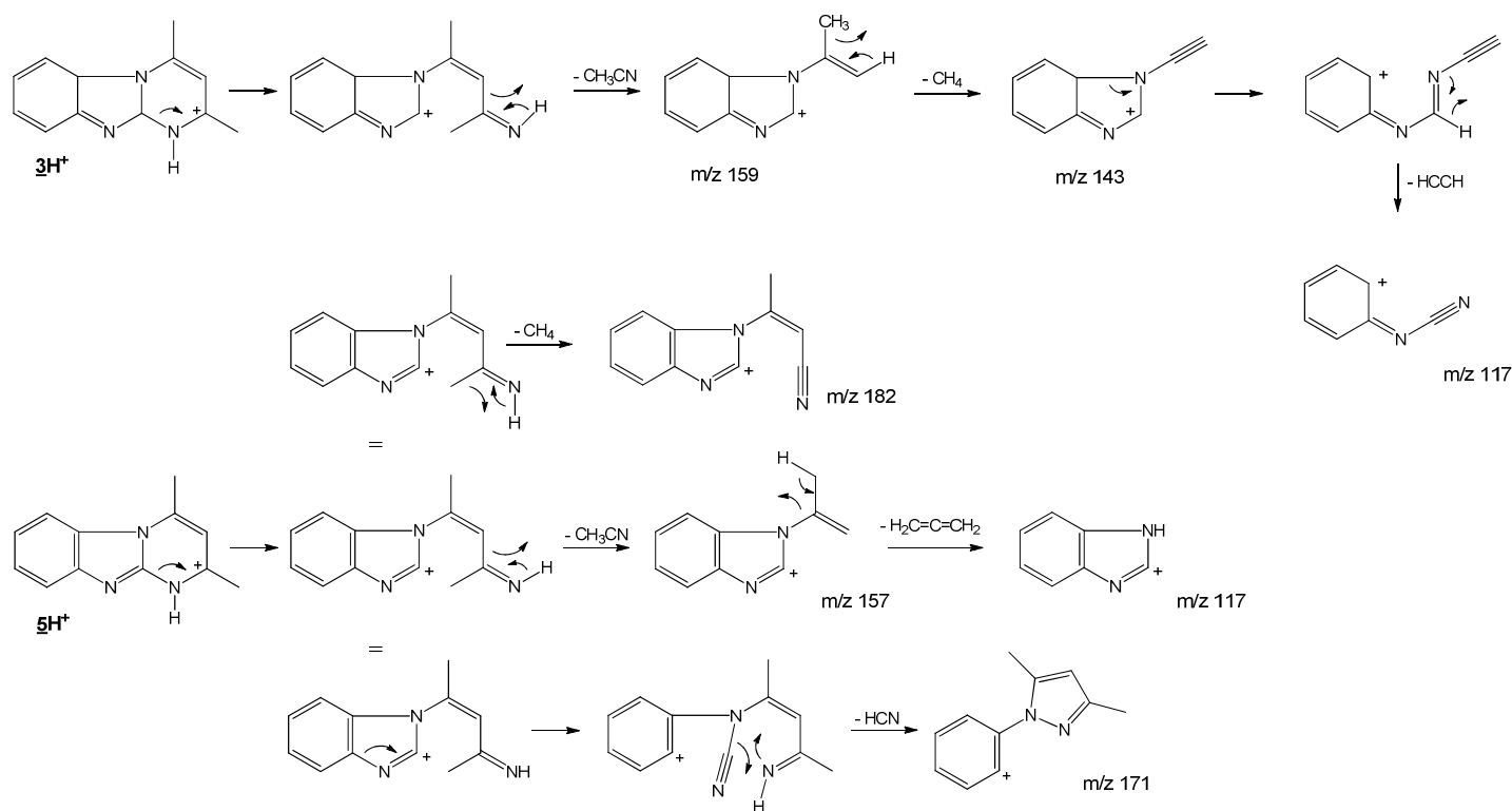
Figure 5. Dissociation pathways of pseudo molecular ions of 3 and 5 .
