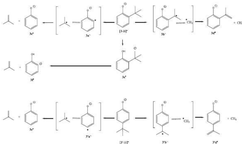
Scheme 7. Elimination pathways of \text{CH}_2 = \text{C}(\text{CH}_3)_2 from [\text{3-H}]^- ions of 2-terbutylphenol and from [\text{3}'\text{-H}]^- ions of 4-terbutylphenol ( 3 and 3' , m/z 149).
