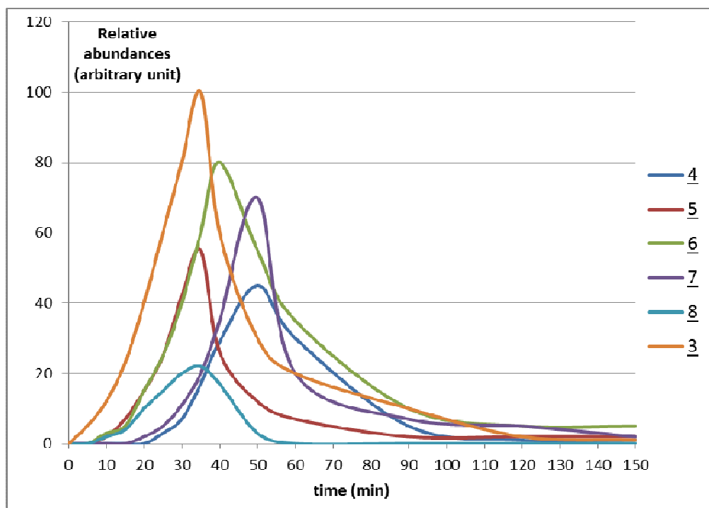
Figure 2. Relative abundances of photoproducts as a function of irradiation time – estimation based on the total ionic current in GC-MS (top) and in LC-MS (bottom)
