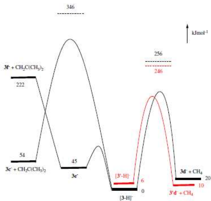
Figure 7. H^{\circ}_{298} ( \text{kJ}\cdot\text{mol}^{-1} ) profiles for the eliminations of \text{CH}_4 or \text{CH}_2\text{C}(\text{CH}_3)_2 from [3\text{-H}]^- and [3'\text{-H}]^- ( 3=2\text{-t-butyl-phenol} , 3'=4\text{-t-butyl-phenols} ).
