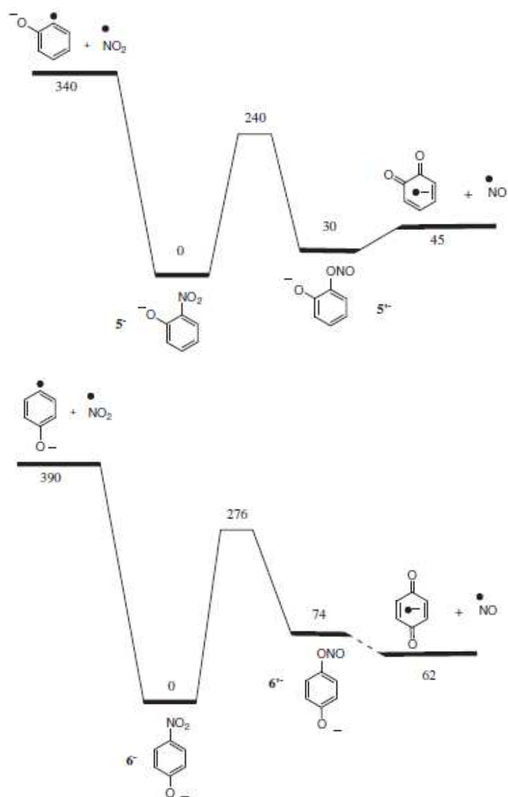
Figure 5. H_{298}^{\circ} (kJ.mol -1 ) profiles for the eliminations of \cdot NO or \cdot NO 2 from ortho and para nitro-phenoxide ions.
