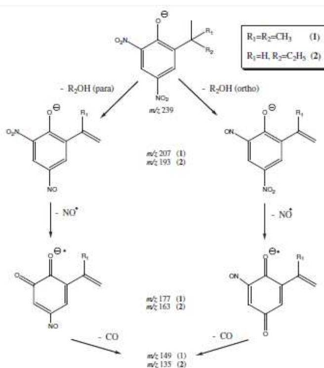
Scheme 10. Model of alcohol elimination from [1-H] - and [2-H] - ions of Dinoterb and Dinoseb respectively.
