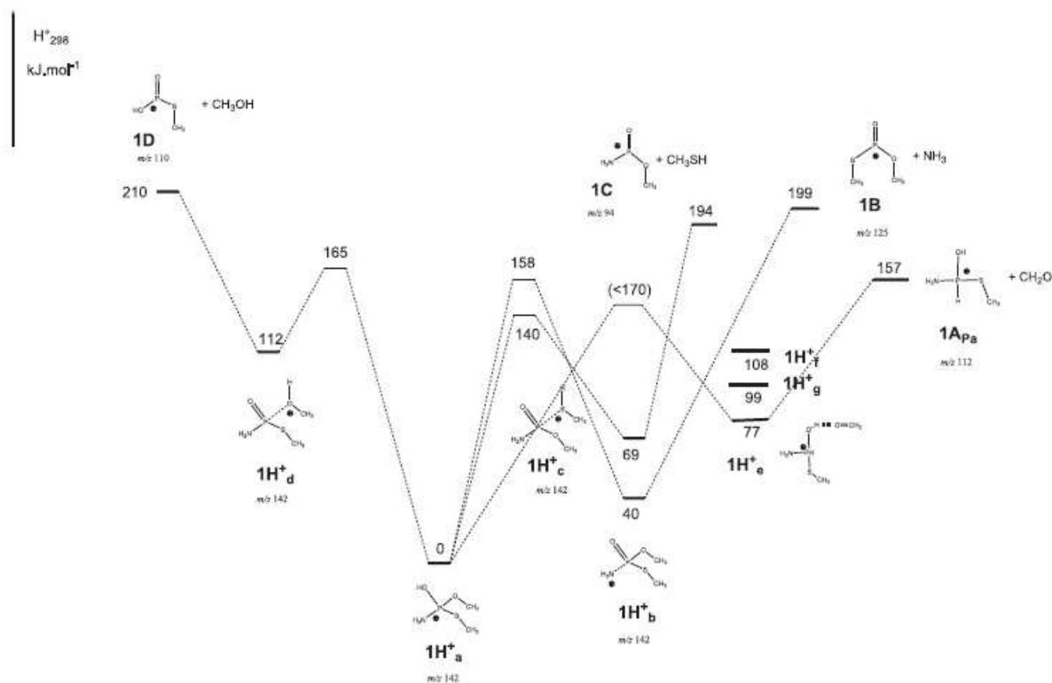
Fig. 3. H^{\circ}_{298} diagram associated with fragmentations of protonated methamidophos 1H^+ (B3LYP/6-311+G(3df,2p)//B3LYP/6-31+G(d) calculations).
