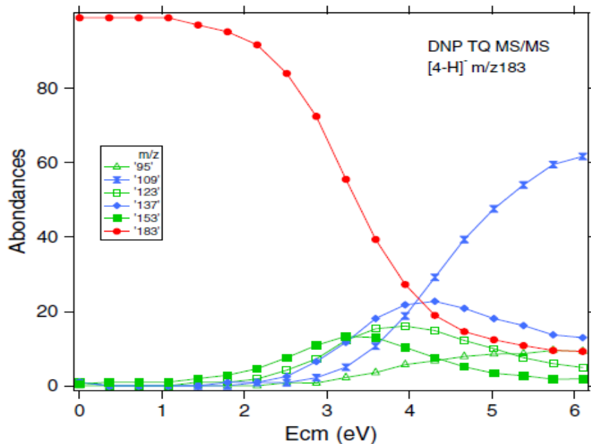
Figure 4. Breakdown graph associated with the decomposition of [4\text{-H}]^- (4=2,4-dinitrophenol) ( m/z 183).
