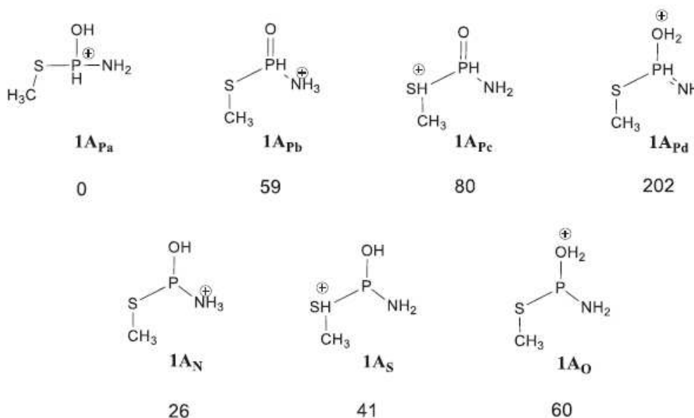
Scheme 4. Calculated B3LYP/6-311+G(3df,2p)//B3LYP/6-31+G(d) relative \Delta H_{298}^{\circ} ( \text{kJ mol}^{-1} ) of various possible structures of m/z 112, [\mathbf{1H}^+ - \text{CH}_2\text{O}] , ions.
