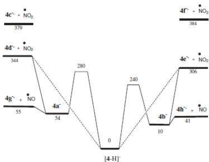
Figure 6. H^\circ_{298} ( \text{kJ}\cdot\text{mol}^{-1} ) profiles for the eliminations of \cdot\text{NO} or \cdot\text{NO}_2 from [4\text{-H}]^- (4=2,4-dinitrophenol).
