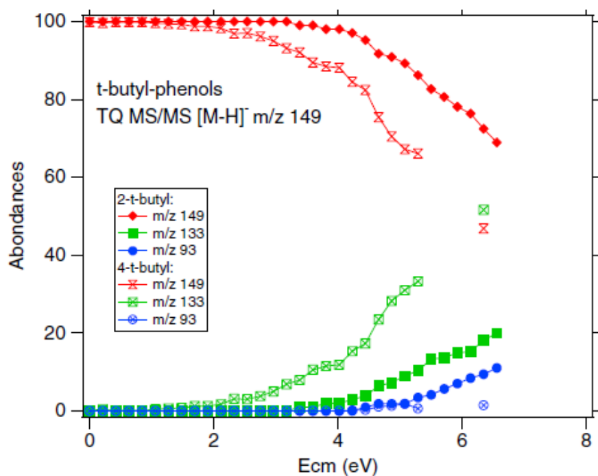
Figure 3. Breakdown graph associated with the decomposition of [3\text{-H}]^- and [3'\text{-H}]^- (3=2-t-butyl-phenol, 3'=4-t-butyl-phenols) ( m/z 149).
