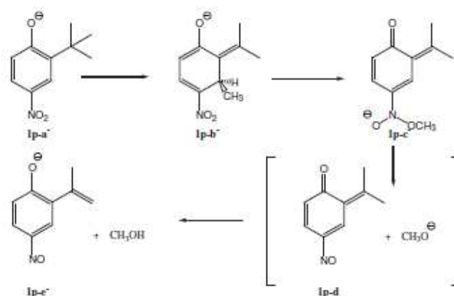
Scheme 9. Model of alcohol elimination from [1p-H]^- ions of para nitro-tbutylphenol.
