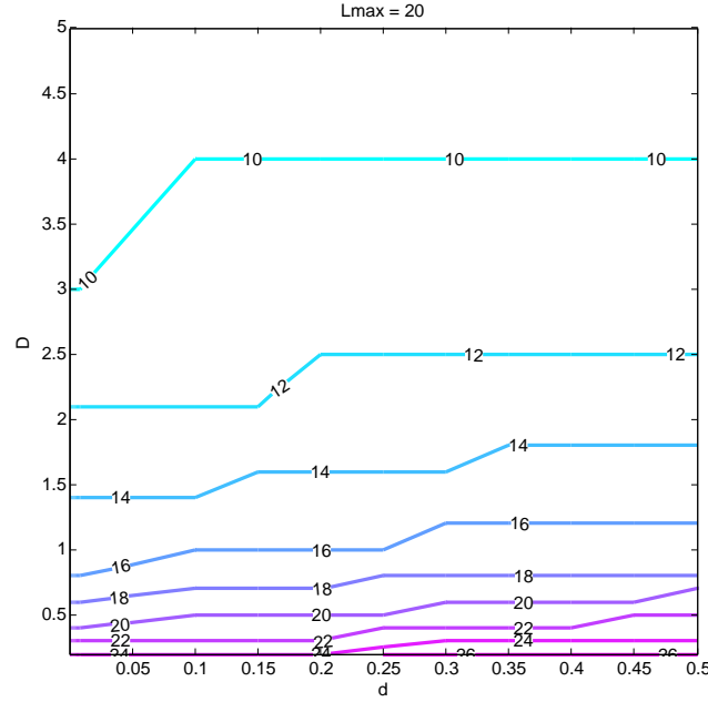
Figure 6.9: \tilde{L}_{max}(d, D) .
