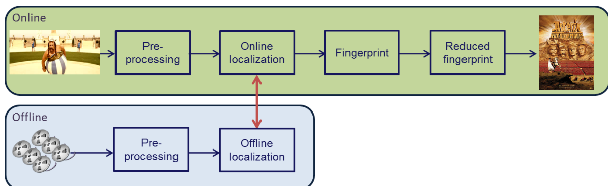
Fig.II.1 TrackART system functional schema
