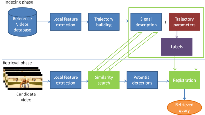
Fig.I.22: Video copy detection framework in [LAW 07]
