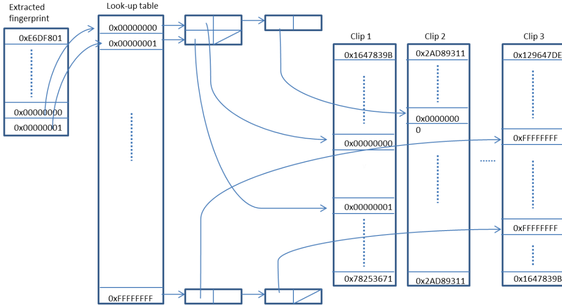
Fig.I.20: Look up table for database efficiency
