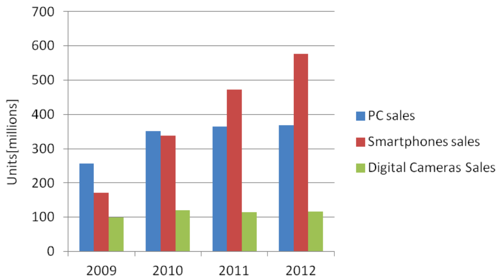
Fig. 1.2: Sales in PCs, smart phones and digital cameras 2009-2012 [GAR 12]
