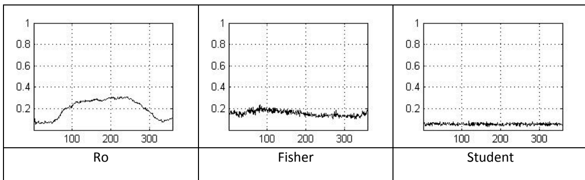
Fig.II.15: The results of the Ro, Fisher, and Student tests in (9,7) DWT domain ( L = 35000 frames, R = 360 coefficients, and D = 250 frames)
