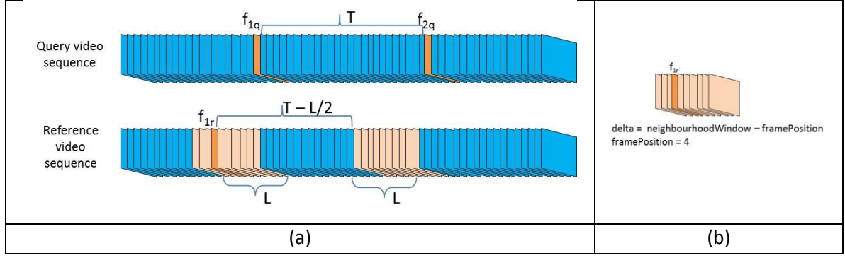
Fig.II.18 Synchronization algorithm first stage
