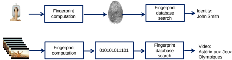
Figure 1: Human versus video fingerprinting
