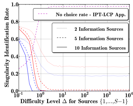
(f) \Delta_s = 1
