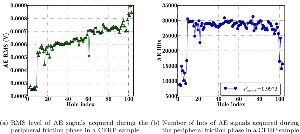
Figure 5.27 – Feature extraction results obtained with studying the peripheral friction phase of a drilling operation on a CFRP sample
