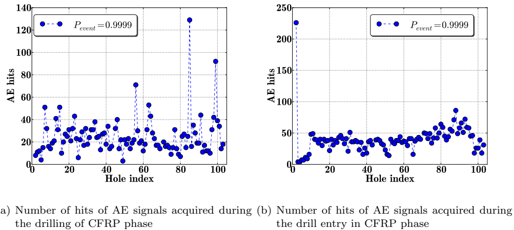
Figure 5.26 – Feature extraction results obtained with the proposed approach applied on the drilling phase of a drilling operation on a CFRP sample (a), and the drill entry phase (b)
