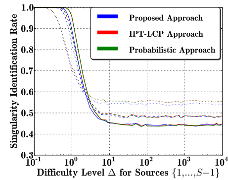
(e) \Delta_s = 1
