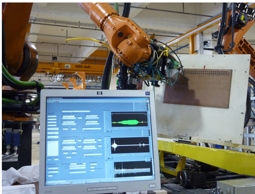
Figure A.3 – Test bed used for test campaign number 4
