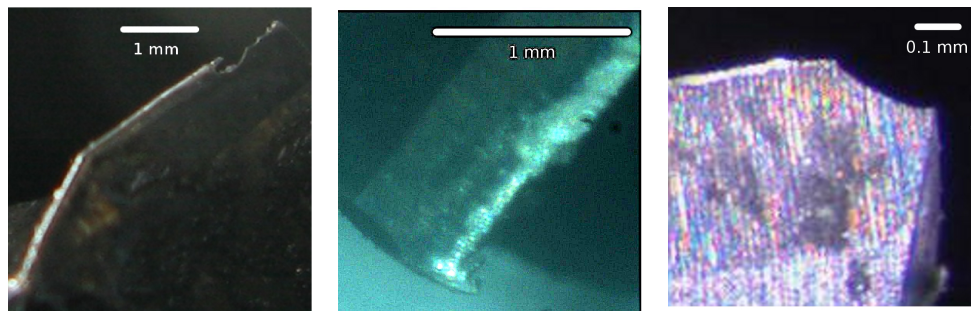
(a) Cutting edge chipping provoked during the 1 st test campaign (b) Cutting edge chipping provoked during the 2 nd test campaign (c) Cutting edge chipping provoked during the 3 rd test campaign
