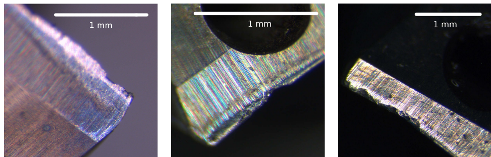
(d) Cutting edge chipping that appeared during the 4 th test campaign (e) Cutting edge chipping provoked during the 5 th test campaign (f) Cutting edge chipping provoked during the 6 th test campaign
