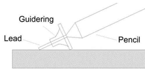
Figure 5.6 – Principle of an Hsu-Nielsen test: breakage of a pencil lead in repeatable conditions at the surface of a sample were AE sensors are mounted allow to characterize their response, or here the quality of the transmission of AE
