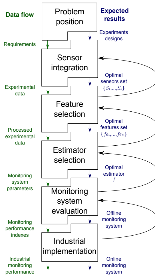
Figure 3.9 – Proposed approach for the implementation of industrial process monitoring systems: eventual feedbacks are represented by gray arrows while data flow and expected results at the end of each steps are given in green and blue respectively. The term optimal is related to the performance level of the monitoring system
