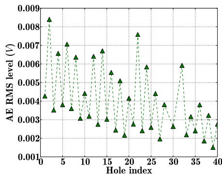
(a) RMS level of AE signals acquired during the drilling of CFRP phase (b) Number of hits of AE signals acquired during the drilling of CFRP phase
