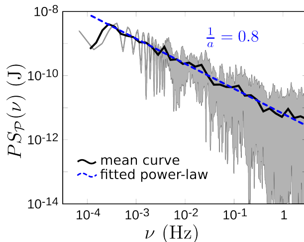
Figure 3.2: Power spectrum of elastic energy derivative signal ( \mathcal{P} ) and its mean curve in logarithmic scale. The blue dashed line represents the fitted power-law. This is computed for sample Sa_1 ( d = 500 \mu\text{m} , V = 16 \text{ nm/s} , no porosity).
