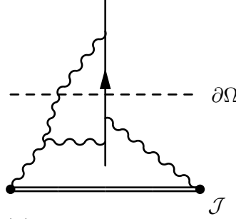
Figure 4.14: The [\alpha_{\mathbf{k}} \cdot \mathbb{T}_u^A] [\xi^{(\mathbf{k}-)} \cdot \mathbb{T}_v^b] b_{\mathbf{p}}(x) contribution. The fermion is cut on the initial surface and replaced by a \xi_{\mathbf{p}}^{(\mathbf{k}+)} vertex 4.9 whose gluon leg matches the cut gluon one-point function.
