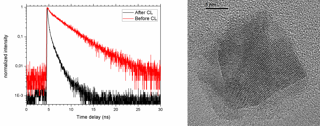
Figure 3.12.: (left) Fluorescence decay curves of a single CdSe/CdS QD on silicon TEM grid, before and after observation of CL in the STEM. The lifetime is reduced by a factor 7-8. (right) HRTEM image of the QD taken after the CL observation.
