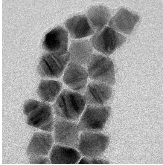
(a) TEM images of CdSe/CdS thick shell QDs, showing polytypic structure (obtained at magnification \times 120000 ).
