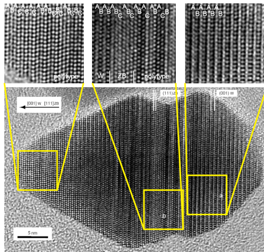
(b) Core-shell dot with wurtzite-zincblende polytypism (obtained at magnification \times 300000 , courtesy of P. Bassoul). From left to right, the magnified areas represent: - a polytypic area, - an area with side by side wurtzite, zincblende and polytypic domains, - a wurtzite domain.
