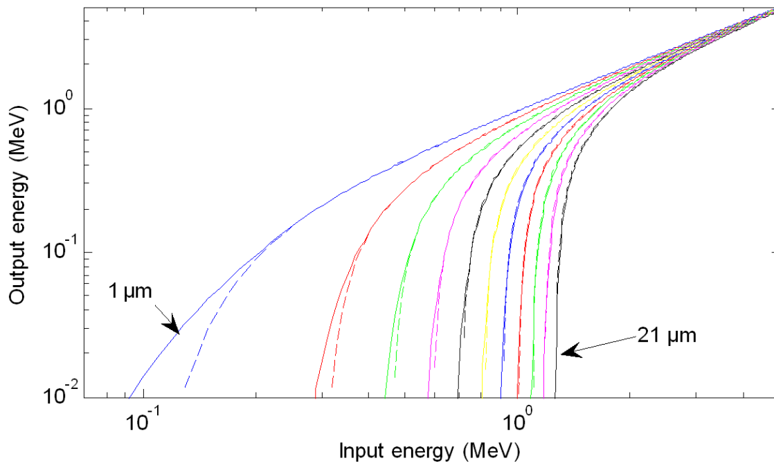
Figure IV-4: Energy of a proton emerging from, respectively, a 300\ \text{K} (dotted lines) and 20\ \text{eV} (plain lines) solid density aluminum foil of various thickness ( 1, 3, 5, 7, 9, 11, 13, 15, 17, 19, and 21\ \mu\text{m} ) as a function of its initial energy.
