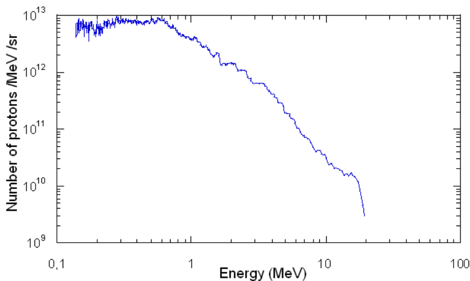
Figure I-14: Typical proton beam spectrum generated by the 100 TW high-intensity short-pulse laser at LULI (1 \mu\text{m} wavelength, 400 fs, 25 J, intensity around 5 \times 10^{19} W/cm 2 on a 10 \mu\text{m} gold target).
