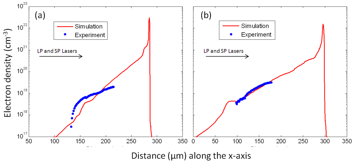
Figure III-39: Density profiles corresponding to a 500 nm plastic target irradiated by a long pulse of intensity of respectively, (a) 3 \times 10^{14} , (b) 3 \times 10^{15} W/cm 2 , 400 and 0 ps prior to the peak of the long laser pulse ( \Delta t = -400 and 0 ps). Blue dots indicate the density profiles obtained by the Interferometry diagnostic, red lines by CHIC simulations. The experimental profiles are extracted at a distance of 10 \mu\text{m} from the center of the expansion to avoid uncertainties caused by the Abel inversion.
