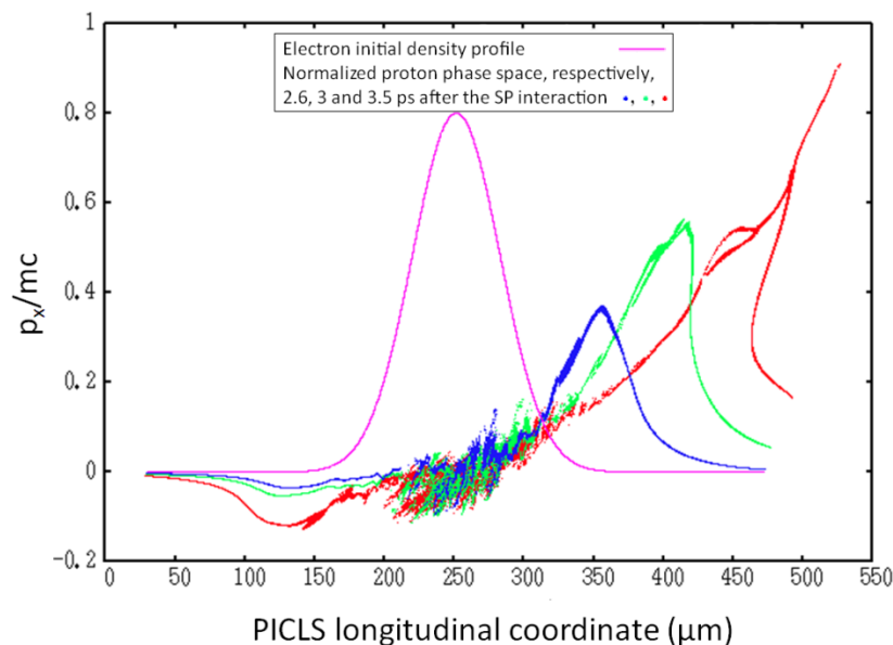
Figure III-50: Normalized proton phase space obtained predicted by a PICLS simulation for a SP of intensity 5 \times 10^{20} \text{ W/cm}^2 , pulse duration 700 fs (FWHM) and the focal spot diameter of 6 \mu\text{m} (FWHM) interacting with a 80 \mu\text{m} thick (FWHM) plastic target (the electron density profile is normalized to the critical density of the laser). The laser is focused 150 \mu\text{m} from the left boundary.
