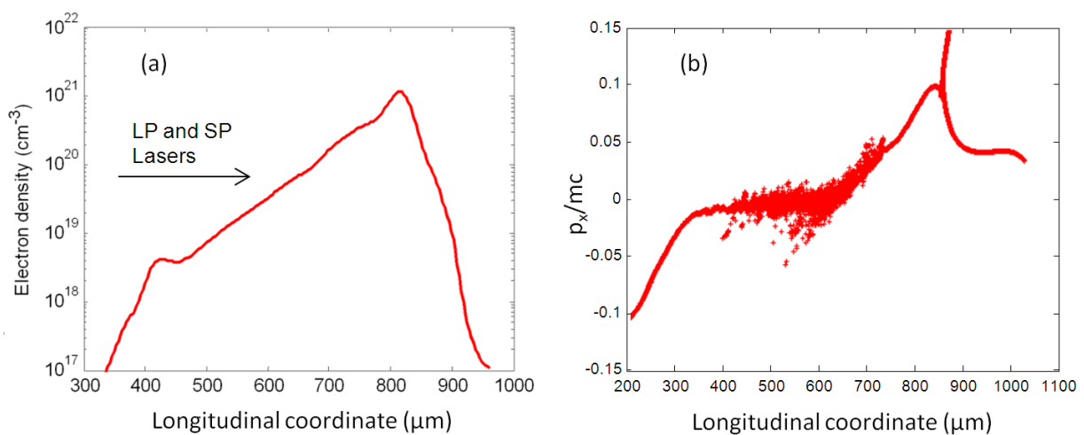
Figure III-47: Density profile obtained with CHIC for a 500 nm plastic foil exploded with a 10^{14} \text{ W/cm}^2 intensity and a +100 ps delay (a) and normalized proton phase space in the longitudinal direction 7.42 ps after the interaction of the maxi-
