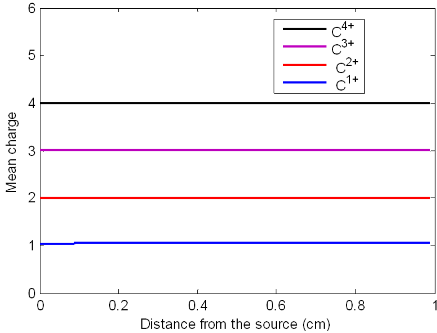
Figure IV-40: Evolution of the mean charge of several 0.1 MeV/u monoenergetic beams composed, respectively of only C 1+ , C 2+ , C 3+ and C 4+ when propagating with the co-moving electrons, according to FLYCHK.
