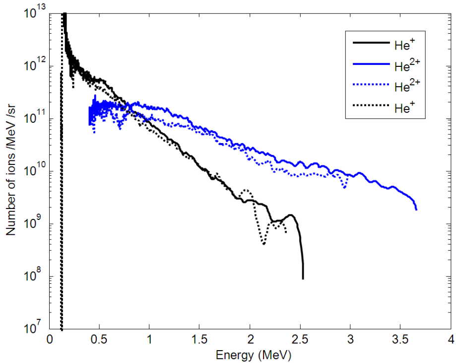
Figure III-25: Spectra of ions accelerated in a 100 bar helium gas jet by a 0.7 ps laser pulse focusing at the edge of the gas 0.75 (discontinuous lines) and 1mm (continuous lines) above the nozzle.
