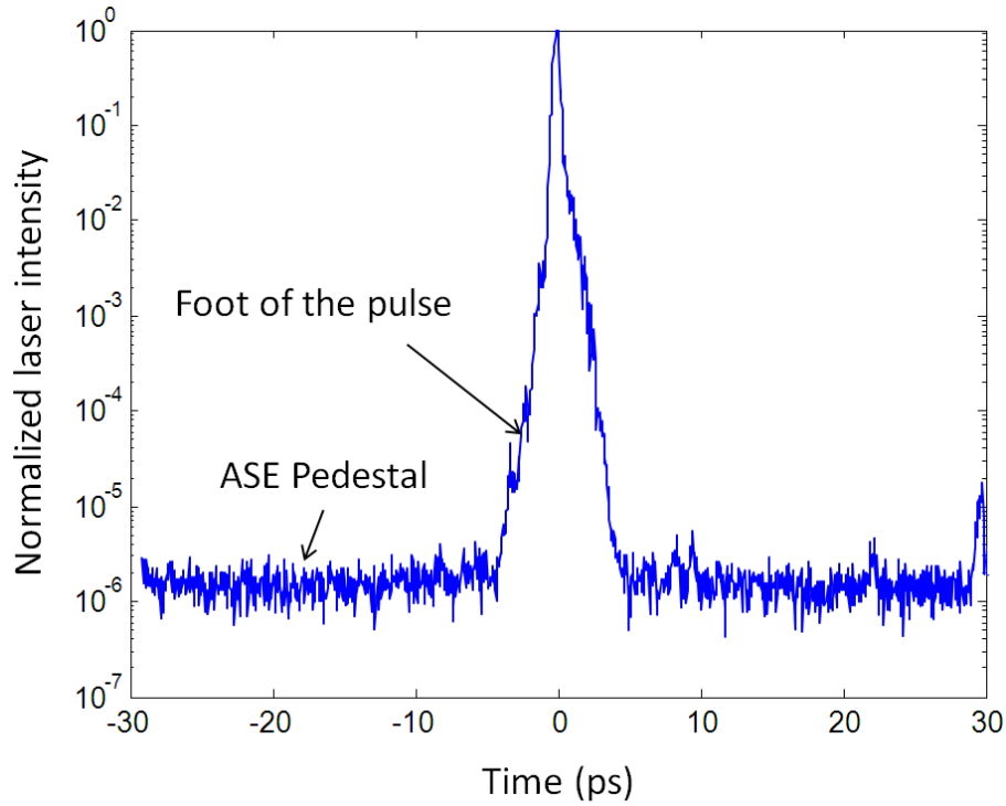
Figure III-1: Temporal profile of the ELFIE compressed beam obtained using a 3\omega autocorrelator, where \omega is the laser frequency. The intensity is normalized to the maximum intensity of the pulse. The curve corresponds to an ASE contrast below 4 \times 10^6 , the noise limit of the measuring device.
