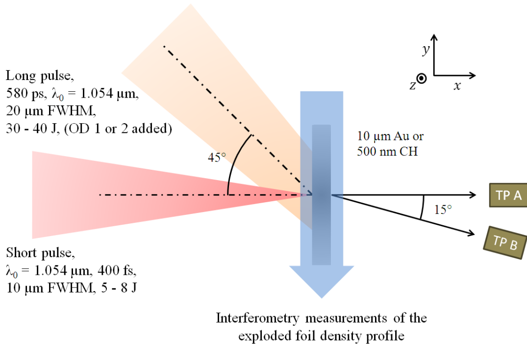
Figure III-31: Experimental set-up.
