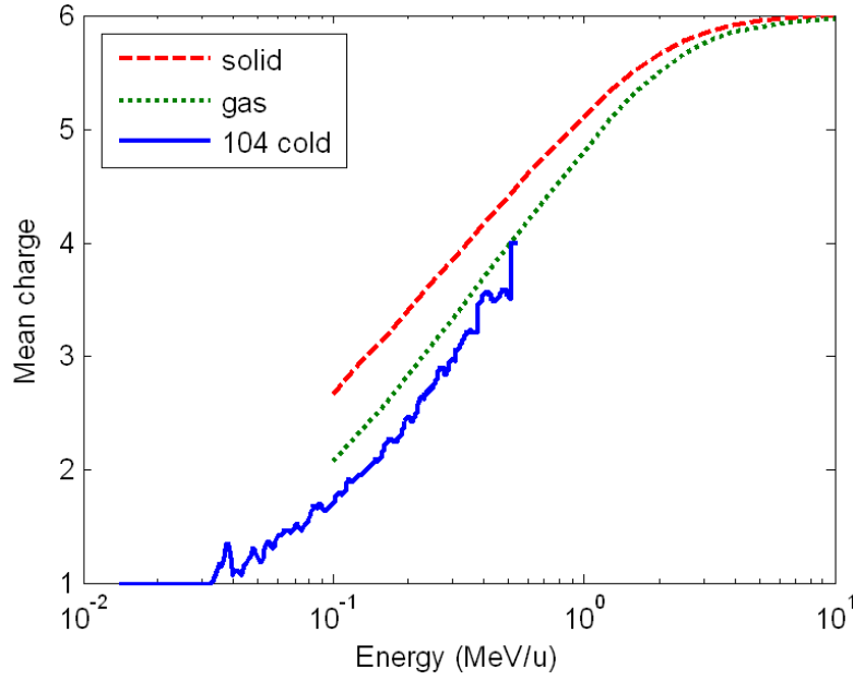
Figure IV-35: Comparison between our experimental mean charge and the equilibrium mean charge in, respectively, cold solid-density aluminum (curve) and in cold nitrogen gas (dotted curve) given in Refs [33, 58]. According to the validity range given for these two formulas, they can be used for energy above 0.1 MeV/u in our case. Their relative error bars in charge is estimated around 16 %.
