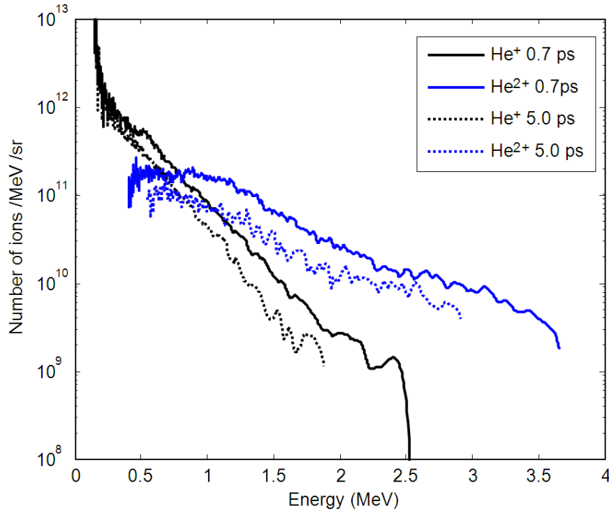
Figure III-26: Spectra of ions accelerated in a 100 bar helium gas jet by respectively 0.7 (continuous lines) and 5 ps (discontinuous lines) laser pulses focused at the edge of the gas jet.
