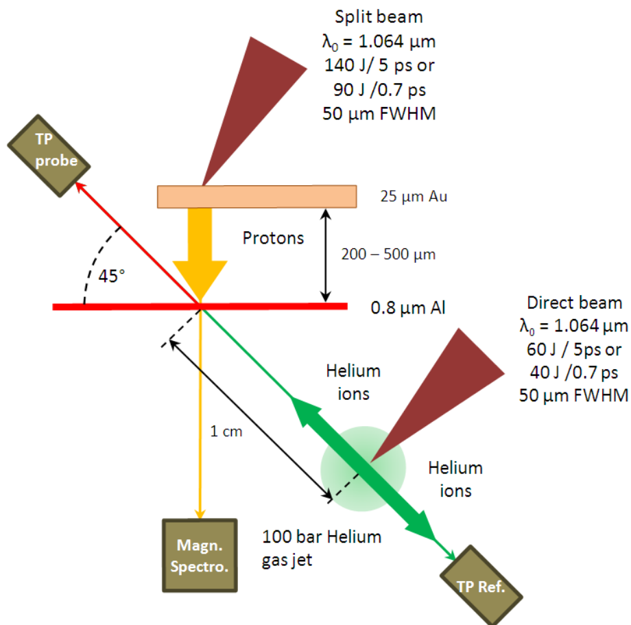
Figure IV-43: Experimental set-up.
