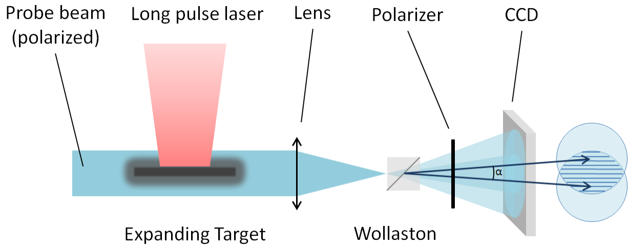
Figure III-34: Interferometer set-up.
