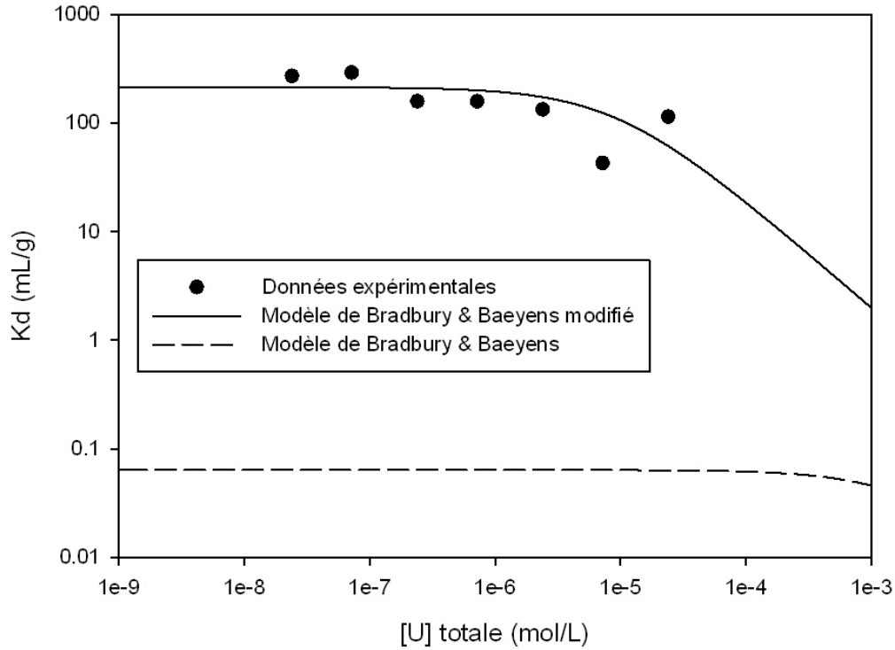
FIGURE 4.22 – Modélisation de l'isotherme K_d(\text{U(VI)-Argile}) à pH = 8 , pCO_2 = 10^{-2} \text{ atm} , [NaCl] = 10^{-2} \text{ mol/L} , S/L = 0, 5 \text{ g/L} .
