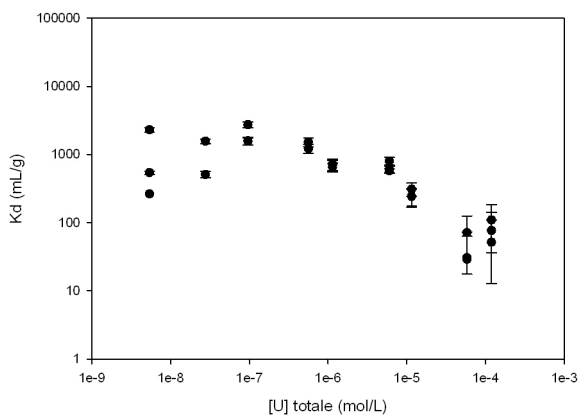
FIGURE 4.19 – Isotherme K_d(\text{U(VI)-Argile}) à pH = 4 , pCO_2 = p_{atm} , [\text{NaCl}] = 6,4 \cdot 10^{-3} \text{ mol/L} , S/L = 0,5 \text{ g/L} .
