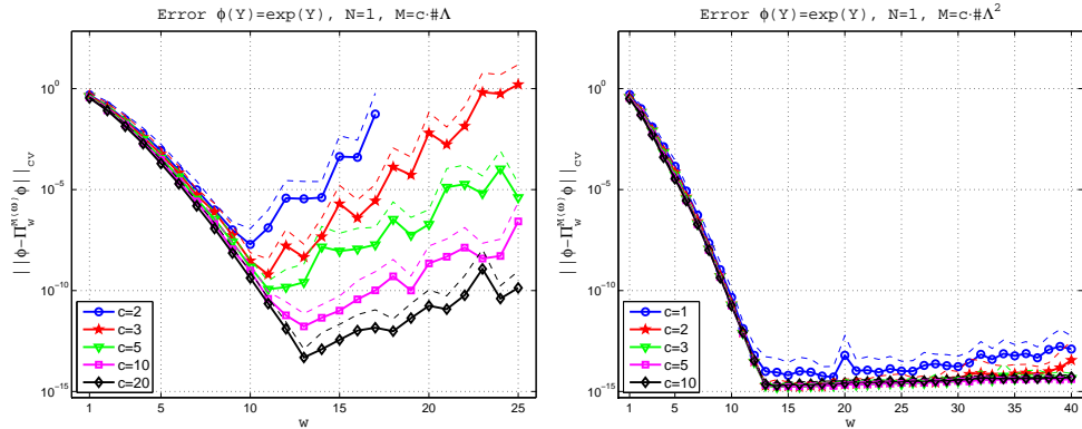
Figure 3.18: Approximation error (1.4.6) with the exponential function (3.4.1), averaged over 100 repetitions. Left: M = c \cdot \#\Lambda . Right: M = c \cdot (\#\Lambda)^2 . Beta density \mathcal{B}(2, 2) .
