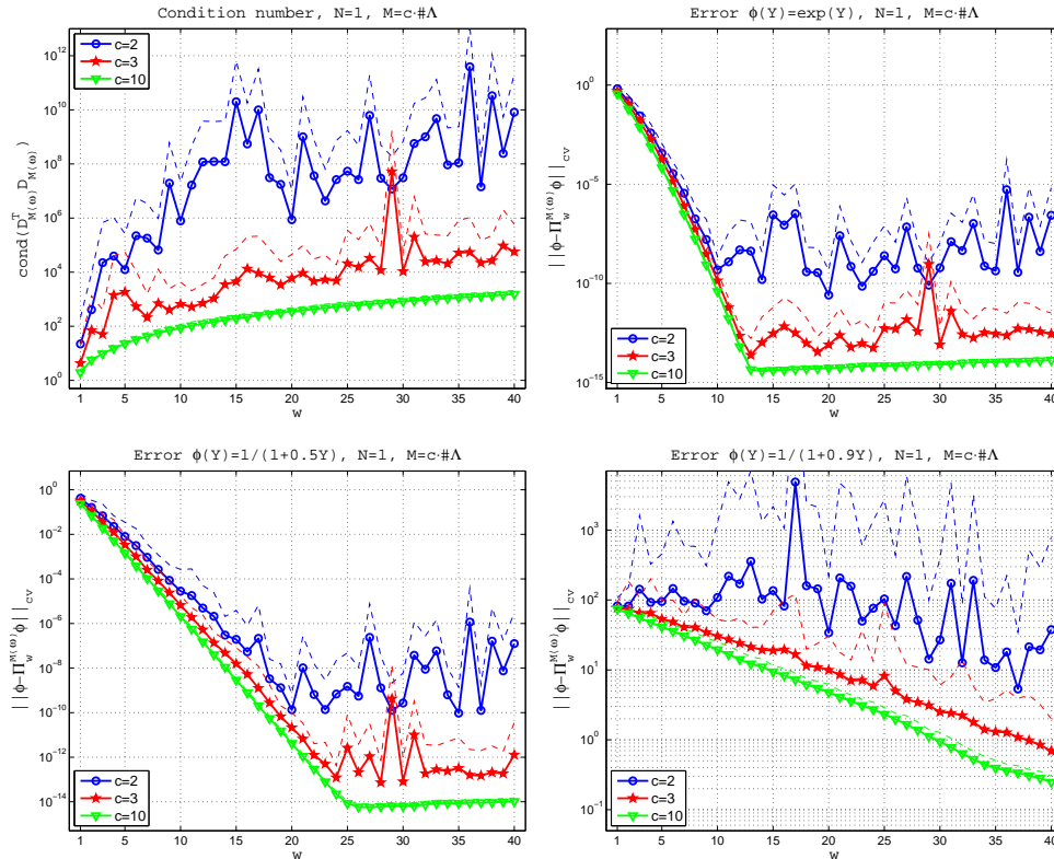
Figure 3.3: Condition number (1.4.9) and approximation error (1.4.6) with the smooth target functions (3.4.1), (3.4.2), (3.4.3), averaged over 1000 repetitions, M = c \cdot \#\Lambda . Beta density \mathcal{B}(0.5, 0.5) .
