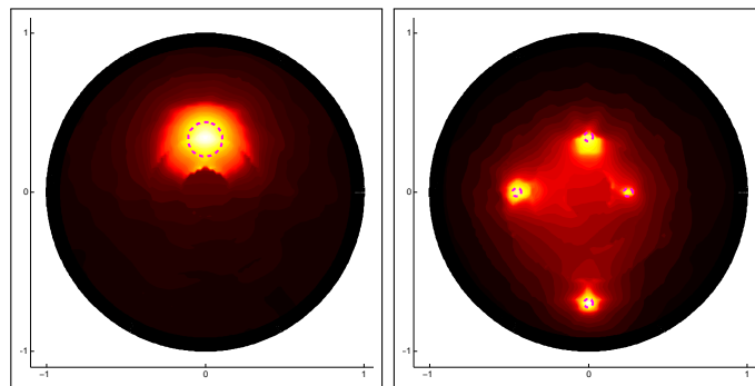
Figure 5.8: Coloring of C(\xi) . Left: test case i2UN, \gamma = 5 \cdot 10^{-2} in (5.2.25). Right: test case i2US, \gamma = 10^{-2} in (5.2.25).
