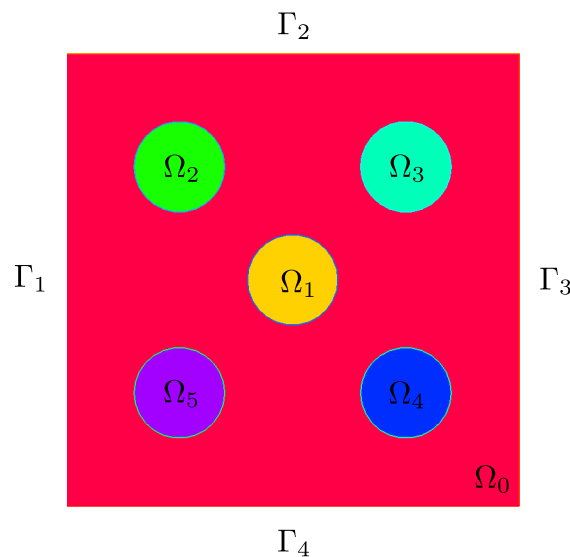
Figure 4.7: Domain with five inclusions \Omega_1, \Omega_2, \Omega_3, \Omega_4, \Omega_5 with random diffusivity for problem (4.3.8).
