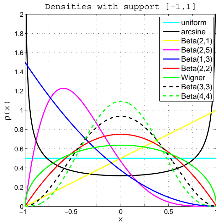
Figure 3.2: Some probability densities in the beta family with support in [-1, 1] .
