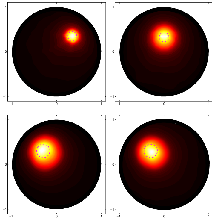
Figure 5.26: Tikhonov regularization. Test case I, \gamma = 10^{-2} (top-left). Test case II, \gamma = 5 \times 10^{-2} (top-right). Test case IIIa, \gamma = 10^{-1} (bottom-left). Test case VI, \gamma = 10^{-2} (bottom-right).
