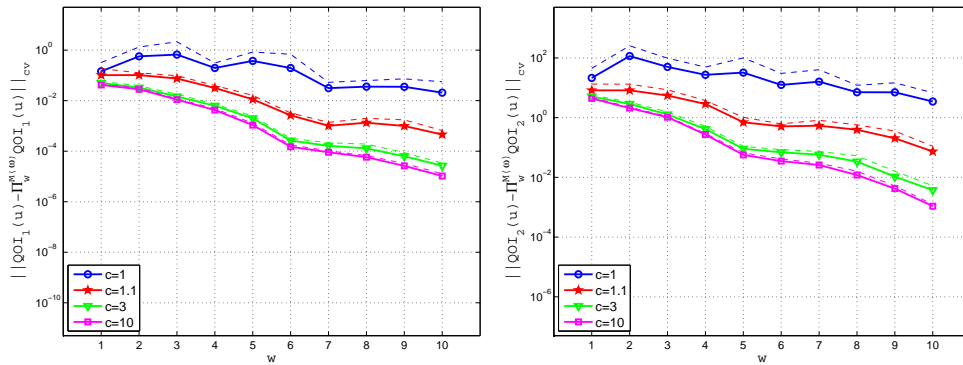
Figure 4.9: Example 3: the Darcy model. \beta = 5 . Approximation errors (4.3.2) in the \text{QOI}_i , i = 1, 2 , using M = c \cdot \#\Lambda = c \cdot (w + 1) . Continuous lines: sample mean averaged over R = 100 repetitions. Dashed lines: sample mean plus one sample standard deviation averaged over R = 100 repetitions.
