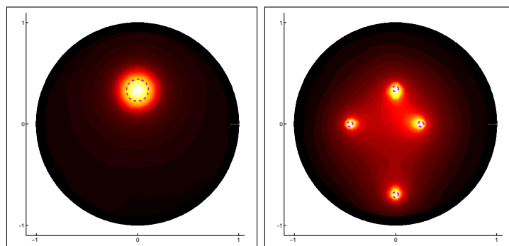
Figure 5.4: Coloring of C(\xi) . Left: test case hN, \gamma = 10^{-2} in (5.2.25). Right: test case hS, \gamma = 5 \times 10^{-3} in (5.2.25).
