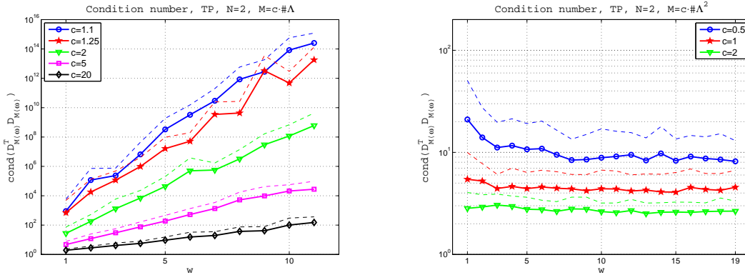
Figure 1.11: Condition number (1.4.9), TP, N = 2 . The continuous, marked, lines show the mean condition number (1.4.10) over 100 repetitions. The dashed lines show the mean (1.4.10) plus one standard deviation (1.4.11). Left: M = c \cdot \#\Lambda . Right: M = c \cdot (\#\Lambda)^2 .
