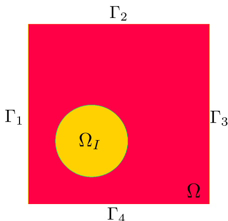
Figure 4.1: Square domain \Omega with a circular inclusion \Omega_I .
