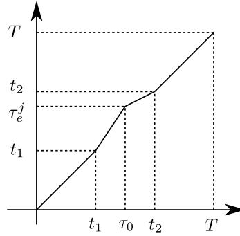
Figure 5.1: Change of variable associated with the perturbation of \tau_e^j .
