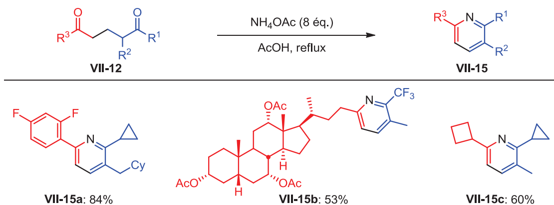
Sch\u00e9ma VII-27 – Synth\u00e8se de pyridines 2,3,6-tri-substitu\u00e9es
