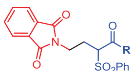
VII-12b: R = Me, 84% VII-10': R = H, 63%
