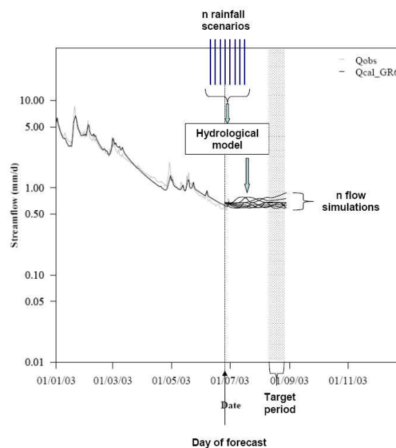
Figure 5.2: Layout of the probabilistic approach of low-flow forecasting (observed and simulated flow hydrographs of catchment J for the year 2003 is illustrated here)
