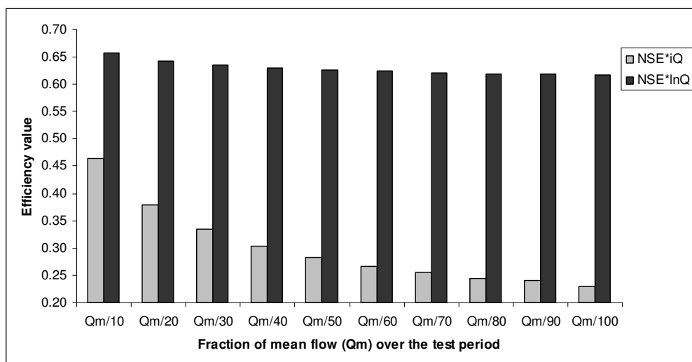
Figure 3.9: Change in the mean value of NSE_{iQ}^* and NSE_{\ln Q}^* obtained by the GR4J model in validation over the catchment set with different values of \varepsilon (fractions of Q_m from Q_m/10 to Q_m/100 )
