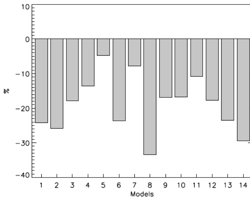
Figure 1.6: Changes in the annual discharges (using SIM model) between the 2046-2065 and 1971-2000 periods averaged over France using the inputs from 14 climate models (Source: Boé et al., 2009)
