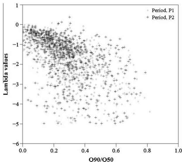
Fig. 12. Scatter plot of Q_{90}/Q_{50} vs. lambda values ( \lambda ) for the two test periods for the GR4J model.
