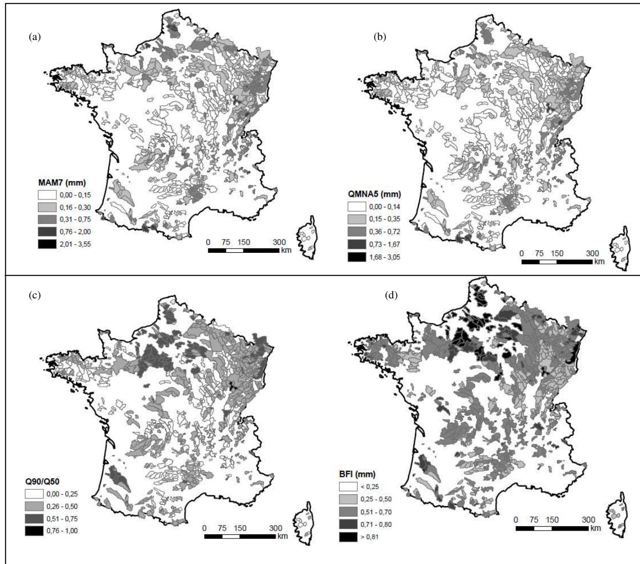
Figure 2.6: Illustration of spatial variability of the low-flow indices: (a) - MAM 7 ; (b) - QMNA 5 ; (c) - Q 90 /Q 50 ; (d) - BFI
