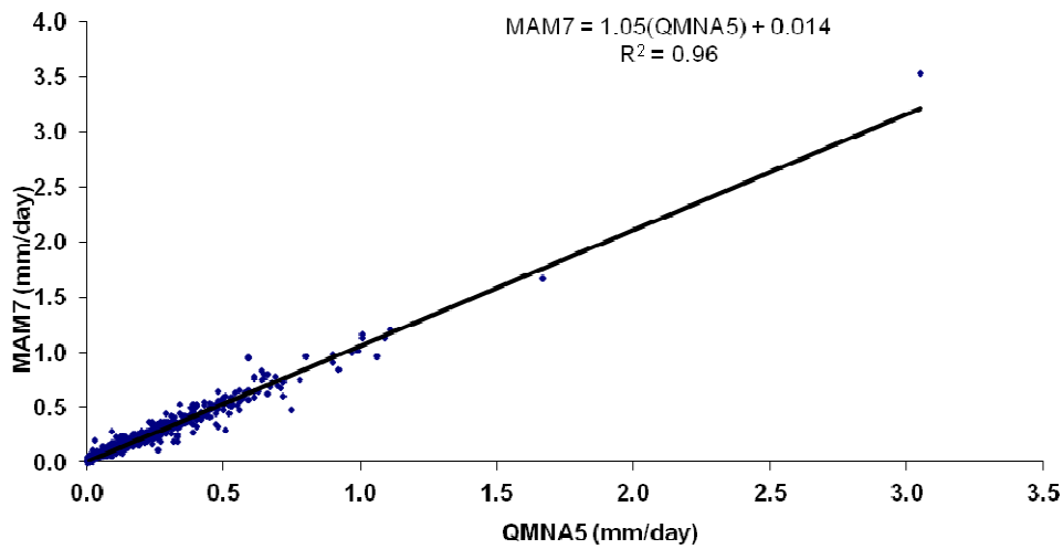
Figure 2.8: Relation between QMNA_5 and MAM_7
