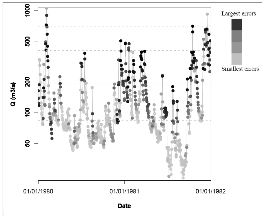
Figure 3.5: Illustration of flow values that contribute the most of the total model error. The error considered here is the square error calculated on flows. The darker the dots, the larger the contribution to the total error. Horizontal dashed lines correspond to the percentiles of the box plot shown in Figure 3.4.
