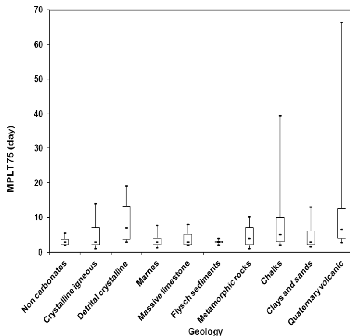
Figure 5.18: Possible link of lead-time with catchment geology
