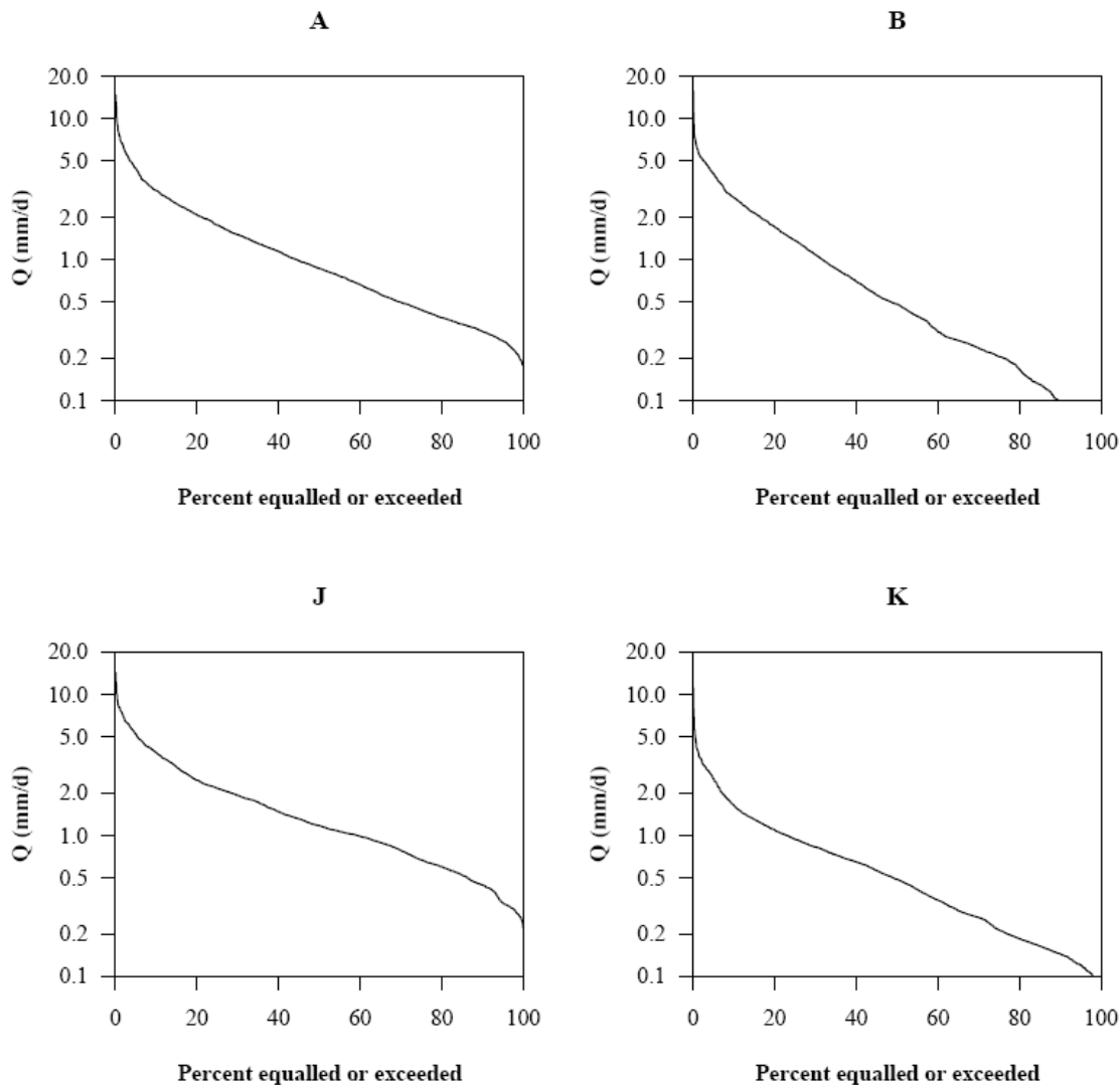
Figure 2.5: Flow duration curve of the sample catchments for a period of 2003 to 2005 (the values below 0.1 mm/d are not shown)
