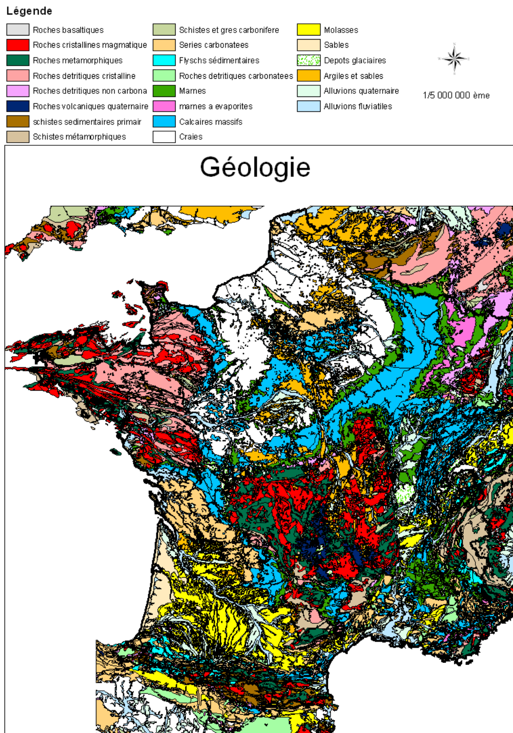
Figure 1.4 Geological map of France (Source: Geological Survey of France)
