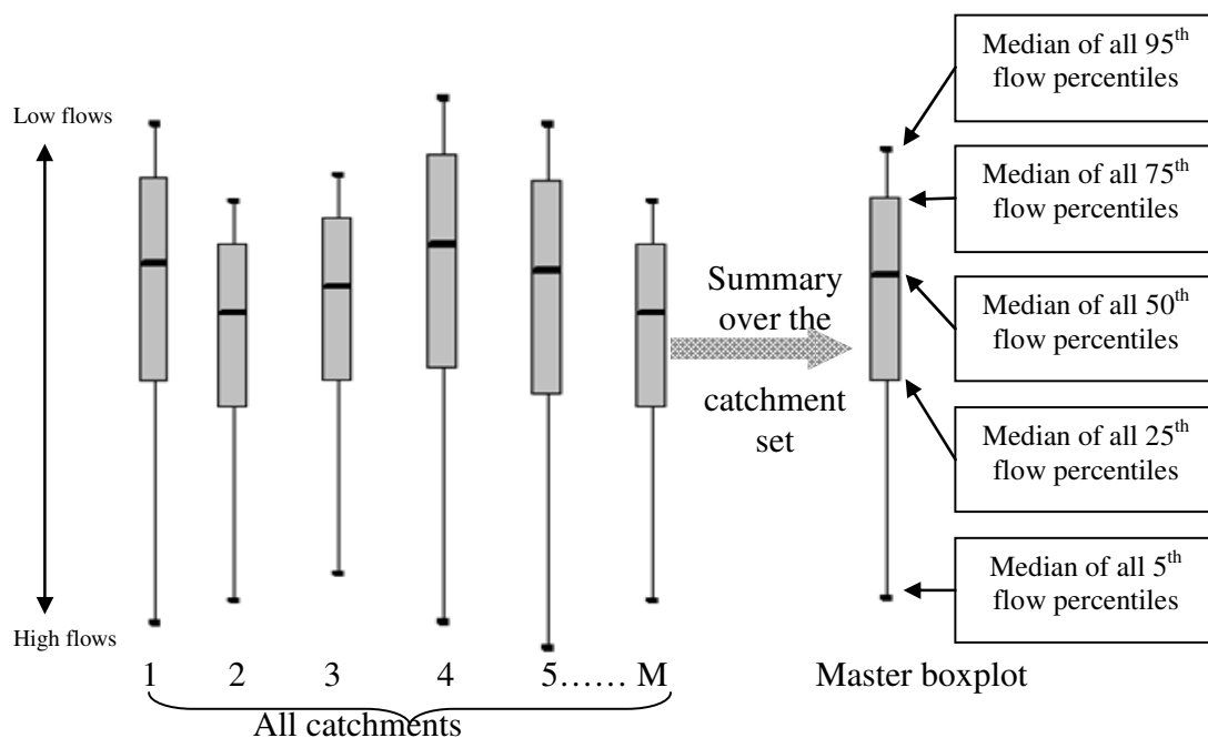
Figure 3.6: Schematic representation of the derivation of master box plot which summarizes the behaviour of a given criterion over the entire catchment set (M stands for the total number of catchments)
