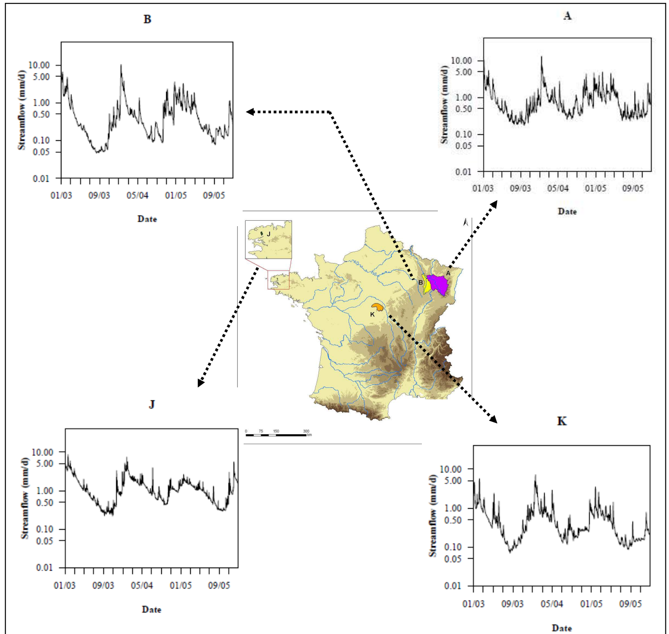
Figure 2.3: Illustration of location of sample catchments and their daily flow hydrographs from 2003 to 2005
