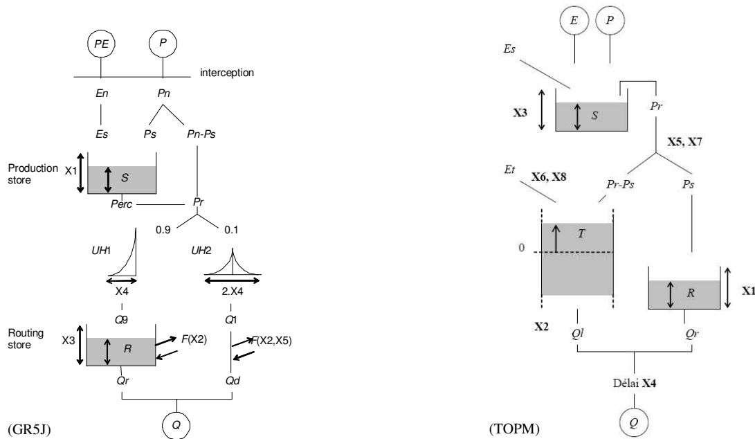
Figure 4.1: Structural layout of the base models
