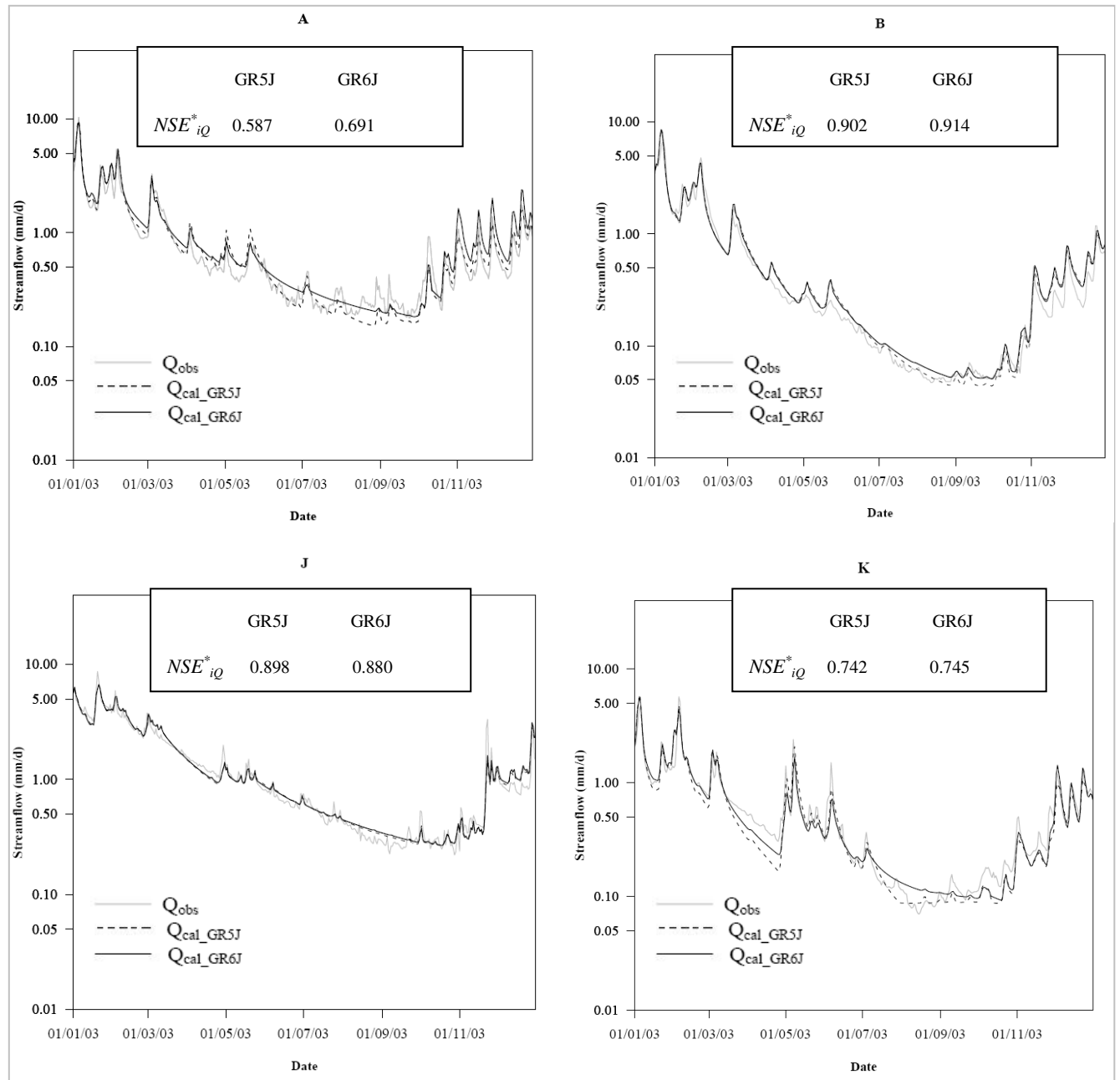
Figure 4.6: Illustration of the hydrographs simulated by the GR5J and GR6J models, with corresponding NSE^*_{iQ} efficiency values
