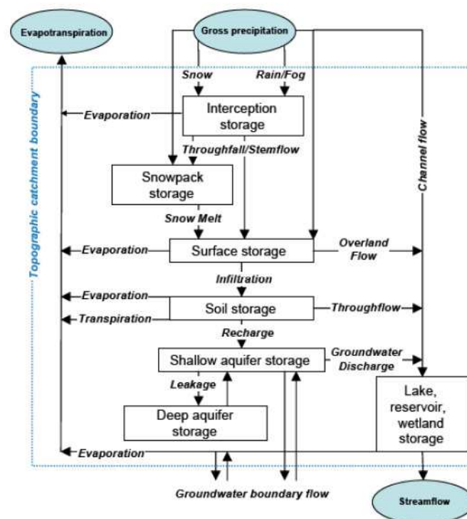
Figure 1.1: Natural hydrological processes and catchment storages (WMO, 2008)
