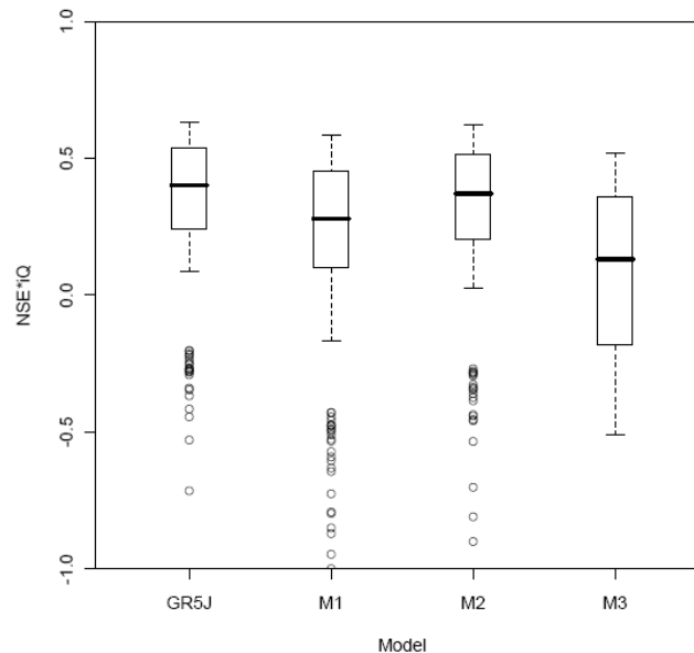
Figure 4.3: Box plots of NSE \cdot iQ values obtained in validation over the catchment set by GR5J and three model versions with modified groundwater exchange functions (boxes represent the 0.25 and 0.75 percentiles, with the median value inside, and the whiskers represent the 0.10 and 0.90 percentiles respectively)
