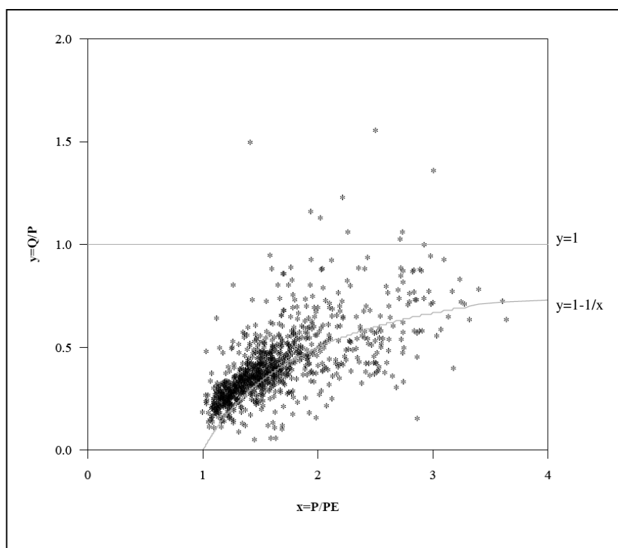
Figure 2.2: Mean Q/P vs P/PE values for the catchments in the data set
