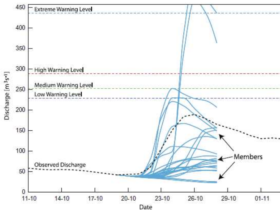
Figure 5.1: An ensemble flood forecast with different levels of warnings (Source: Cloke and Pappenberger, 2009)
