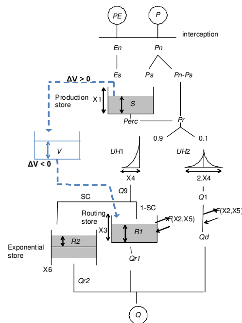
Figure 6.3: Illustration of how to account for the artificial reservoir volume variations ( \Delta V ) in the GR6J model
