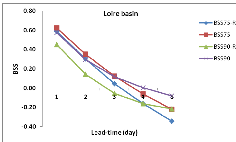
Figure 6.9: Illustration of forecast skill score of the model GR6J in the Loire basin
