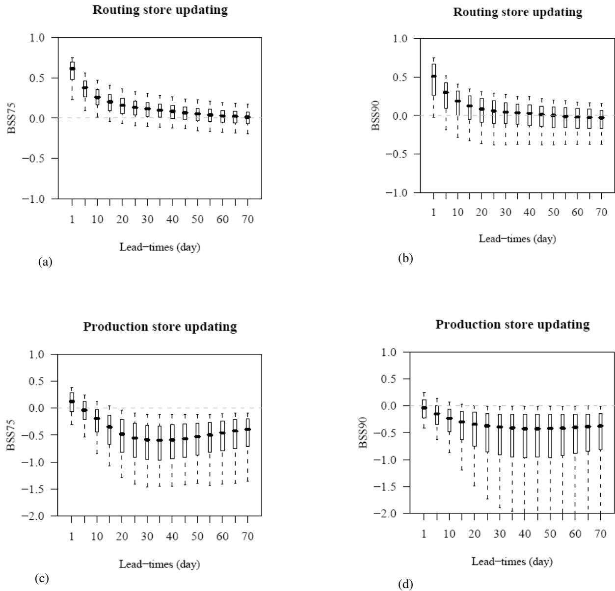
Figure 5.12: Illustration of the model's forecast skill score with the state updating ((a) & (b): updating of routing stores; (c) & (d): updating of the production store)
