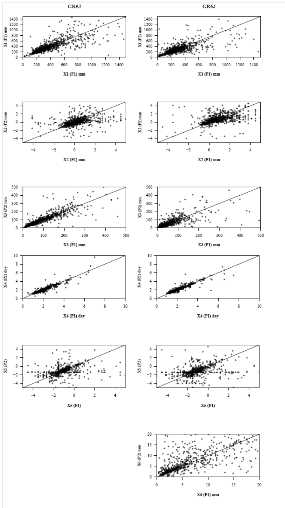
Figure 4.7: Comparison of the parameter values obtained on the two calibration periods P1 and P2 for the GR5J and GR6J models (1:1 line on each graph)
