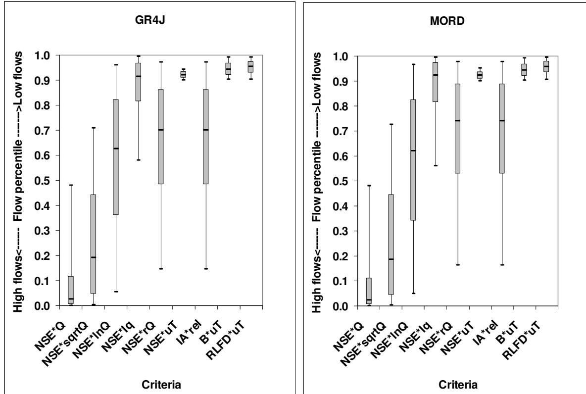
Figure 3.8: Master box plot obtained over the entire catchment set for the GR4J and MORD models (each flow percentile of exceedance corresponds to the median of this percentile over all the box plots obtained on each catchment of the entire set)
