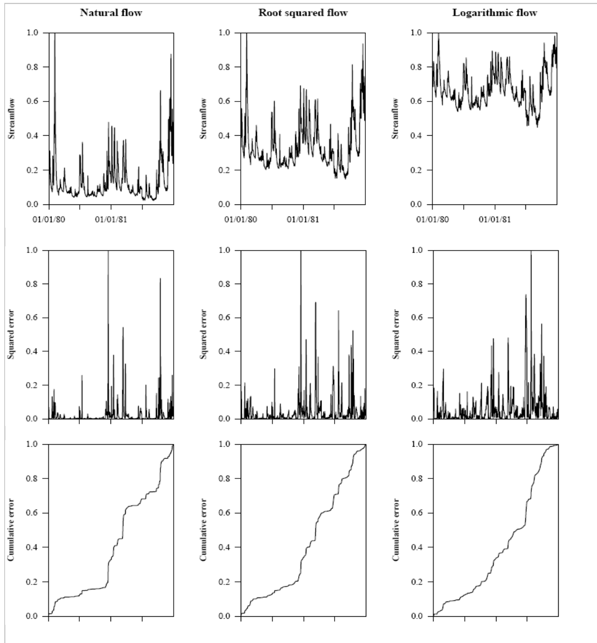
Figure 3.1: Illustration of changes in the series of flows, model errors and cumulated squared errors using root square and logarithm transformations for the Moselle River at Custines (Hydro code: A7010610; catchment area: 6830 km 2 ; period: 01/01/1980–31/12/1981).
