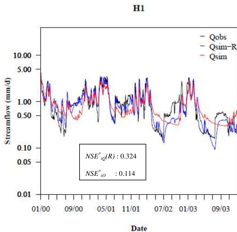
Figure 6.7: Illustration of the observed and simulated hydrographs (with and without R) of one of the test catchments for a period of four years (2000-2003) and its efficiency values
