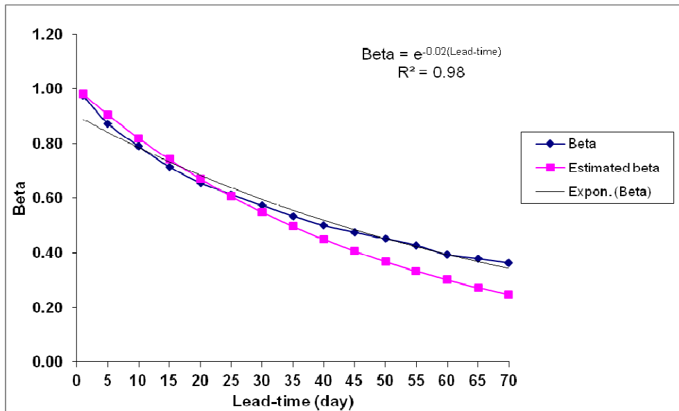
Figure 5.10: Dependency of beta value with forecast lead-time
