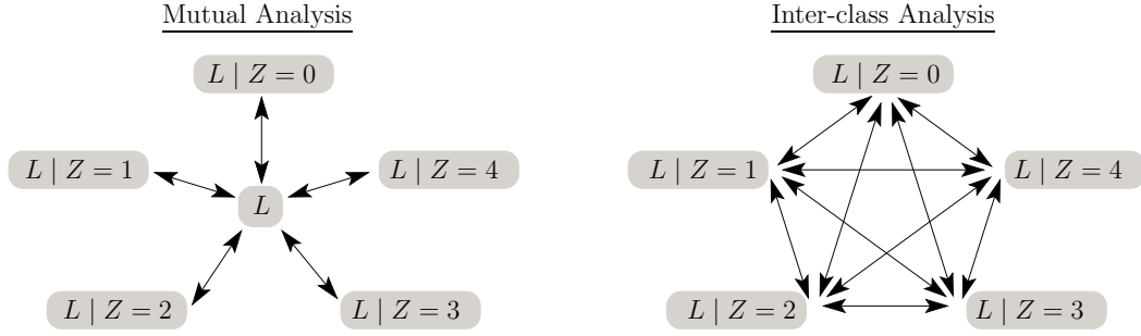
Figure 5.1: Reflecting different strategies to compare classes of conditional probability distributions (the distance between A and B is depicted with an arrow).
