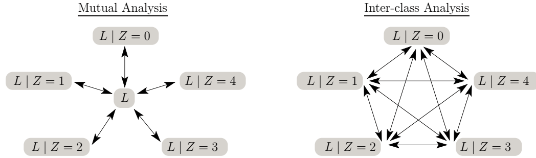
Figure 5: Le distingueur “Inter-class Information Analysis”
