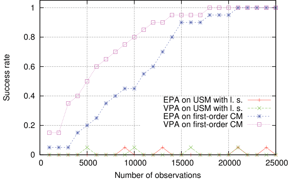
Figure 10.7: First-order success rate of 3 distinguishers.
