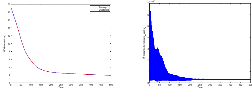
Figure 5.3: H^s norm to the ground state (left) for the averaged system (continuous line) and the oscillating system (dashed line). H^2 gap from the average (right).
