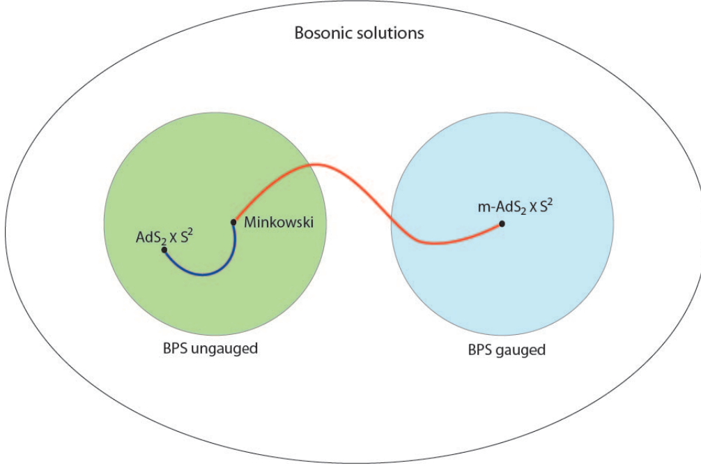
Figure 3.1: The two bubbles represent the space of BPS solutions of ungauged and abelian gauged supergravity with a flat potential, as subspaces of all bosonic solutions, common to both theories. Note the presence of two distinct \text{AdS}_2 \times S^2 backgrounds that are supersymmetric only within one theory. The blue line represents the BPS black hole solutions, interpolating between Minkowski space and the fully BPS \text{AdS}_2 \times S^2 . It is supersymmetric with respect to the ungauged theory, but not with respect to the gauged one. The solutions described here, represented by a red line, interpolate between Minkowski and the so called magnetic \text{AdS}_2 \times S^2 vacuum and they are globally non-supersymmetric.
