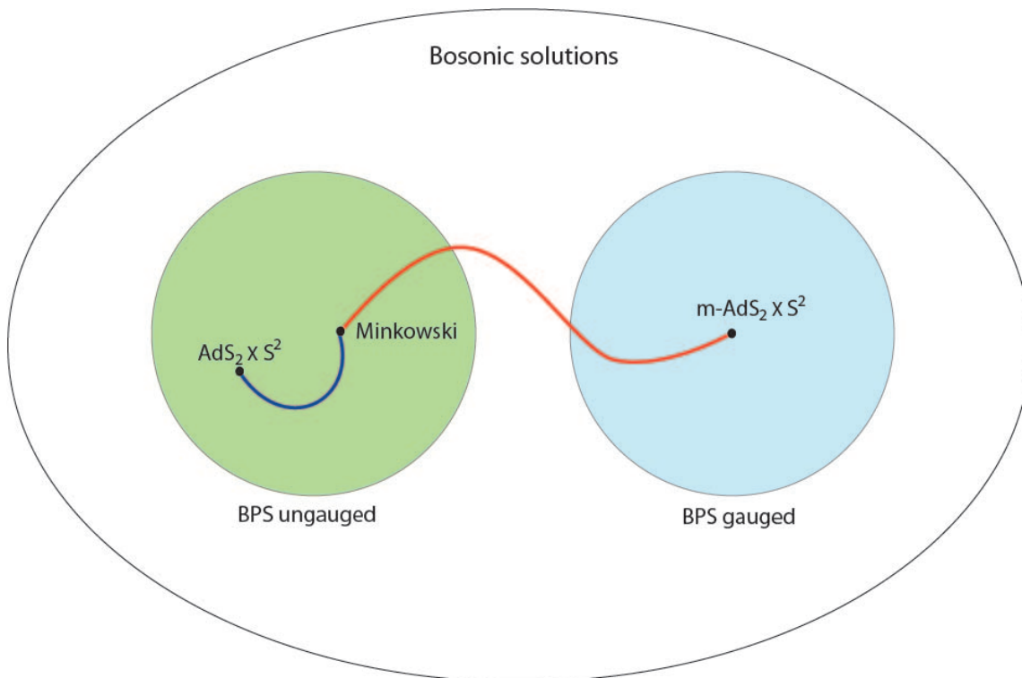
Figure 1. The two bubbles above represent the space of BPS solutions to ungauged and abelian gauged supergravity with a flat potential, as subspaces of all bosonic solutions, common to both theories. Note the presence of two distinct \text{AdS}_2 \times S^2 backgrounds that are supersymmetric only within one theory. The blue line represents the BPS black hole solutions, interpolating between Minkowski space and the fully BPS \text{AdS}_2 \times S^2 . The solutions described in this paper, represented by a red line, interpolate between Minkowski and the so called magnetic \text{AdS}_2 \times S^2 vacuum.
