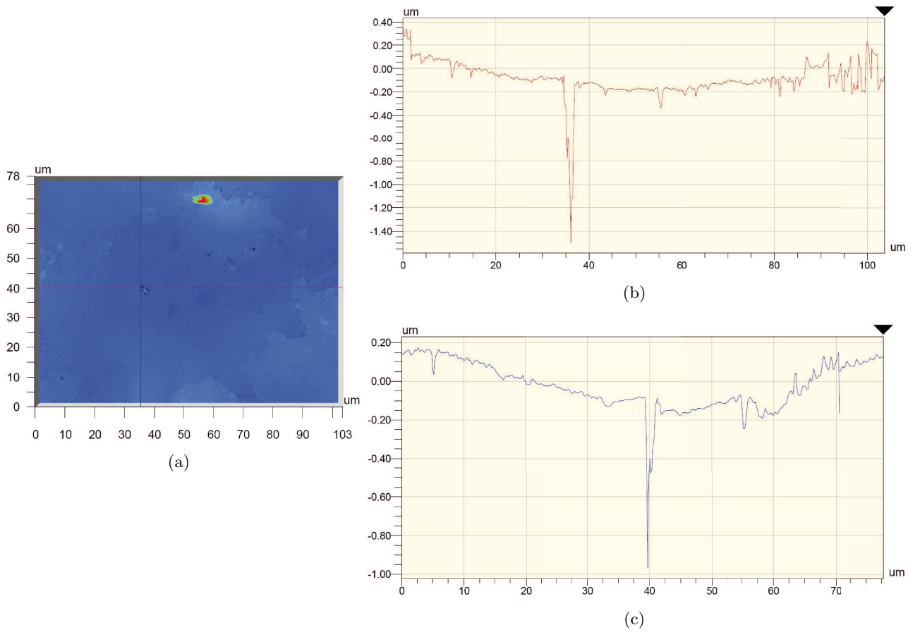
Figure 6.26: Interferometer profile measurements on a cavity, error bar: \pm 5\% . (a) location of the cavity: X-axis in red curve and Y-axis in blue; (b) X-axis profile scan: (c) Y-axis profile scan.
