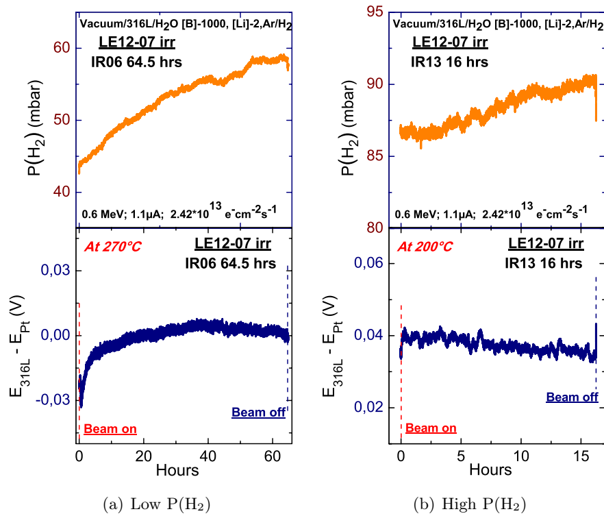
Figure 6.15: Sequential irradiations experiments of LE12-07 irr (D), ageing influence: (a) IR06: 64.5 hours under electron irradiation at 270°C; (b) IR13: 16 hours under electron irradiation at 200°C.
