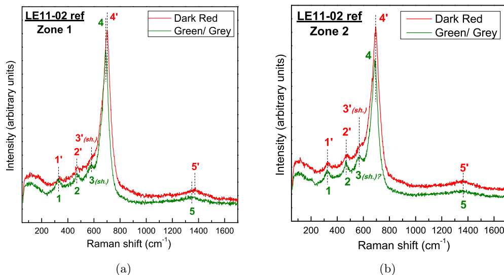
Figure 5.18: Raman spectra of LE11-02 ref (72hr, 133 m bar), zone 1 (central zone) in (a) and zone 2 (confined zone) in (b).
