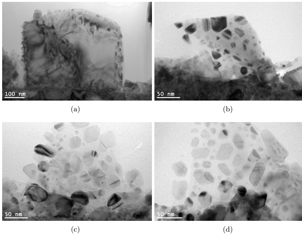
Figure 5.23: TEM micrographs on the outer layer of the oxide film formed on LE11-02 ref (72hr, 133 s mbar): (a), (b), (c) and (d), different spots of the outer layer.
