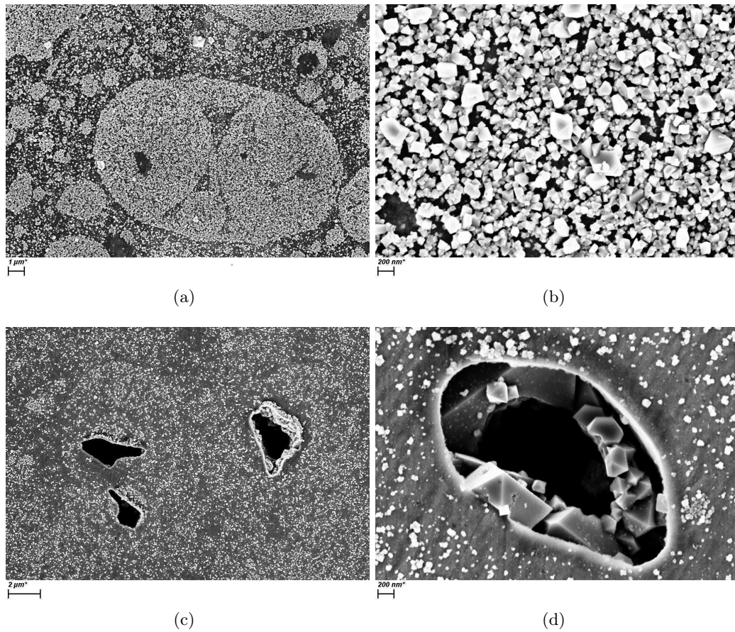
Figure 6.23: SEM micrographs for different sports of LE12-07 irr (D) in zone 1 (irradiated). SEM under the conditions: EHT = 5kV, WD = 6.0 mm.
