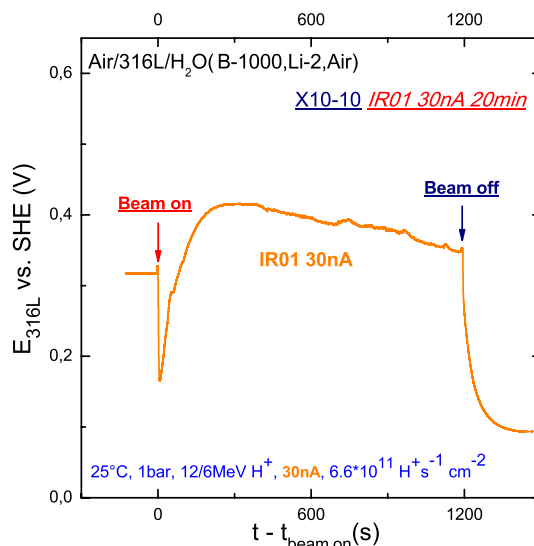
Figure 8.4: Free corrosion potential of 316L as a function of time for the sample X10-10, irradiated with a flux of 30 nA at room temperature.
