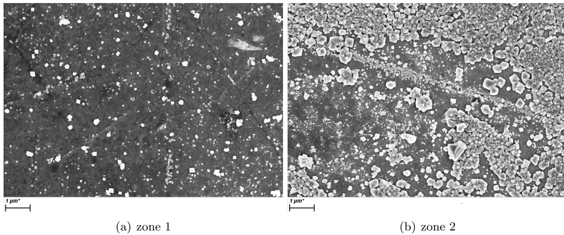
Figure 5.5: SEM micrographs of LE11 – 03 ref (168hr, 33 s mbar), SEM under the conditions: EHT = 5kV, WD = 6.2 mm, Mag = 10kX. (a) zone 1 , the 6 mm in the centre of the 316L disc; (b) zone 2 , the surrounding zone inside of seal mark.
