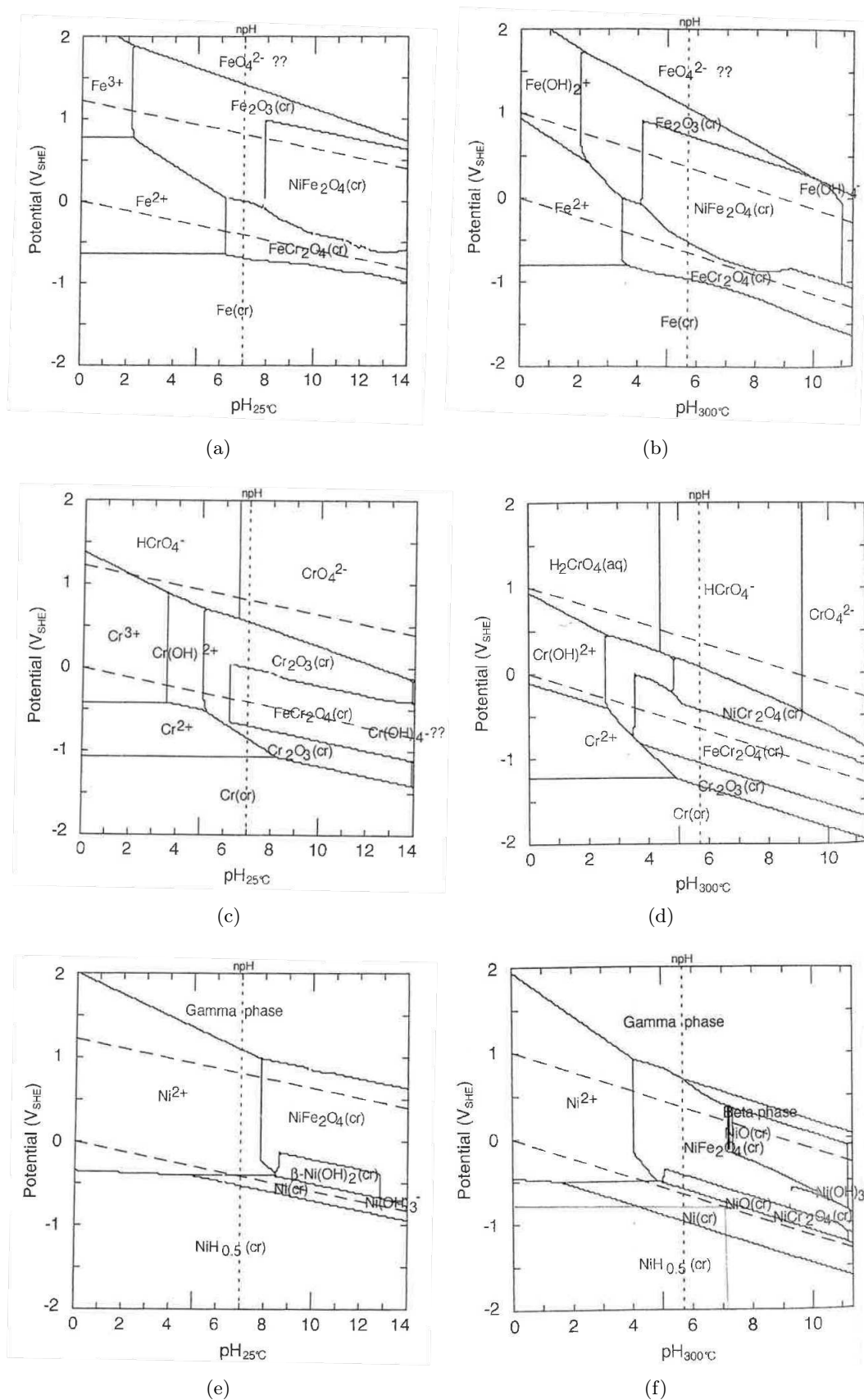
Figure 7.11: Pourbaix diagrams for the ternary system of iron-chromium-nickel at 25°C and 300°C and [\text{Fe}(\text{aq})]_{\text{tot}} = [\text{Cr}(\text{aq})]_{\text{tot}} = [\text{Ni}(\text{aq})]_{\text{tot}} = 10^{-6} molal: (a) and (b) iron species; (c) and (d) chromium species; (e) and (f) nickel species, (cr): crystallised [12].
