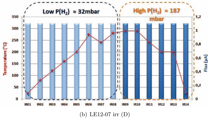
Figure 6.10: History diagrams of sequential irradiations experiments performed on LE11-04 irr (D) and LE12-07 irr (D), respectively. Red curve: temperature of the HTHP cell; Blue column: flux for each irradiation. (a): LE11-04 irr (D): [25, 300]°C, [168, 465] nA, fixed initial P(H_2) , 190 mbar; (b): LE12-07 irr (D): [25, 300]°C, 1.1 \pm 0.2 \mu A , [32, 195] mbar of P(H_2) .
