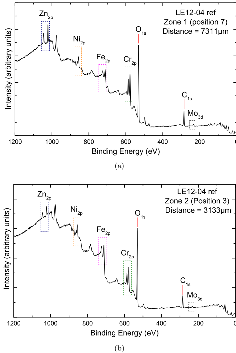
Figure 5.8: Survey spectra of 316L stainless steel discs, LE12-04 ref (120hr, 33 s mbar), 120 hours under simulate primary PWR conditions in the HTHP cell : (a) position 7 in the zone 1 (central zone); (b) position 3 in the zone 2 (confined zone).
