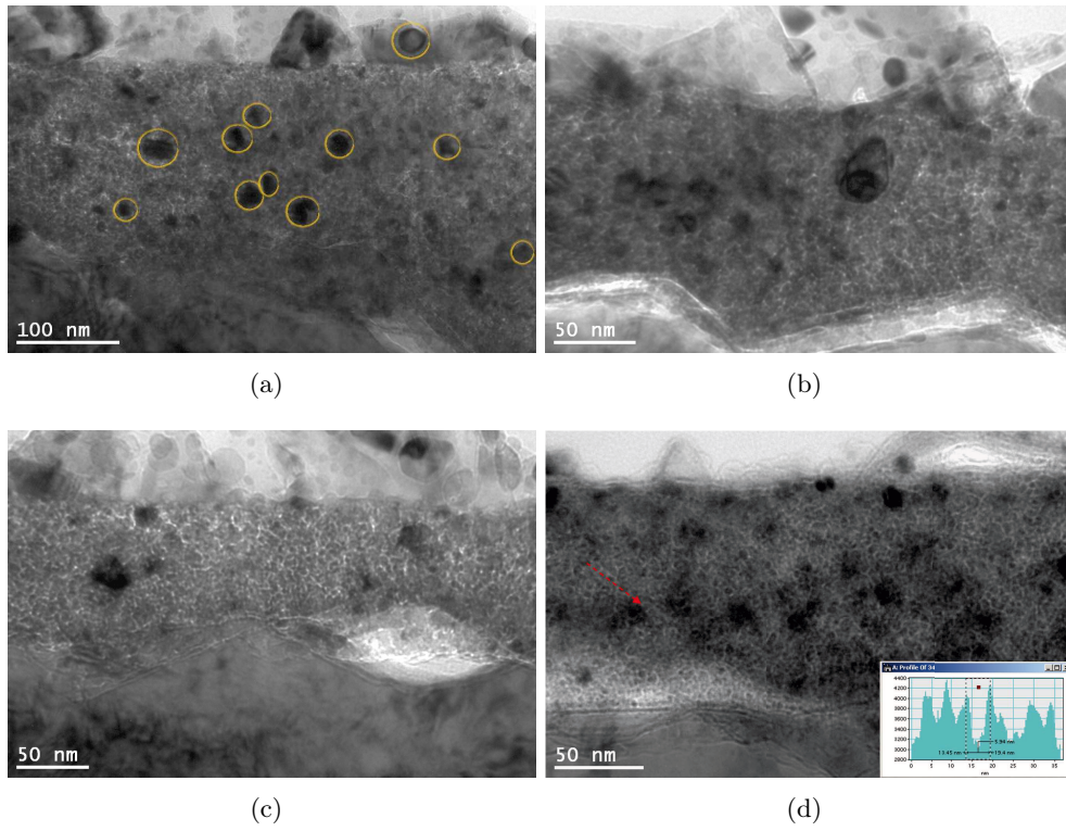
Figure 5.22: TEM micrographs on the inner layer of the oxide film formed on LE11-02 ref (72hr, 133 s mbar): (a), (b), (c) and (d), different spots of the inner layer.
