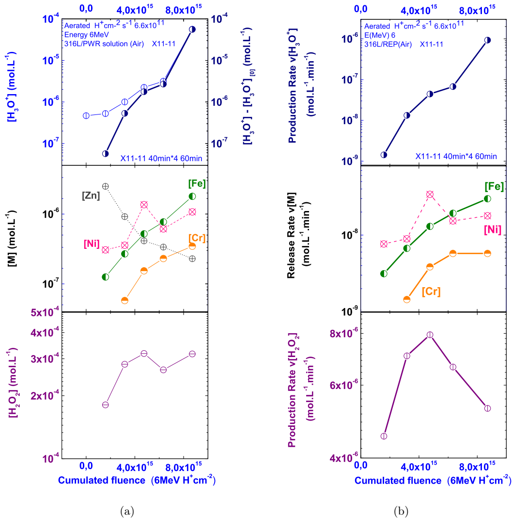
Figure 8.7: Solution analysis of different parameters versus cumulated fluence on the 316L stainless steel X11-11: (a) concentration of [H 3 O + ] (left) and [H 3 O + ] - [H 3 O + ] 0 (right) ( on the top ), cations ( in the middle ) and [H 2 O 2 ] ( at the bottom ) versus cumulated fluence on 316L stainless steel X11-11; (b) production rate of [H 3 O + ] ( on the top ), release rate of cations ( in the middle ) and production rate of [H 2 O 2 ] ( at the bottom ).
