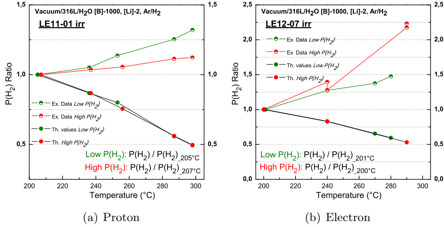
Figure C.1: Hydrogen Pressure Ratio versus temperature: (a) LE11-01 irr, proton irradiation, P(H_2)/P(H_2)_{205^{\circ}C} for low P(H_2) and P(H_2)/P(H_2)_{207^{\circ}C} for High P(H_2) ; (b) LE12-07 irr, electron irradiation, P(H_2)/P(H_2)_{201^{\circ}C} for low P(H_2) and P(H_2)/P(H_2)_{200^{\circ}C} for High P(H_2) .
