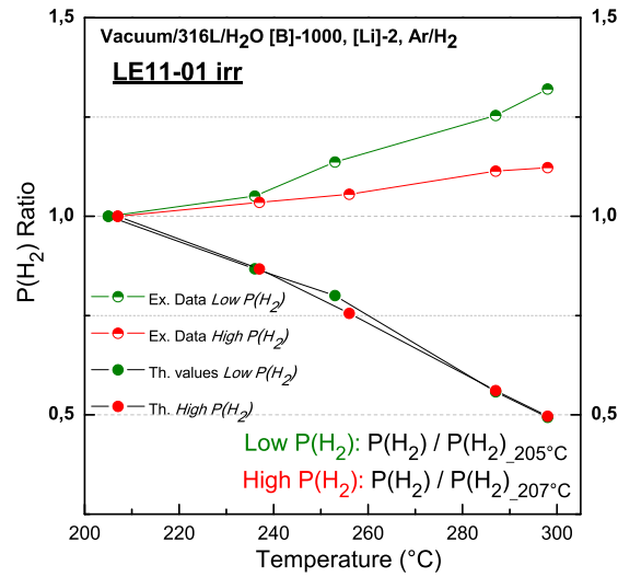
Figure 6.7: Hydrogen Pressure Ratio versus temperature, P(H_2)/P(H_2)_{205^\circ C} for low P(H_2) and P(H_2)/P(H_2)_{207^\circ C} for High P(H_2) . Ex. data are calculated on the basis of Fig.6.6 (b), and Th. data are calculated in Appendix C.
