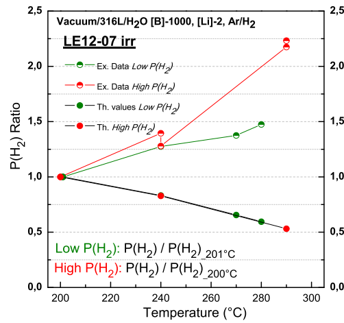
Figure 6.14: Hydrogen Pressure Ratio versus temperature, P(H_2)/P(H_2)_{201^\circ C} for low P(H_2) and P(H_2)/P(H_2)_{200^\circ C} for High P(H_2) . Ex. data are calculated on the basis of Fig.6.6 (b), and Th. data are calculated in Appendix C.
