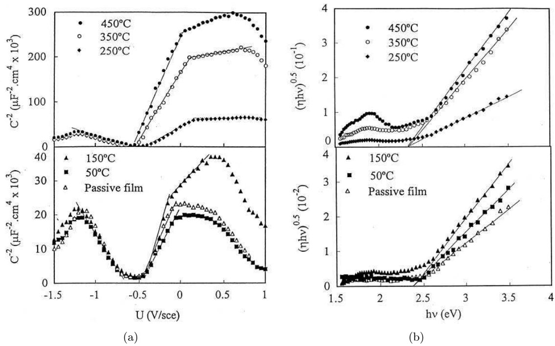
Figure 3.19: The effect of temperature on electrochemical behaviour of oxide formed 304 stainless steel in the temperature range from 50 to 450°C, with the presence of passive film formed at 0.8 V/SCE in borate buffer solution : (a) plot of 1/C^2 as a function of applied potential U ; (b) plot of (\eta h\nu)^{0.5} versus the incident light energy h\nu [31].
