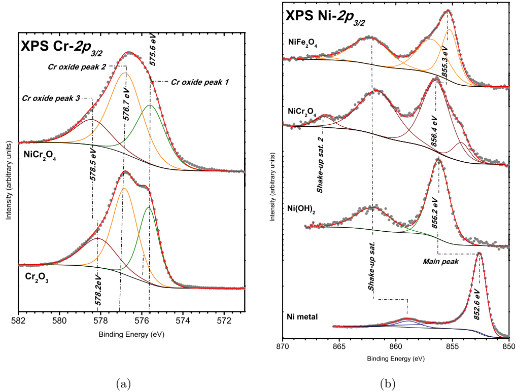
Figure 5.10: Reference spectra of Cr 2p 3/2 and Ni 2p 3/2 : (a) Cr 2p 3/2 , including NiCr 2 O 4 (top) and Cr 2 O 3 (bottom); (b) Ni 2p 3/2 , including NiFe 2 O 4 , NiCr 2 O 4 , Ni(OH) 2 and metallic Ni, in order from top to bottom [9].
