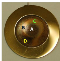
Figure 6.16: Photo of LE11-04 irr (D), showing the different spots for the SEM analysis. (A): zone 1, irradiated zone, (B) and (C) mixed zone, between zone 1 and 2, (D) zone 2, unirradiated zone.
