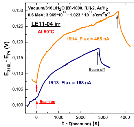
Figure 6.11: Sequential irradiations experiments of LE11-04 irr (D): IR13 (168 nA) and IR14 (465 nA) at the same temperature 50°C with the same initial hydrogen pressure.
