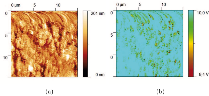
Figure 6.39: Cartography images of LE12-07 irr (D), zone 1 (irradiated), analysed area: 15 \times 15 \mu\text{m}^2 . (a) topography images and (b) current image.
