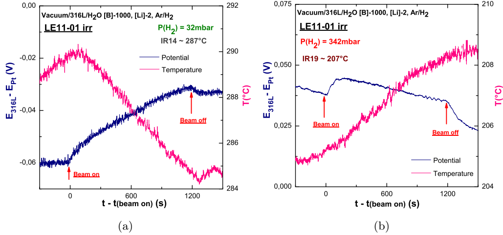
Figure 6.5: 1 st sequential irradiations experiments of LE11-01 irr (D), potential between 316L and Pt ( on the left ) and temperature ( on the right ) in function of time. (a): I14 at 287°C and P(H_2) 32 mbar; (b): I19 at 207°C and P(H_2) 342 mbar.
