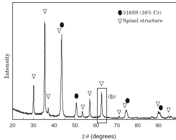
Figure 3.2: XRD analysis of 316L formed under PWR simulated conditions, 320°C, 380 hours [10].
