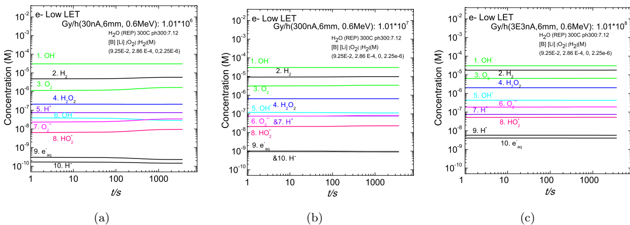
Figure 7.14: Modelling of radiolysis species produced at 300°C, PWR water (1000 ppm [B] and 2ppm [Li]) aerated by Ar/H 2 5%, by using homogeneous calculation of chemical kinetics, Data Set ( g_{300^\circ C} , k_{300^\circ C} ) [27] for an electron beam of: (a) 30 nA; (b) 300 nA; (c) 3000 nA.
