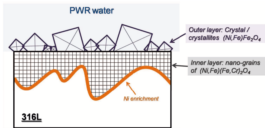
Figure 7.1: Schematic sketch for the reference oxide film formed on 316L stainless steel exposed to primary PWR water at 300°C in the HTHP cell for a duration around 70 - 170 hours.
