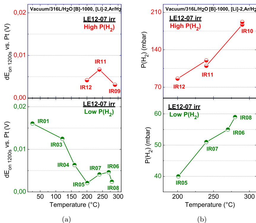
Figure 6.13: Sequential irradiations experiments of LE12-07 irr (D): (a) \Delta E_{1200s} versus temperature, irradiations under low hydrogen pressure on the bottom and the ones at high hydrogen pressure on the top ; (b) hydrogen pressure of each irradiation versus temperature, low hydrogen part on the bottom and high hydrogen part on the top .
