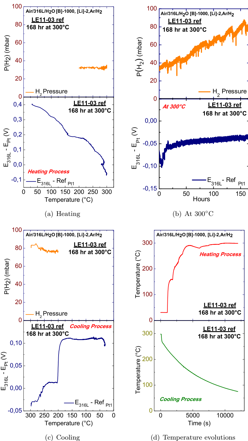
Figure 5.1: Electrochemistry and hydrogen measurements of LE11-03 ref (168hr, 33,mbar), hydrogen pressure ( on the top ) and free potential between 316L and platinum ( at the bottom ) versus temperature: (a) heating process; (c) cooling process. (b): Electrochemistry ( at the bottom ) and hydrogen evolution ( on the top ) at 300°C for 168 hours. (d): Heating ( on the top ) and cooling ( at the bottom ).
