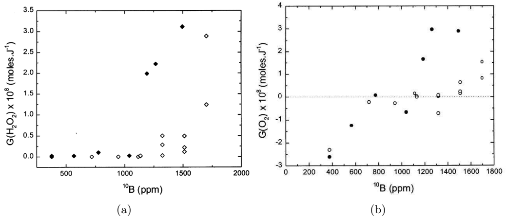
Figure 2.18: The effect of Fe(NO_3)_3 at 30°C on water radiolysis: (a) G(H_2O_2) vs. [^{10}B] ; (b) G(O_2) vs. [^{10}B] . Solid points: \bullet and \blacklozenge for 2ppm Fe(NO_3)_3 ; open points: \circ and \diamond for blank solution [87].
