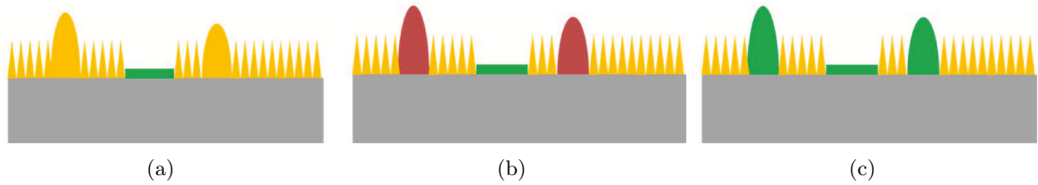
Figure 6.42: Schematic layout of the oxide film formed on LE12-07 irr (D), observed by CS-AFM, (a) general case; (b) conductive case and (c) resistive case. Small and big yellow triangle: small and big general crystallites; big red triangle: conductive crystallites; big green triangle: resistive crystallites; green substrate: smooth and insulated area.
