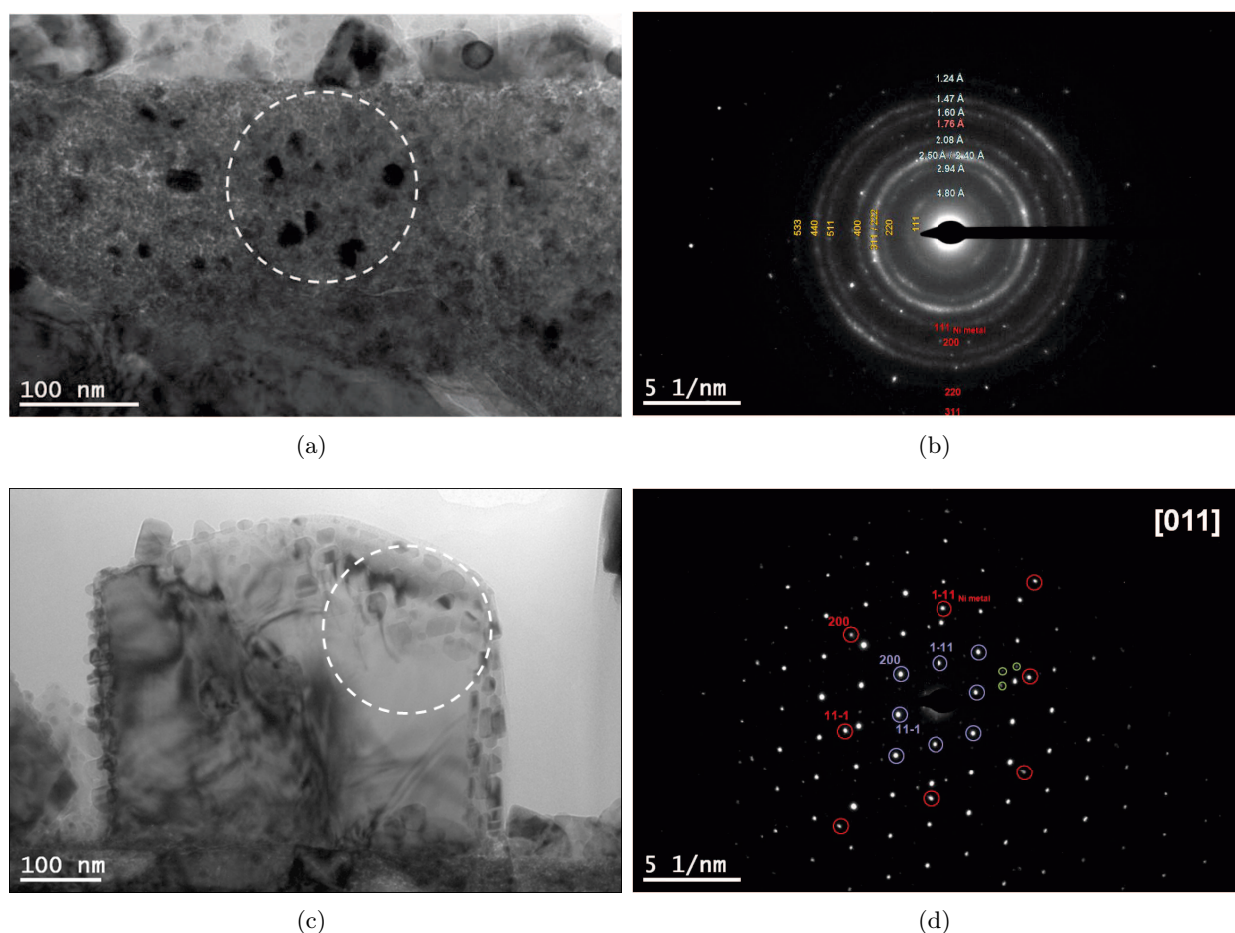
Figure 5.26: TEM-SAD analysis on LE11-02 ref (72hr, 133, mbar): (b) & (d) are the electron diffraction patterns of the selected area on images (a) & (c), respectively. Indicators: blue and yellow for the spinel oxides; red for the metallic Ni and green for the double diffraction.
