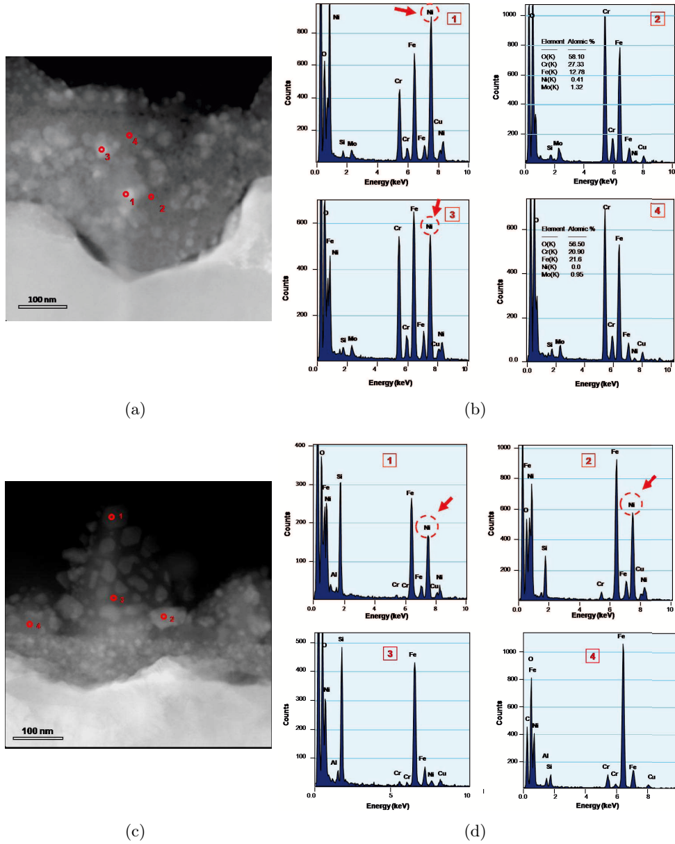
Figure 5.24: TEM-EDX Analysis on LE11-02 ref (72hr, 133 s mbar), (a) & (b) for the inner layer, (c) & (d) for the outer layer. (a): STEM-HADDF image of the inner layer; (b): EDX spectra of different spots indicated in (a); (c): STEM-HADDF image of the outer layer; (d): EDX spectra of different spots indicated in (c).
