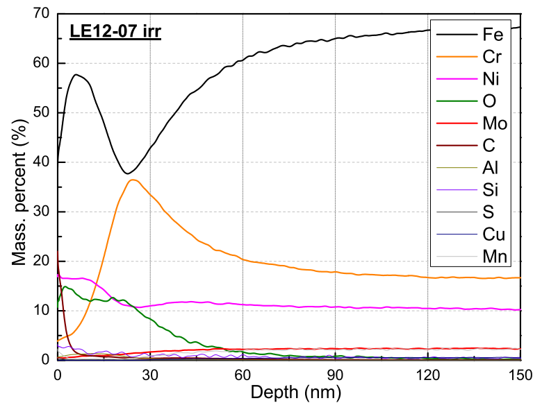
Figure 6.38: GD-OES elemental scan in depth profile on LE12-07 irr (D) (zone 1, irradiated), error bar: \pm 5\% .
