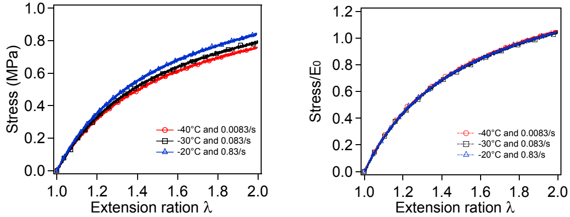
Figure G.1. (a) Nominal stress vs. extension ratio of PB50/SBR50 blend at different temperature and strain rate: T=-40^{\circ}\text{C} and \dot{\epsilon}_1 = 0.0083/\text{s} ( \circ ); T=-30^{\circ}\text{C} and \dot{\epsilon}_2 = 0.083/\text{s} ( \square ); T=-20^{\circ}\text{C} and \dot{\epsilon}_3 = 0.83/\text{s} ( \Delta ). (b) Nominal stress normalized by initial modulus vs. extension ratio with same conditions.
