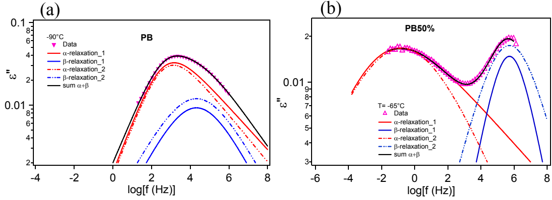
Figure 3.24. Separation of \alpha -relaxation and \beta -relaxation by two individual Havriliak-Negami functions; (a) PB sample at -90^\circ\text{C} , (b) PB50% samples at -65^\circ\text{C} . Solid lines are fits with lower \beta -relaxation amplitude value (hypothesis 1) and dotted lines are fits with higher \beta -relaxation amplitude value (hypothesis 2).
