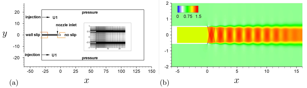
FIGURE 6.11: (a): Sketch of the jet configuration with boundary conditions. In the inward is depicted the discretization near the nozzle exit (one discrete point out of two). (b): Mach number contours of the baseflow \mathbf{w}_b near the nozzle exit.
