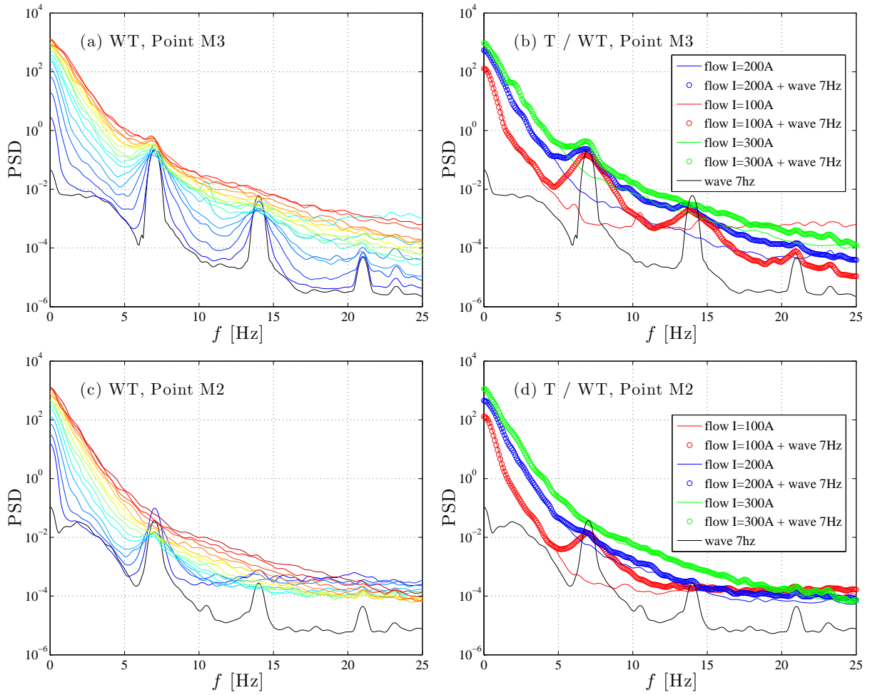
Figure 6.5: Power spectral densities (PSD). Top panels corresponds to M3, and bottom panels to M2. Figures on the left were obtained with turbulence and waves for all the explored forcing intensities. Those on the right are few examples when wave + turbulence (WT) is compared with the case with only turbulence (T).
