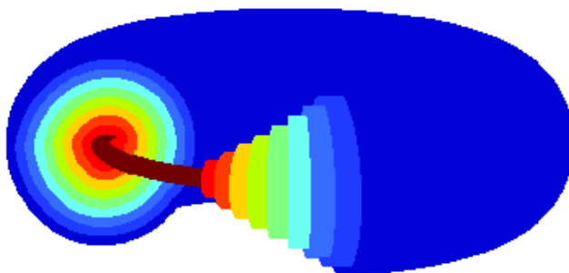
Figure 2.1: Nested tori representing the magnetic surfaces.
