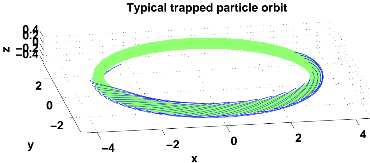
Figure 2.7: Typical orbit of a trapped particle in a tokamak. A slow toroidal precession (from the right to the left) is observed on top of the bounce motion. The fast cyclotron motion is averaged out.
