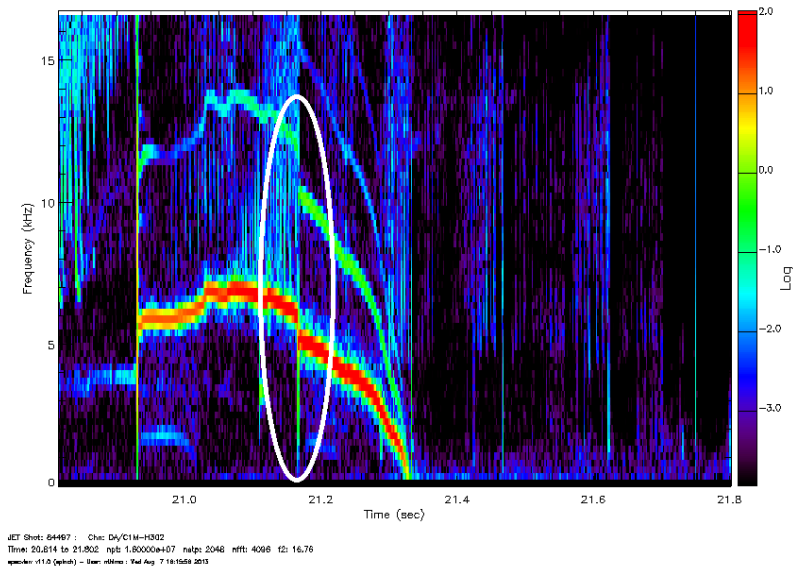
Figure 5.19: Spectrogram of the magnetic coil signal after the triggering of the NTM. Mode locking can be seen to occur at t = 21.33 .
