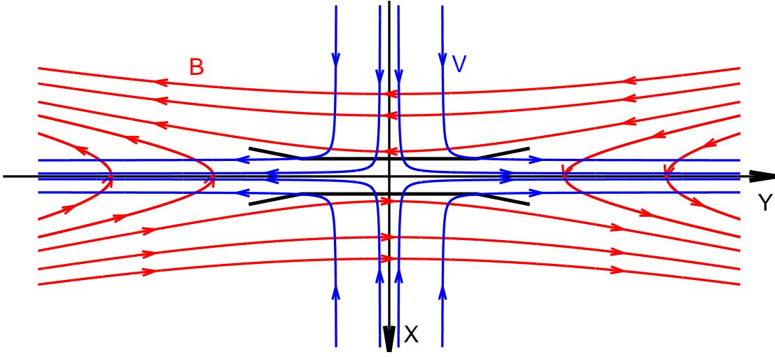
Figure 2.11: Structure of a Sweet-Parker current sheet. Streamlines (blue) and magnetic field lines (red). Away from the current sheet in the center, ideal MHD is valid and the flow carries the field lines with itself.
