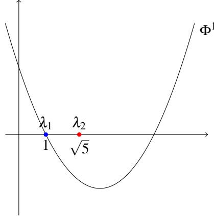
Figure 7.1: A scalar Riccati dynamic function. The stable equilibrium point is in blue ( \lambda_1 ). The right end point of the contraction interval is in red ( \lambda_2 ).
