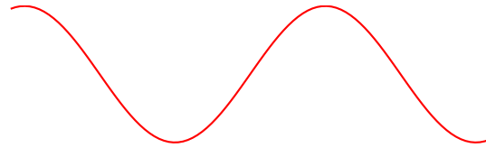
(a) semiconvex function \psi(x) = \sin x
