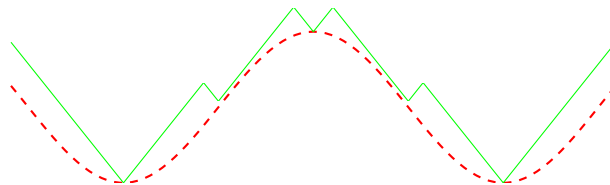
(b) projection P_{\mathcal{L}}(\psi) = |x| + 1 \wedge |x - \frac{\pi}{2}| \wedge |x + \frac{\pi}{2}| \wedge |x + \pi| + 1 \wedge |x - \pi| - 1
