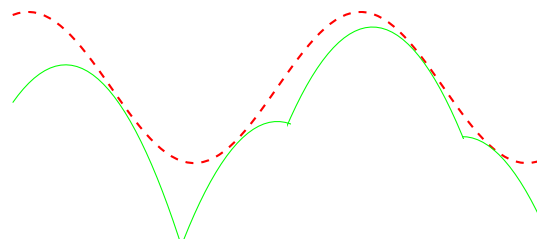
(b) projection P_{\mathcal{M}}(\psi) = -\frac{x^2}{2} + 1.55 \vee -\frac{(x-1.8)^2}{2} + 2.8 \vee -\frac{(x+4)^2}{2} + 2.3 \vee -\frac{(x-3.5)^2}{2} + 1.35
