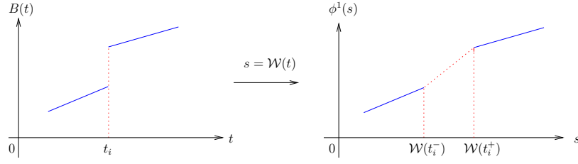
FIGURE 3.1: Reparametrization
