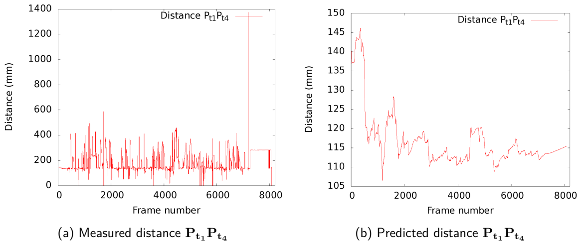
Figure 5.12: Distance \mathbf{P}_{t_1}\mathbf{P}_{t_4}
