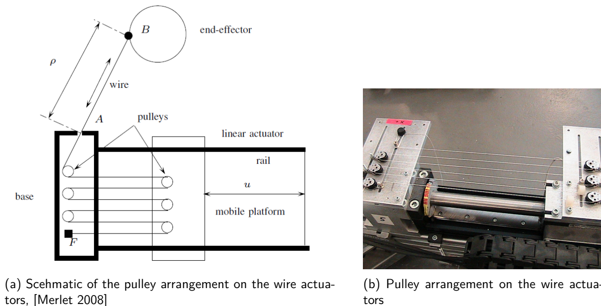
Figure 3.2: The pulley arrangement on the actuated cable-based parallel robot
