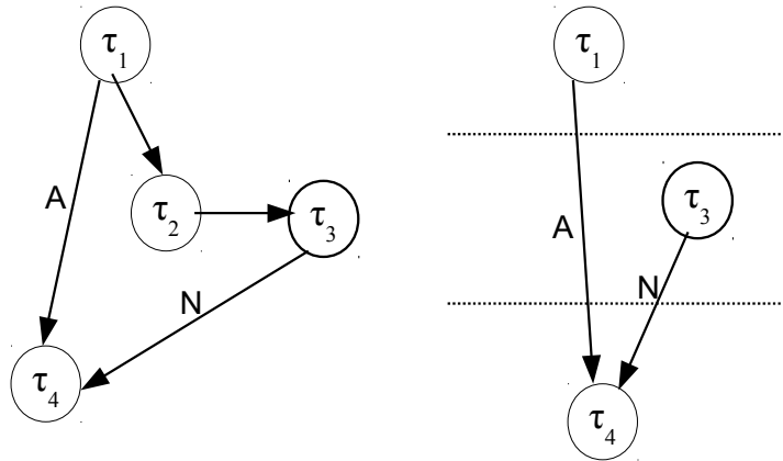
Figure 7.12: A part of an SDG and the topological sort order of predecessors of \tau_4
