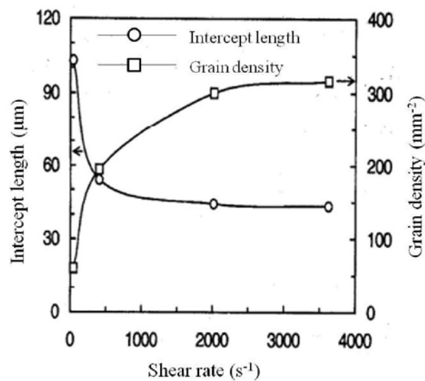
Fig. 1.26. Effect of shear rate on the grain size and density of Sn-15% Pb alloy cooled from 215^{\circ}\text{C} to 205^{\circ}\text{C} with a cooling rate of 0.5^{\circ}\text{C}/\text{min} [88].
