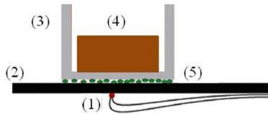
Fig. 2.28. Schematic drawing of the sample crucible. [1] Pt/Pt-10%Rh thermocouple. [2] Platinum sample holder. [3] Crucible. [4] Sample. [5] Al 2 O 3 powder to prevent welding of the platinum parts.
