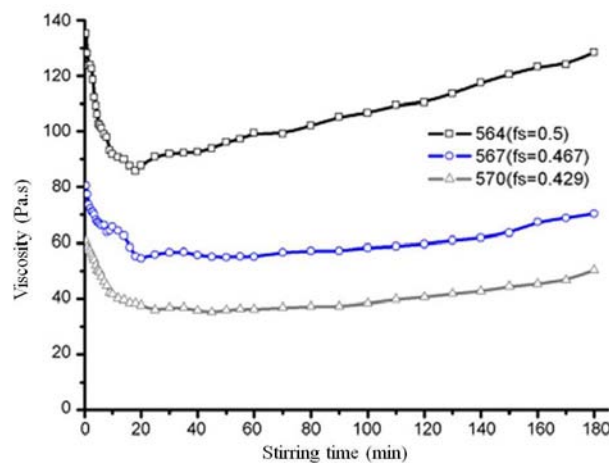
Fig. 1.33. Influence of stirring time on the apparent viscosity performed on AZ91D alloy [56].
