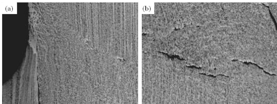
Fig. 4.32. Macrographs of the semi-solid zone in the part formed at temperature 1450°C.
