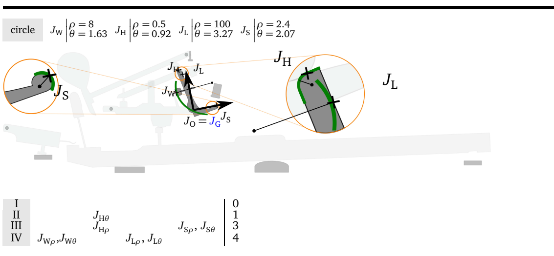
Figure 4.14 – Contacts description, jack (lengths in (mm), angles in (rad)).
