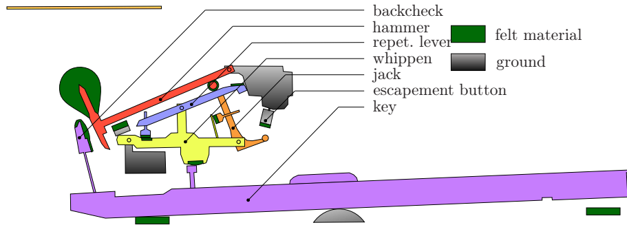
Figure 2.3 – Grand piano action (without damper).
