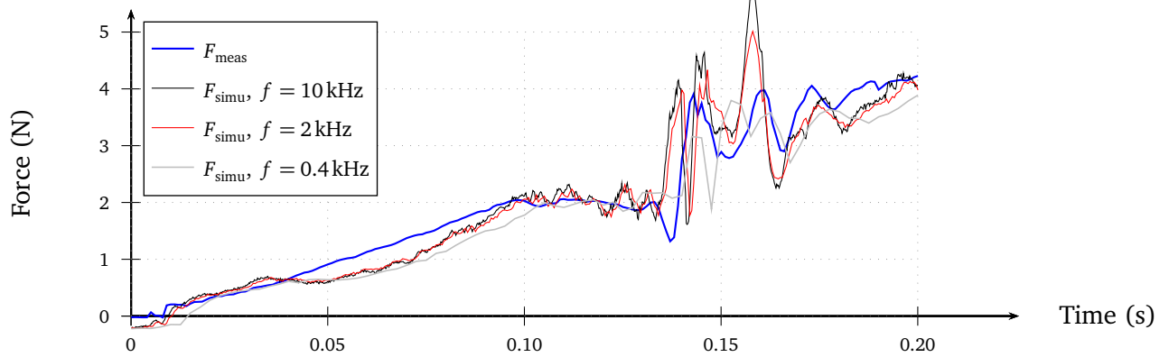
Figure 6.10 – Computed force F_{simu} for different time steps.
