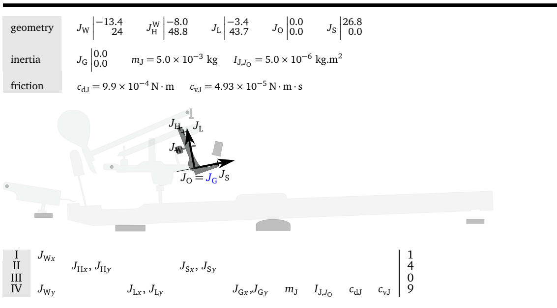
Figure 4.13 – Jack frame, measurements (lengths in (mm)).
