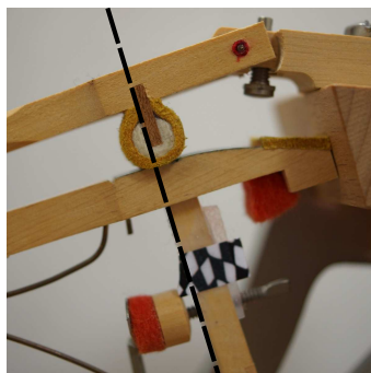
Figure A.3 – Appropriate adjustment of the jack regulating screw.
