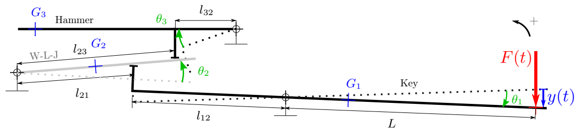
Figure 2.4 – Simplified scheme of the grand piano action in three blocks: Key, Whippen-Jack-Lever, Hammer. The damper has been excluded. The position \theta_i of each block is defined as positive when the key is pushed downwards, from 0 at rest. With an counterclockwise convention for angles (and torques), \theta_1 and \theta_3 are negative when they leave their rest position. For the sake of clarity, the reaction forces R_{ij} at the contact points between solids are not represented.
