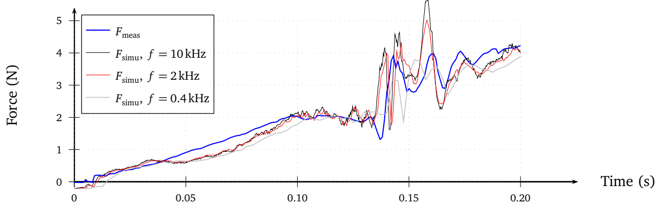
Figure 6.10 – Computed force F_{\text{simu}} for different time steps.
