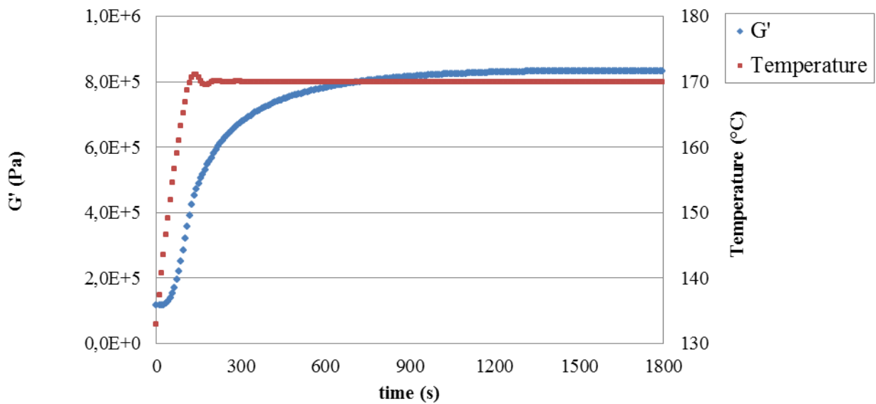
Figure 3-28: Evolution of storage modulus during crosslinking of Nordel 4520 at 170°C
