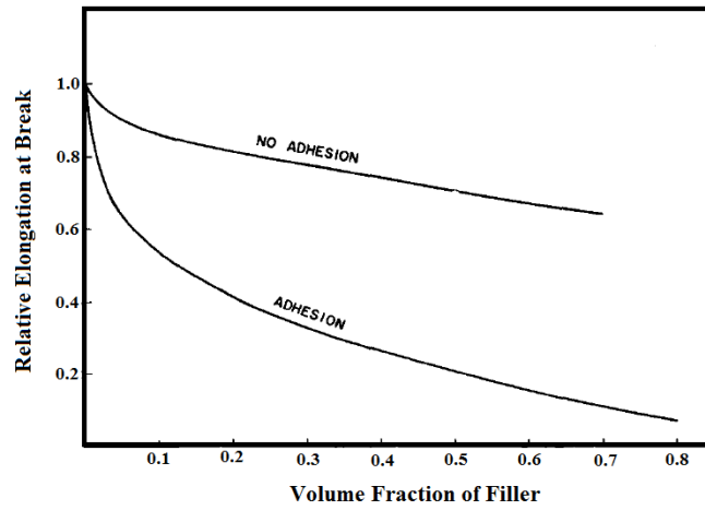
Figure 1-9: Effect of filler fraction on elongation at break [62]
