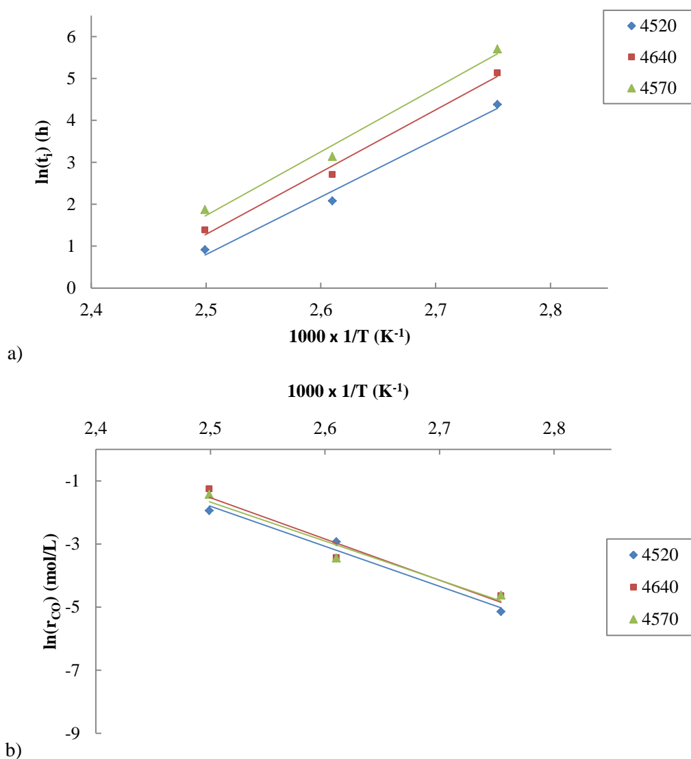
Figure 4-17: Arrhenius graph of of carbonyls' a) t_{CO} and b) r_{CO} in air between 90 and 130°C for the three EPDMs under study
