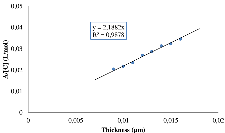
Figure 3-3: Determination of the molar extinction coefficient of methylene groups of polypropylene according to the Beer-Lambert law
