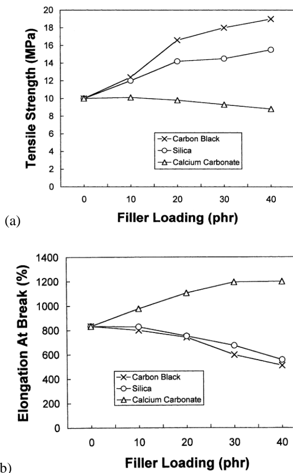
Figure 1-10: Effect of several filler fraction on a) tensile strength and b) elongation at break of EPDM composite [65]
