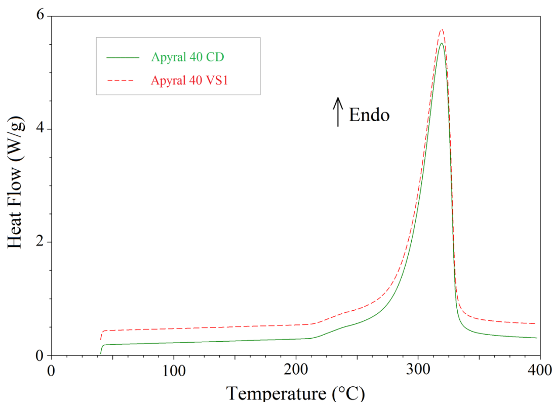
Figure 3-8 : DSC thermograms of PATH (40 CD) and TATH (40 VS1) ( 10^{\circ}C.min^{-1} , in N_2 )
