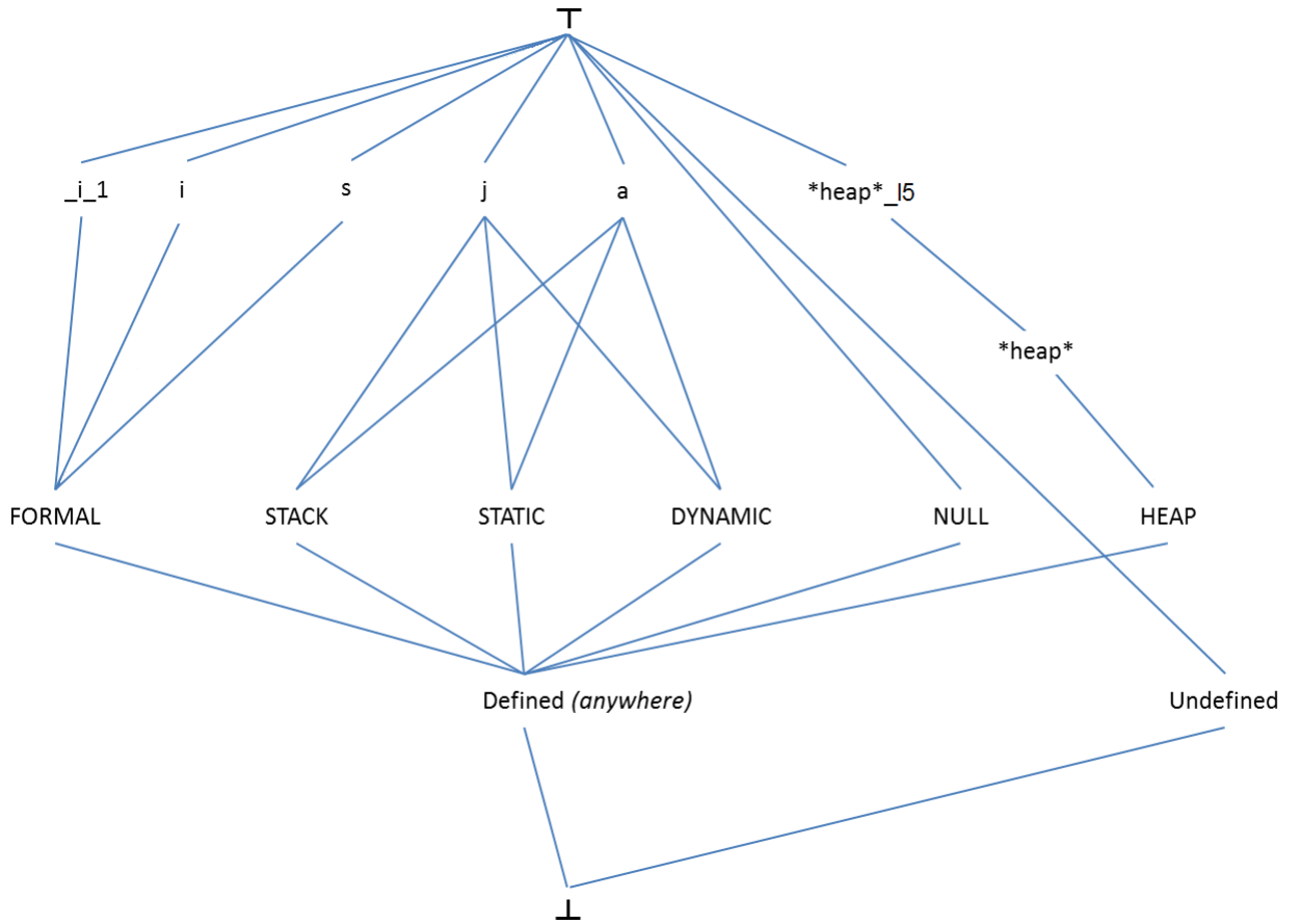
FIGURE 5.9 – Le treillis Name
