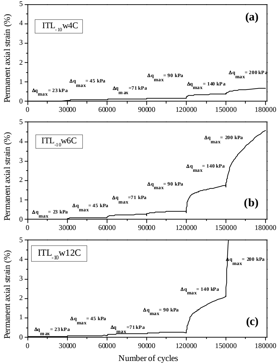
Fig.10: Permanent axial strain versus number of cycles for ITL -10 – (a) 4% water content; (b) 6% water content; (c) 12% water content
