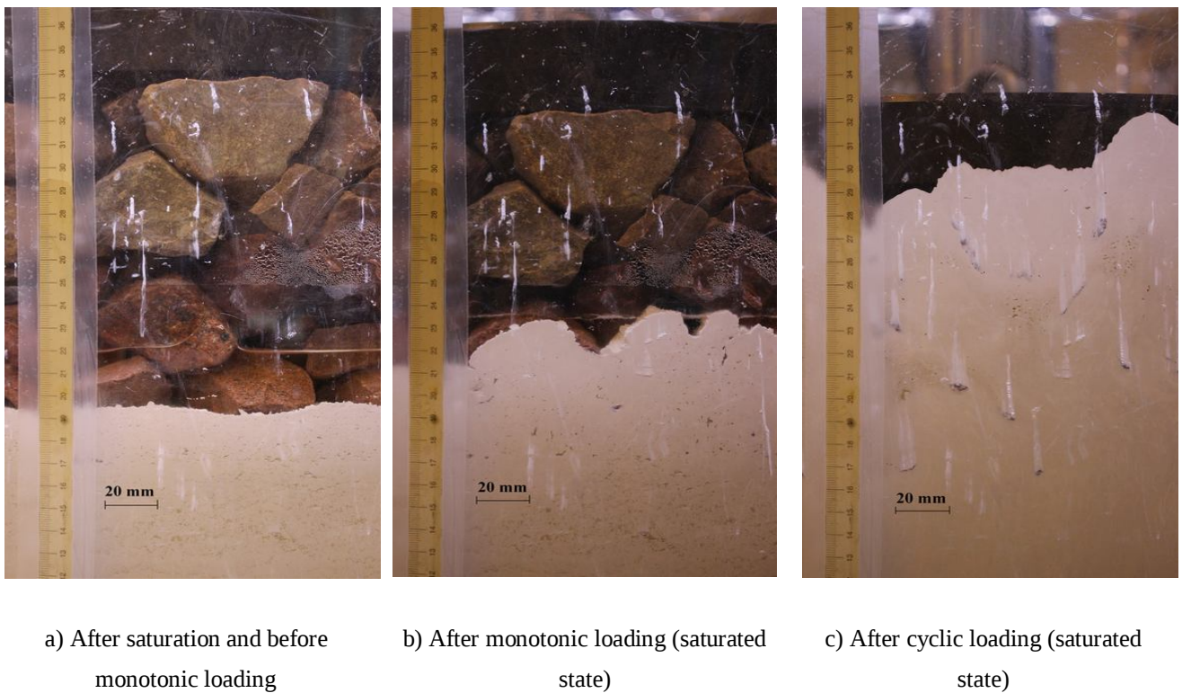
Fig.17: Photographs showing the evolution of the ballast/sub-soil interface: ( \rho_{d-initial} = 1.5 \text{ Mg/m}^3 ).
