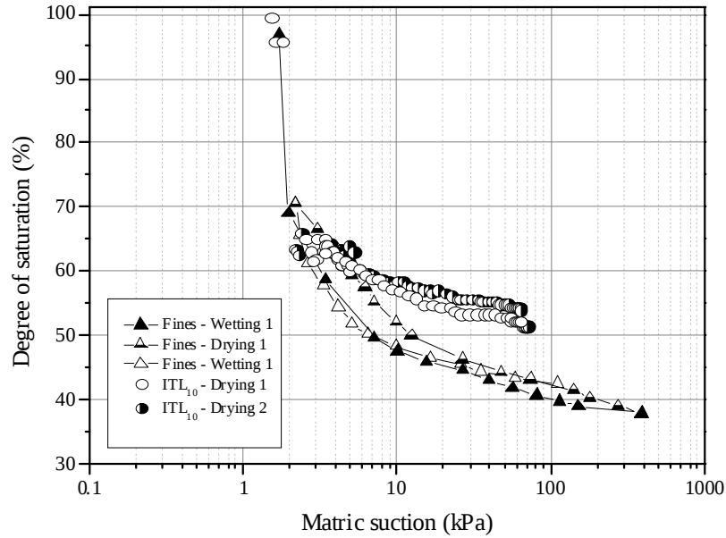
Fig. 22: Comparison of SWRC between ITL_{10} and Fines
