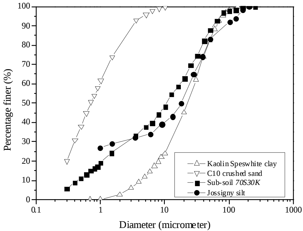
Fig. 1: Grain size distribution curve of the studied materials
