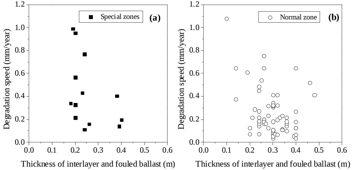
Fig. 16: Correlation of the degradation rate to the thickness of interlayer and fouled ballast for Track 1- Data from coring train. a) special zones and b) normal zone
