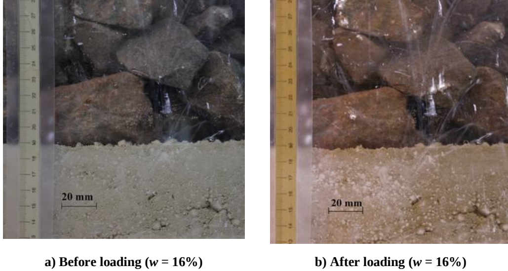
Fig. 18: Camera view of the interface between two soils: a) before and b) after loading ( w = 16\% and \rho_{d-initial} = 1.4 \text{ Mg/m}^3 ).
