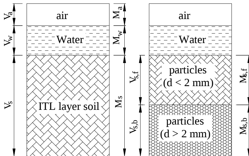
Fig. 5: Components of the unsaturated interlayer soil
