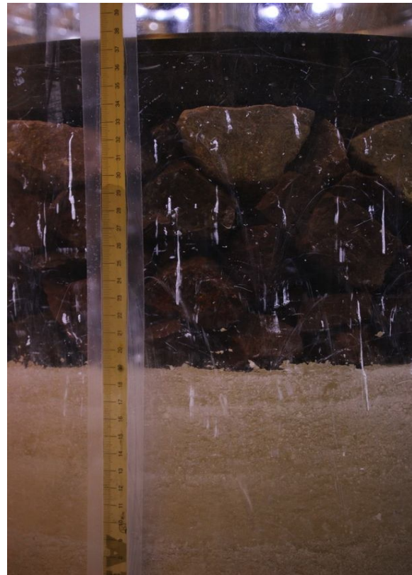
b) After loading ( w = 16\% )
