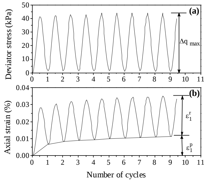
Fig. 8: First cycles of cyclic triaxial test on ITL_0 at w = 4\% (test ITL_0w4C ) - (a) Deviator stress; (b) Axial strain
